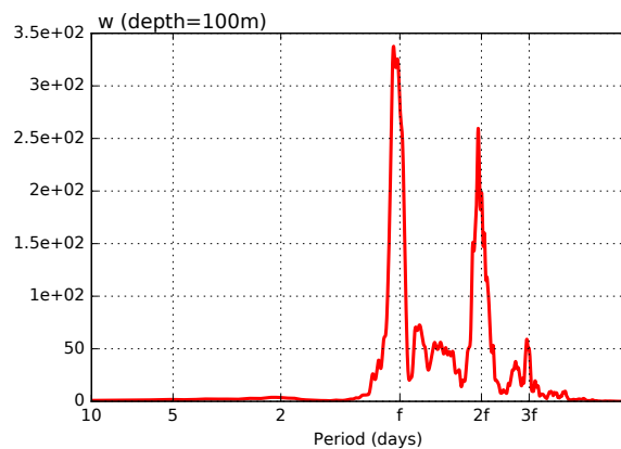
Figure 4.9: Power spectrum for w at a 100m for a point ( y= 2400\text{km} , x=1600\text{km} ) in the domain from the same configuration however run at dx=2\text{km} with hourly outputs, f is the inertial period.
