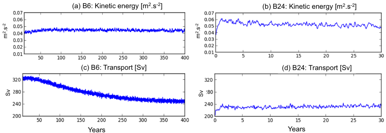
Figure 2.17: Numerical adjustments of kinetic energy [ \text{m}^2 \cdot \text{s}^{-2} ] and transport [Sv] for the B6 and B24 runs.
