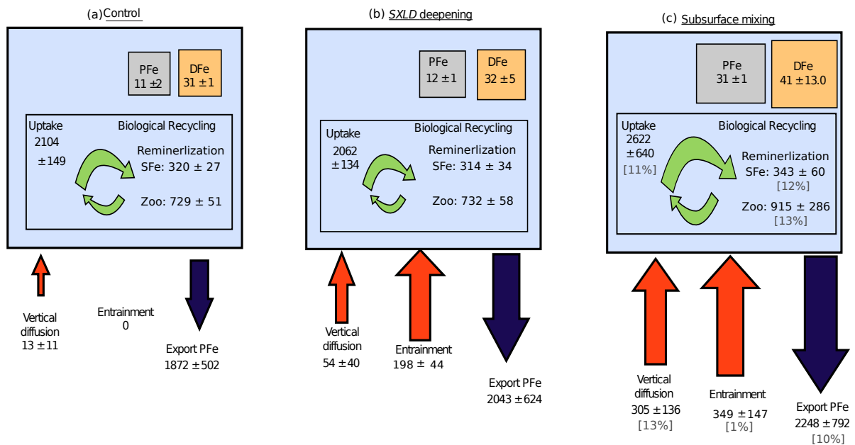
Figure 3.3: A summary of the total summer standing stocks [ \mu molm -2 ] and fluxes [nmol.DFe.m -2 .d -1 ] of iron for the upper MLD min between all model ensembles: (a) Control , (b) SXLD deepening and (c) subsurface mixing runs following the approach of Bowie et al. [2015]. Entrainment includes DFe only. Vertical diffusion of DFe is computed across the MLD interface. Export of PFe is computed at 250m below the XLD. Remineralisation includes disaggregation of small particulate iron (SFe) and zooplankton excretion and sloppy feeding (Zoo). Where indicated, the percentage that each summer value represents over the total annual mean is provided (gray text).
