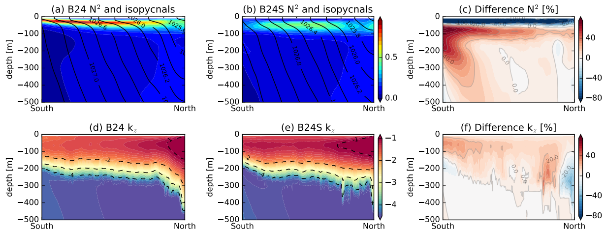
Figure 5.8: Five year annual mean stratification N^2 [ 1e4 \text{ s}^{-2} ] overlaid with isopycnals [ psu ] for (a) B24, (b) B24S and the (c) percentage mean difference (B24S - B24) / B24S \times 100 . (d-f) is the same but for vertical mixing \log_{10}[\text{m}^2 \cdot \text{s}^{-1}]
