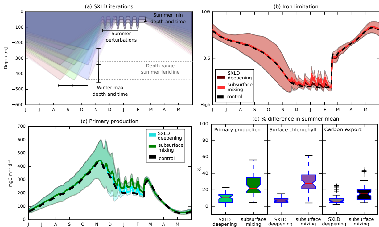
Figure 3.2: (a) Seasonal iterations of SXLD [m], (b) simulated iron limitations on phytoplankton, (c) integrated PP [ \text{mg C m}^{-2} \text{d}^{-1} ] and (d) the percentage mean change in summer PP, surface chlorophyll and carbon exported at 250m (i.e., [subsurface mixing runs - control runs]/control runs). Shading = standard deviation, solid line = mean of all iterations. The seasonal control run (no SXLD perturbations) is shown by the black-dashed curve.
