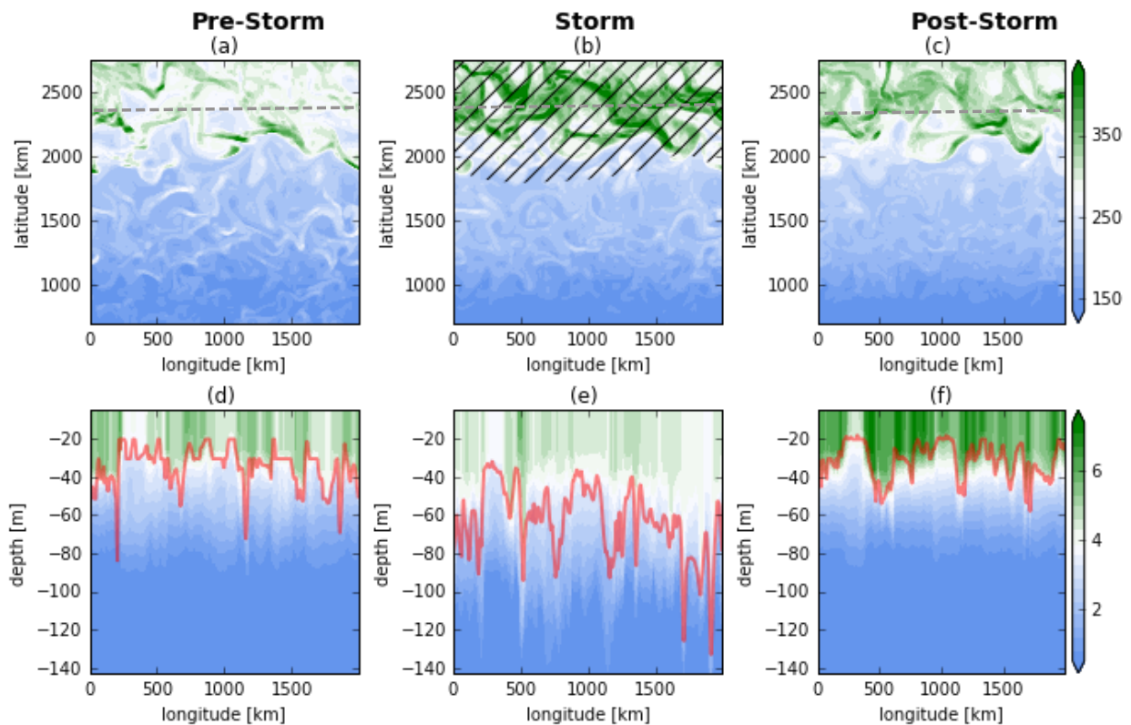
Figure 4.3: Horizontal 2-day mean snapshots of (a,b,c) integrated PP ( \text{mg C m}^{-2} \text{d}^{-1} ) and (d,e,f) meridional depth sections (at y=2400\text{km} as shown by grey dashed line on a,b,c) of PP ( \text{mg C m}^{-3} \text{d}^{-1} ). The snapshots are from (a,d) before the storm 14th of November, (b,e) during the passage of a storm on 16-18th November and (c,f) "post storm" 4 days after the storm on the 22nd November. The black hatched lines in (b) mark the area impacted by the storm, while the MLD is marked by a red line in (d,e,f).
