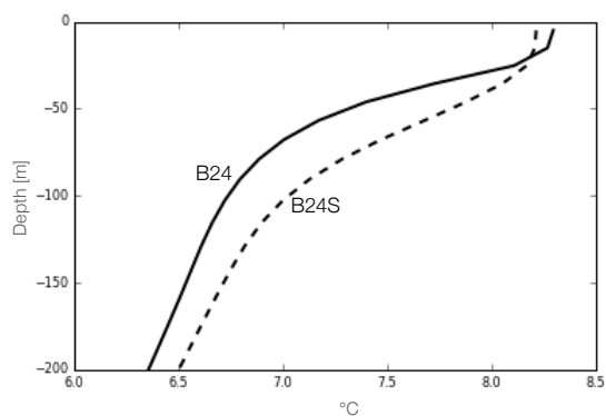
Figure A.9: Five year annual mean vertical temperature ^{\circ}C profiles of the upper 200m comparing B24 and B24S.
