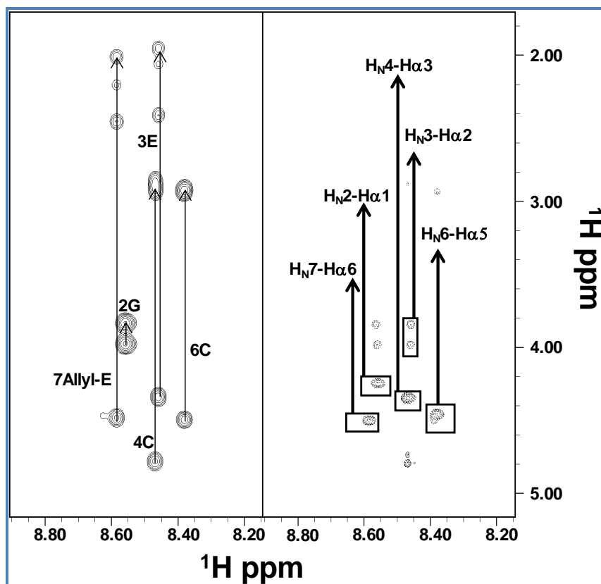
Figure 27. Comparison of 2D [ ^1\text{H} , ^1\text{H} ] TOCSY ( left ) and ROESY ( right ) spectra of PeptideE in \text{H}_2\text{O}/\text{D}_2\text{O} (90/10). The HN-aliphatic protons correlation regions are shown in each panel; spin system assignments are indicated in the left side. In the right panel, sequential ROE contacts are highlighted by rectangles and the corresponding assignments are indicated.
