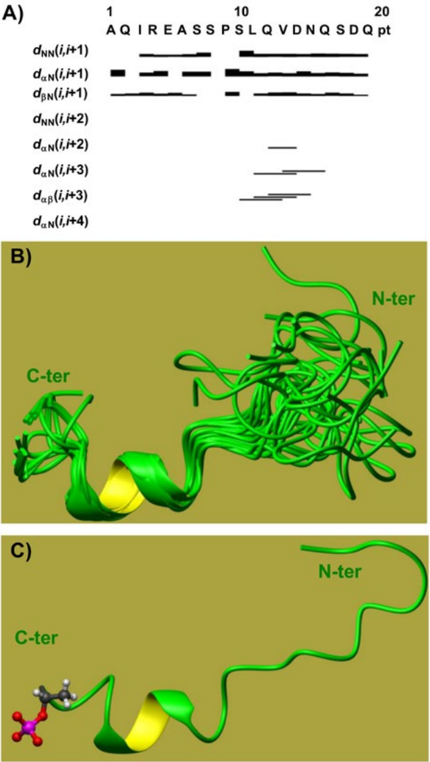
Figure 3. (A) NOE intensity pattern for IDP1 in H 2 O/TFE-d 3 . Only principal short and medium range NOEs are reported. Different residues are specified with the one-letter amino acid code; " d_{\alpha\alpha}(b, c) " designates a NOE contact between the H \alpha and H \alpha protons in the b and c residues respectively. (B) Overlay on the backbone atoms (residues 12-18, RMSD=0.70 ± 0.33 Å) of 20 IDP1 structures. (C) Ribbon representation of the best IDP1 CYANA conformer (i.e. the one with the lowest target function). The D-phospho-Threonine side chain is reported in neon representation. The final CYANA calculation included 143 upl (upper distance limits) of which 60 intra-residue, 73 short- and 10 medium-range.
