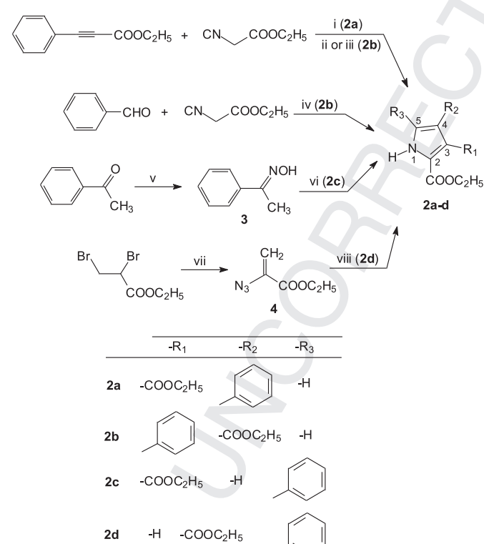
Scheme 1. Synthesis of phenyl-1 H -pyrrole-diester 2a–d ; Reagents and conditions: (i) dppp, dioxane, 100 °C; (ii) Method A: Ag 2 CO 3 , dioxane, 80 °C; Method B: 1) Ag 2 CO 3 , dioxane, 25 °C; 2) 80 °C; Method C: 1) Ag 2 CO 3 , NMP, 25 °C; 2) 80 °C; (iii) Method D: Cu 2 O, phenanthroline, dioxane, 100 °C; (iv) Method E: DBU, THF, 50 °C; (v) H 2 NOH, HCl, Pyridine, EtOH, reflux; (vi) 1) H 5 C 2 OOC–C≡C–COOC 2 H 5 , DABCO, toluene, 80 °C; 2) 170 °C, P; (vii) NaN 3 , DMF, 65 °C; (viii) C 6 H 5 –CO–CH 2 –COOC 2 H 5 , Mn(OAc) 3 2H 2 O, 40 °C.
