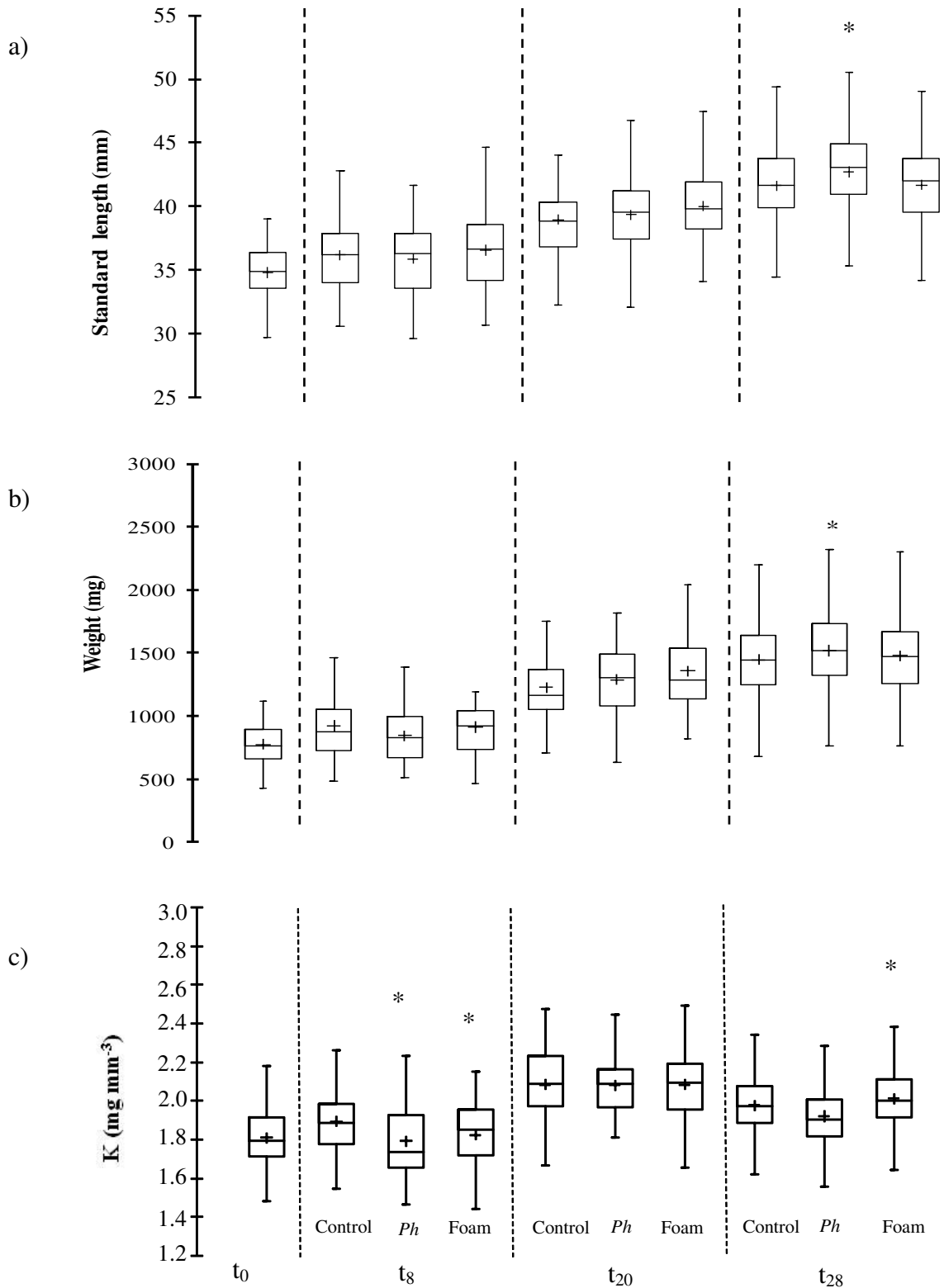
Figure 35. Box and whisker plots of sea bass juvenile size: standard length (a; mm), weight (b; mg) and Fulton's condition index K (c; \text{mg mm}^{-3} ) in control, Phaeocystis and Foam treatments for each sampled week ( t_0 , t_8 , t_{20} and t_{28} ). Whiskers extend to the highest and lowest values. Median (-) and arithmetic mean (+) are also indicated.
