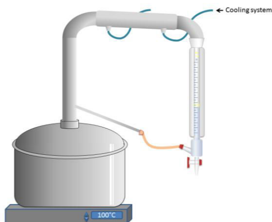
Figure III-5: Hydrodistillation apparatus
