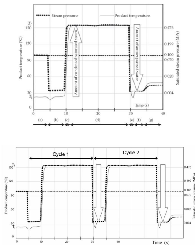
Figure III-7: Instant controlled pressure drop (DIC) cycle.
