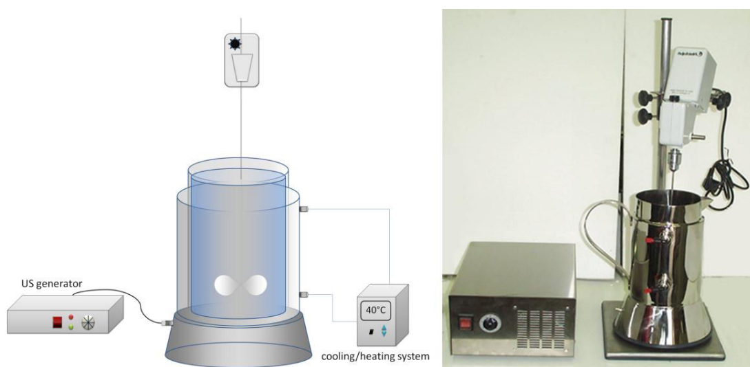
Figure III-8: Ultrasound apparatus
