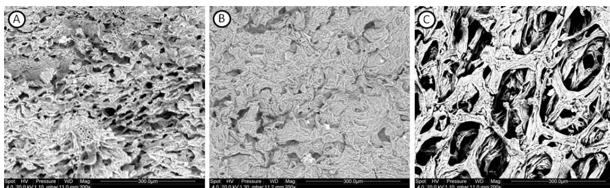
Figure III-15 Scanning Electron Micrographs of untreated dried orange peel (A); HD-treated dried orange peel (B); DIC-treated dried orange peel (C) zoomed 200 times
