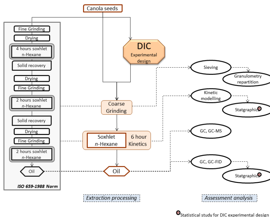
Figure IV-1. Experimental Protocol
