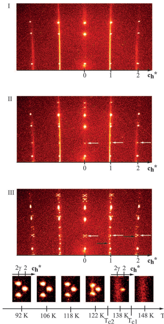
FIG. 2. Section of a channel axis oscillation x-ray image of n -heptane/urea in phases I ( T = 200 \text{ K} ), II ( T = 140 \text{ K} ), and III ( T = 90 \text{ K} ). The detector distance is 300 \text{ mm} . In phases I (host: hexagonal P6_122 ) and II (host: monoclinic P2_111 ), the guest diffraction image appears as diffuse bands perpendicular to \mathbf{c}_g^* . In phase II, white arrows indicate host superstructure Bragg peaks with indices h = 1, k = 2, l = 0, 1, \text{ and } 2 in the low symmetry notation. In phase III, black arrows indicate guest Bragg peaks (1, 1, 0, 1) and (1, 1, 0, 2) appearing on the diffuse bands. Bottom: enlargement of the reciprocal zone around the (1, 2, 2, 0) and (1, 1, 0, 2) Bragg peaks showing the host periodicity (at 2) and guest periodicity (at 2\gamma = 1.962 ) along the aperiodic \mathbf{c}^* direction.
