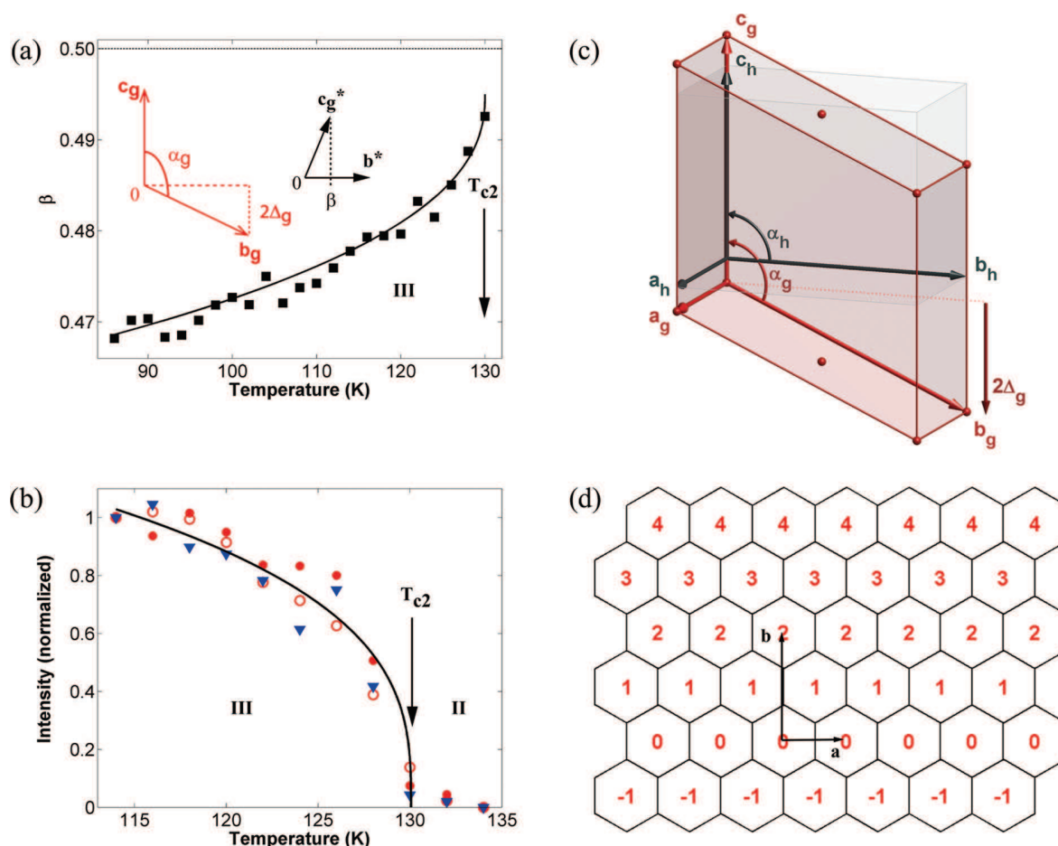
FIG. 6. (a) Temperature evolution of the misfit parameter \beta = 2\Delta_g/c_g (black squares). (b) Temperature evolution of the intensity of the guest Bragg peaks l = 0 and m = 1 (solid red circles), l = 0 and m = 2 (open red circles), and satellite Bragg peaks l = 1 and m = 1 (blue triangles), all normalized at 114 K. (c) Schematic representation of n -heptane/urea in phase III with mean host and guest monoclinic cells. In the limit of precision of our measurements, the angle \alpha_h is found to be 90^\circ . The difference between the lengths of c_h and c_g has been exaggerated. Furthermore, a different origin along the channel direction is given for host and guest subsystems to stress the fact that they are aperiodic in this direction. (d) Projection of the unit cells along the channel axis. In the projection, the urea substructure is represented as black hexagons, and the normal basis vectors \mathbf{a} and \mathbf{b} are drawn as black arrows. The red numbers indicate the relative positions of alkane molecules along the channel axis, in \Delta_g units.
