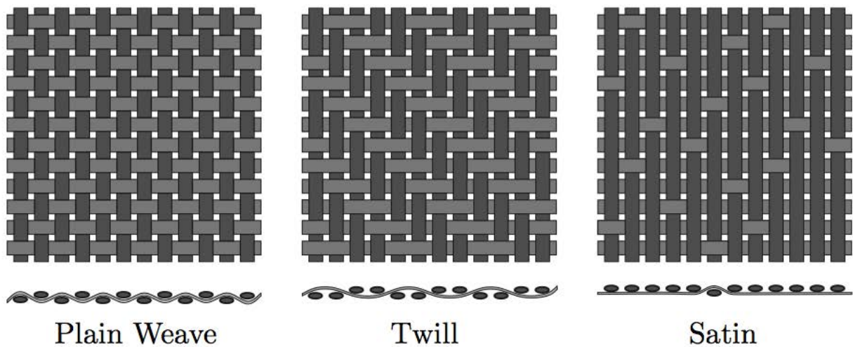
Figure 1.8: Schemes of weaving for fibrous composite reinforcements
