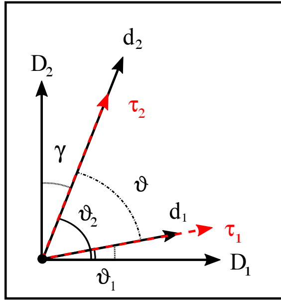
Figure 4.3: Defined angles
