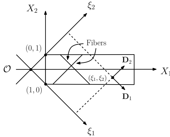
Figure 5.2: Material axes and fibers directions.
