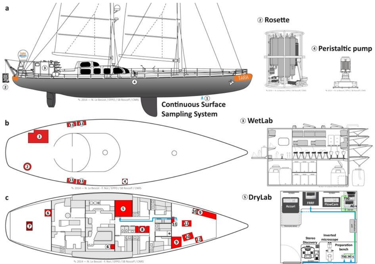
Figure 1.14. Sampling devices and working areas on-board SV Tara are shown from the vessel's (a) side-view, (b) bird's-eye-view of the deck, and (c) inside-view. They consist of the (1) continuous surface sampling system; (2) CTD-rosette; (3) wet lab; (4) peristaltic pump for large-volume sampling; (5) dry lab; (6) oceanography engineers working areas; (7) winch; (8) video imaging area; (9) storage areas at room temperature; (10) storage areas at +4°C and -20°C; (11) MilliQ water system (12) diving equipment, and (13) storage boxes. Water flow from the continuous surface sampling system to the dry lab is shown in blue. (Taken from Pesant et al., 2015).
