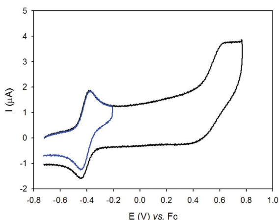
Fig. 7 Cyclic voltammograms of 8 ( \text{CH}_2\text{Cl}_2 + 0.1 M [n\text{-Bu}_4\text{N}]\text{PF}_6 , Glassy carbon electrode, scan rate 0.1 V \text{s}^{-1} , vs. \text{Fc}^+/\text{Fc} ).
