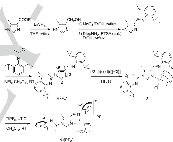
Scheme 9. Synthesis of H C2 L', 8 and 9 + [PF 6 ] - .
