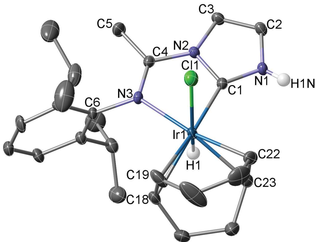
Figure S5. Molecular structure of 8^+ in 8^+[\text{BF}_4]^- . H atoms omitted for clarity, except H1(N1) and H1(Ir). Thermal ellipsoids are at the 30% level. Selected bond lengths (Å) and angles ( ^\circ ): C1–N1 1.327(3), C1–N2 1.371(3), C2–N1 1.397(4), C2–C3 1.345(4), C3–N2 1.392(3), C4–N2 1.391(3), C4–N3 1.290(3), C4–C5 1.486(4), C6–N3 1.452(3), Ir1–Cl1 2.4901(8), Ir1–C1 1.983(2), Ir1–N3 2.125(2), Ir1–C18 2.281(3), Ir1–C19 2.287(3), Ir1–C22 2.180(3), Ir1–C23 2.191(3), C18–C19 1.367(6), C22–C23 1.375(6); N1–C1–N2 105.0(2), C1–Ir1–N3 77.45(9), C1–Ir1–C22 97.10(12), C1–Ir1–C23 97.03(11), N3–Ir1–C18 95.69(10), N3–Ir1–C19 103.11(14), C1–Ir1–Cl1 82.23(8), N3–Ir1–Cl1 87.35(6).
