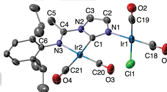
Figure 7. Molecular structure of 11 . Thermal ellipsoids are at the 30% level. Selected bond distances (Å) and angles ( ^\circ ): C1-N1 1.336(9), C1-N2 1.391(9), C2-N1 1.386(9), C2-C3 1.351(1), C3-N2 1.392(8), C4-N2 1.378(9), C4-N3 1.302(9), C4-C5 1.47(1), C6-N3 1.443(8), C1-Ir2 2.052(7), N3-Ir2 2.097(6), C20-Ir2 1.838(8), C21-Ir2 1.907(8), N1-Ir1 2.074(6), C11-Ir1 2.339(2), C18-Ir1 1.848(9), C19-Ir1 1.85(1), C18-O1 1.15(1), C19-O2 1.14(1), C20-O3 1.148(9), C21-O4 1.131(9); N1-C1-N2 106.6(6), C1-Ir2-N3 77.5(2), C1-Ir2-C20 97.6(3), C20-Ir2-C21 89.9(3), C21-Ir2-N3 95.0(3); N1-Ir1-C11 86.6(2); N1-Ir1-C19 91.8(3); C18-Ir1-C19 88.9(4); C18-Ir1-C11 92.7(3).
