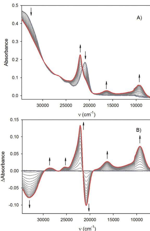
Fig. 8 (A) Time-resolved UV-visible-NIR spectra of 8 for the first oxidation step (transition Rh(I)/Rh(I) to Rh(I)/Rh(II)) in \text{CH}_2\text{Cl}_2 + 0.1 M [n\text{-Bu}_4\text{N}]\text{PF}_6 (spectra recorded every 5 s). (B) Time-resolved UV-visible-NIR differential spectra for the first oxidation step.
