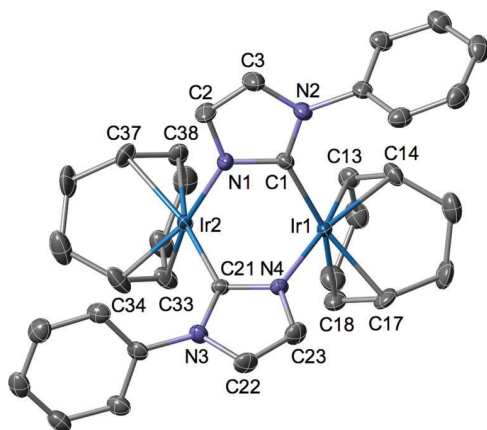
Fig. 2 View of the molecular structure of 3_{\text{H-T}} , H atoms and methyl groups are omitted for clarity. Thermal ellipsoids are at the 30% level. Selected bond lengths (Å) and angles (°): Ir1...Ir2 3.1407(2), C1–N1 1.349(5), C1–N2 1.373(5), Ir1–C1 2.058(4), Ir1–N4 2.068(3), Ir1–C13 2.121(4), Ir1–C14 2.112(4), Ir1–C17 2.166(4), Ir1–C18 2.158(4), C13–C14 1.409(6), C17–C18 1.390(6), C21–N3 1.378(5), C21–N4 1.335(5), Ir2–N1 2.067(3), Ir2–C21 2.043(4), Ir2–C33 2.135(4), Ir2–C34 2.118(4), Ir2–C37 2.168(4), Ir2–C38 2.159(4), C33–C34 1.404(7), C37–C38 1.395(6); N1–C1–N2 106.1(3), N3–C21–N4 106.7(3), C1–Ir1–N4 86.9(1), C13–Ir1–C14 38.9(2), C14–Ir1–C17 82.0(2), C17–Ir1–C18 37.5(2), C18–Ir1–C13 81.2(2), N1–Ir2–C21 86.6(1), C33–Ir2–C34 38.6(2), C34–Ir2–C37 82.0(2), C37–Ir2–C38 37.6(2), C38–Ir2–C33 81.2(2).
