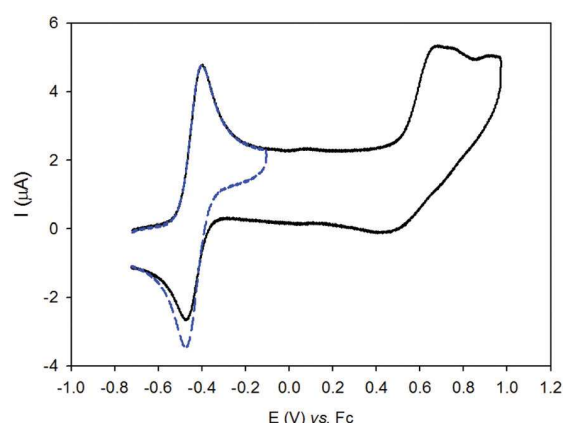
Fig. 5 Cyclic voltammograms of 3 H-T (CH 2 Cl 2 + 0.1 M [n-Bu 4 N]PF 6 , glassy carbon electrode, scan rate 0.1 V s -1 , vs. Fc +/0 ).
