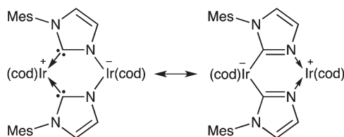
Scheme 5 Limiting resonance structures for the diiridium(I) complex 3_{\text{H-H}} emphasising the dipolar nature of this isomer.
