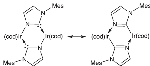
Scheme 6 Limiting resonance structures for 3_{\text{H-T}} .
