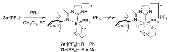
Scheme 8. Synthesis of 7a/b + [PF 6 ] - .
