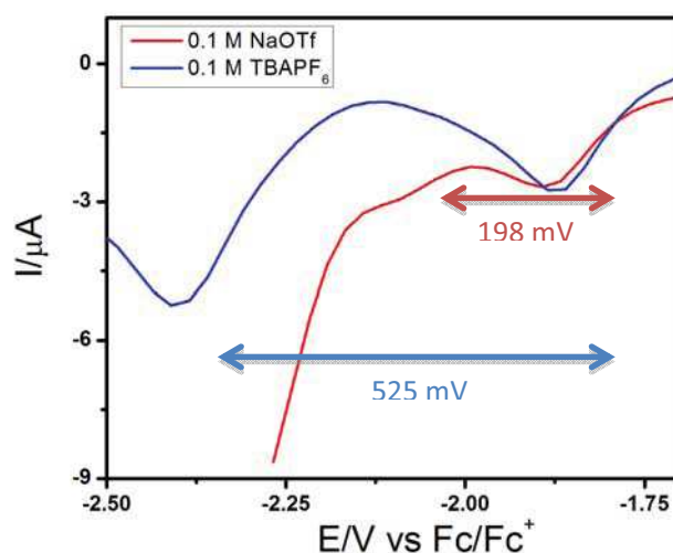
Figure 10. Differential pulsed voltammograms recorded for complex \text{Au}_3\text{-(PC}_{\text{NHCP}})_2 in MeCN at concentration of 1 mM, using a) 0.1 M TBAPF 6 (blue trace) and b) NaOTf (red trace) as supporting electrolyte and GC as working electrode. Pulse height is 0.025 V.
