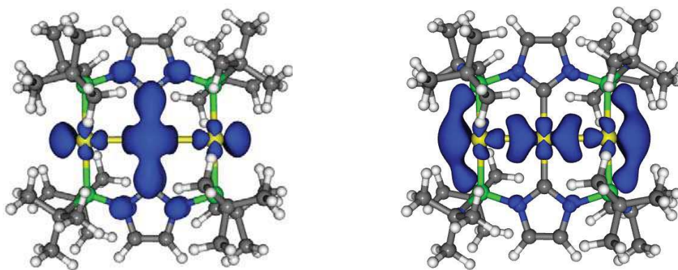
Figure 14. Spin density of the optimized triplet T1 (left) and T2 (right).
