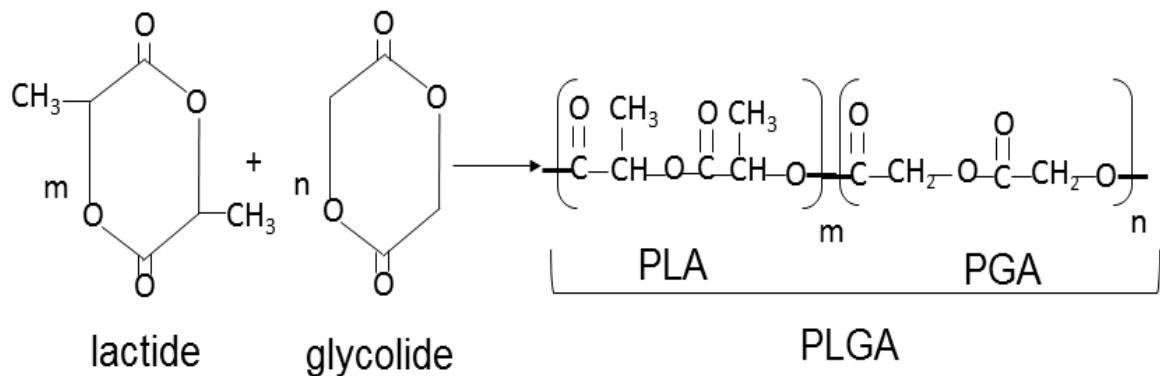
Figure I.3: Structure of poly (lactic-co-glycolic acid) and copolymerization reaction (D'Avila Carvalho erbeta et al., 2012).
