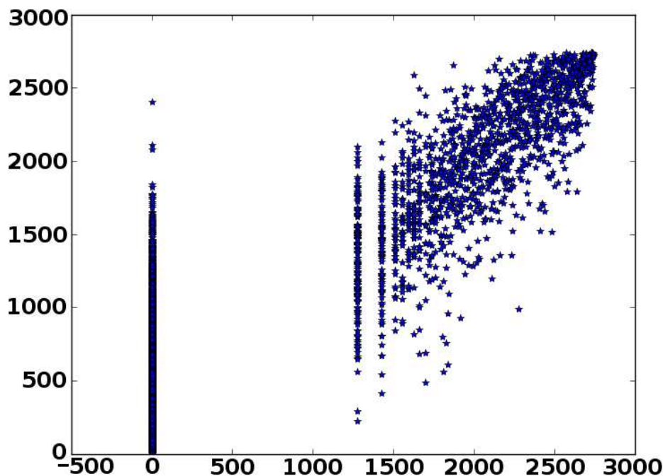
FIGURE 6.18: Comparing the ranking of the middle values of the HPD intervals between the p-value of the proposed statistical method (horizontal axis) and the GE of the RF classifier in the 2D reduced space (vertical axis) in a given ROI of 2742 voxels in the brain.
