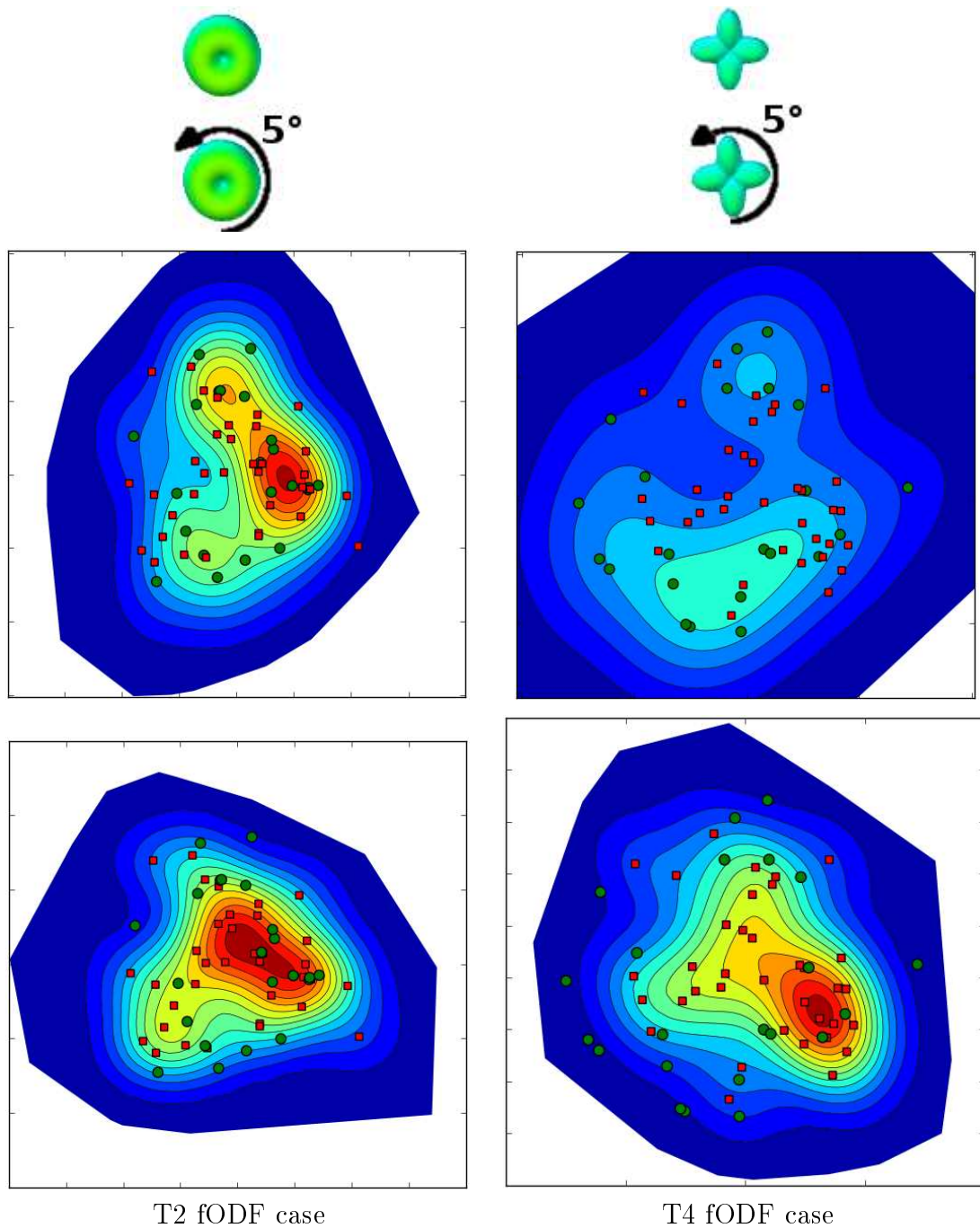
FIGURE 6.9: Statistical comparisons on the T2 and T4 fODF models. The first two rows give an example of two samples from the normal population (first row) and the abnormal population (second row) for both T2 (on the left) and T4 (on the right) fODF models. Abnormal tensors are rotated by 5 degrees in comparison to the normal tensors. The 22 green points correspond to the normal population and the 36 red squares correspond to the abnormal population. All individuals are constructed by adding noise to their corresponding template. The third row depicts the PDF distribution of the normal points, while the fourth row shows the PDF of the abnormal points. We can notice that normal and abnormal distributions are dissimilar in the T4 fODF case and quite similar in T2 fODF case. Populations' PDFs use the same color scale in each case (column). Red color: high density, blue color: low density.
