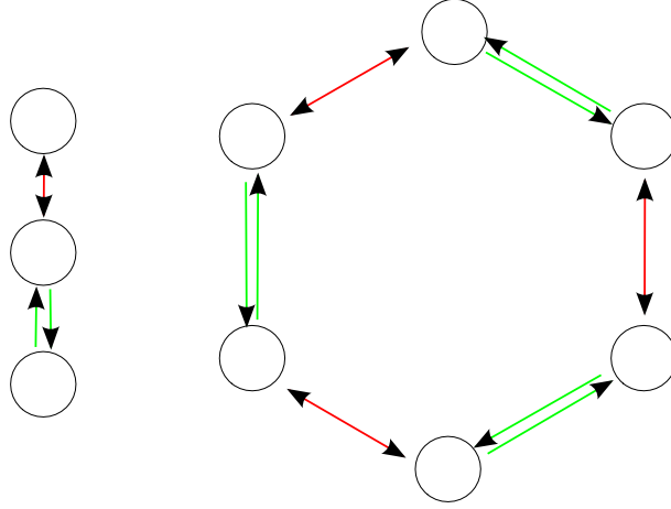
Figure 2.3: The diagram of dualities for SO(4) . In red, we show the action of S -duality on the massive vacua, in green T -duality (when non-trivial).
