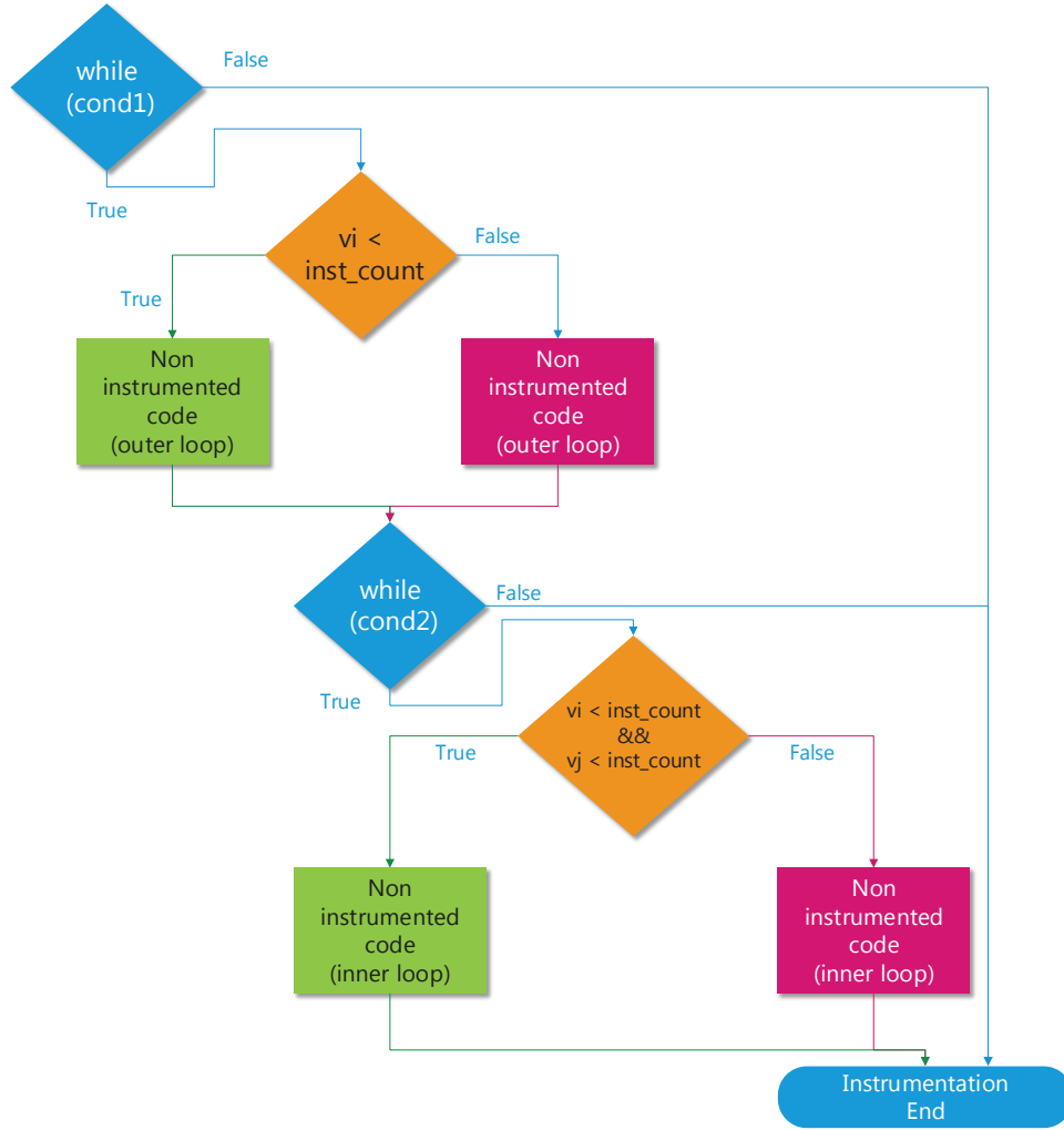
Figure 4.4: Partial instrumentation of loops
