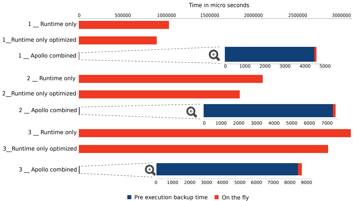
Figure 5.2: Comparison of various backup strategies
