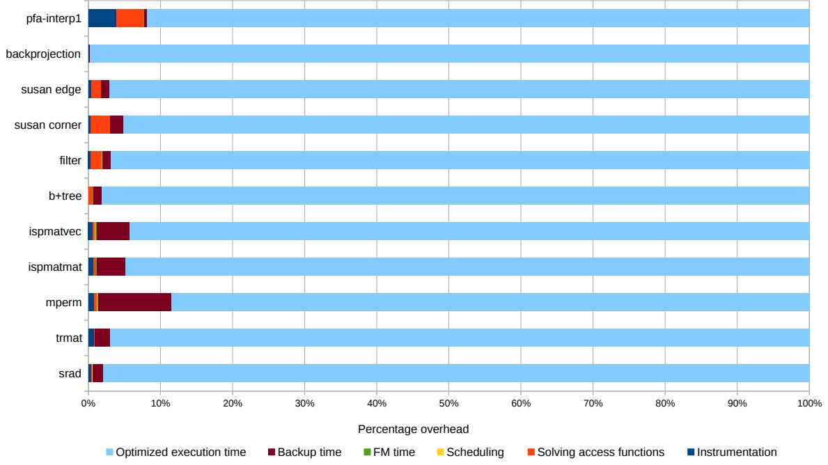
Figure 5.5: Overhead classification in percentage
