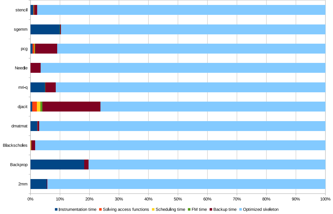
Figure 4.9: Overhead comparison
