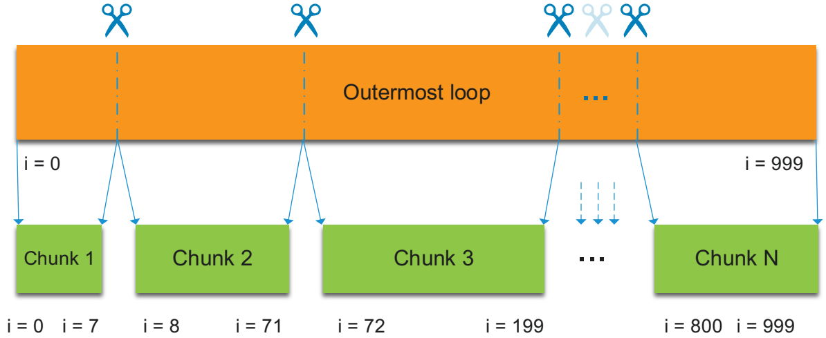
Figure 4.2: Chunking of outer most loop
