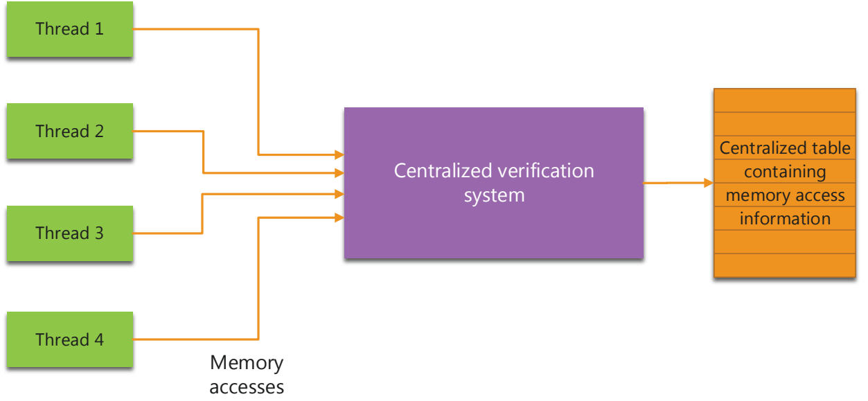
Figure 3.4: TLS: verification
