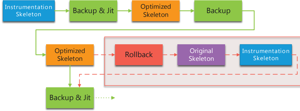
Figure 4.5: Execution flow
