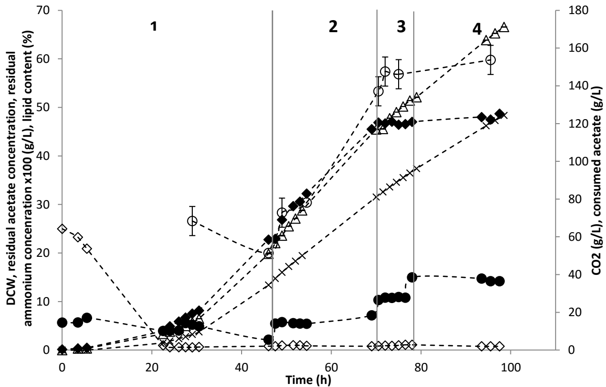
Figure III-11. Results of a fed-batch cultivation of Cryptococcus curvatus in a 7-L fermenter. Time course of dry cell weight (DCW)(♦), lipid content (○), CO 2 production (×), acetate (Δ) consumption, residual acetate (●) and NH 4 + concentration (◇). From 0 to 48 hours, growth was promoted (phase 1). pH was set to 7.0 and regulated with an acetate/NH 4 + feed medium as acidic solution. From the 48 th hour, the feed medium was switched to an acetate feed medium, causing a NH 4 + limitation, to promote lipid accumulation. Manual acetate additions were realized at 48 (phase 2), 70 (phase 3), 78 (phase 4) hours to increase the residual acetate concentrations to, respectively, 5, 10 and 14 g/L. This corresponded to final C/N ratios of, respectively, 300, 500 and 900.
