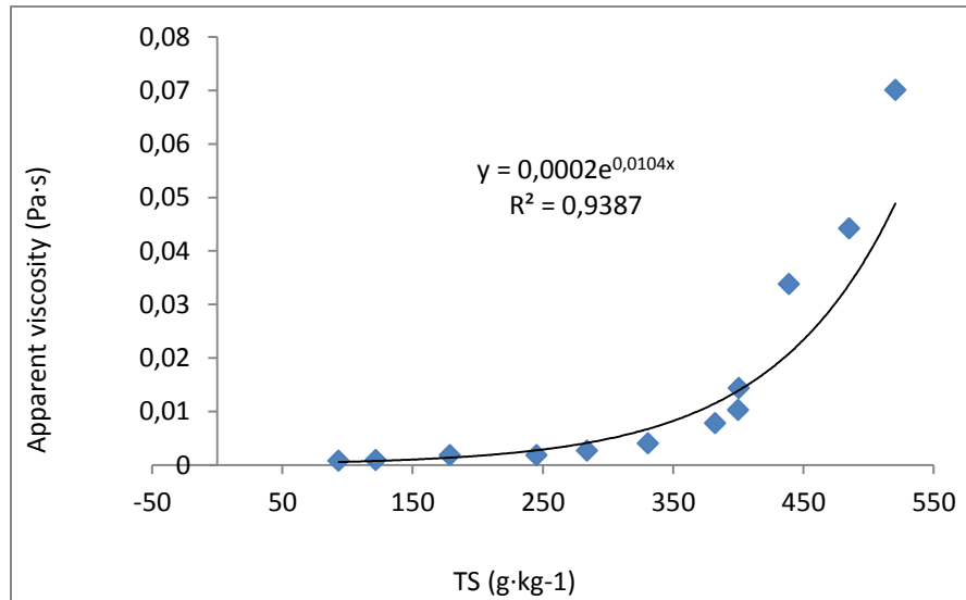
Figure 4.9. Skim milk apparent viscosity ( \eta_{100} ) measured at 60°C in function of total solids contents.
