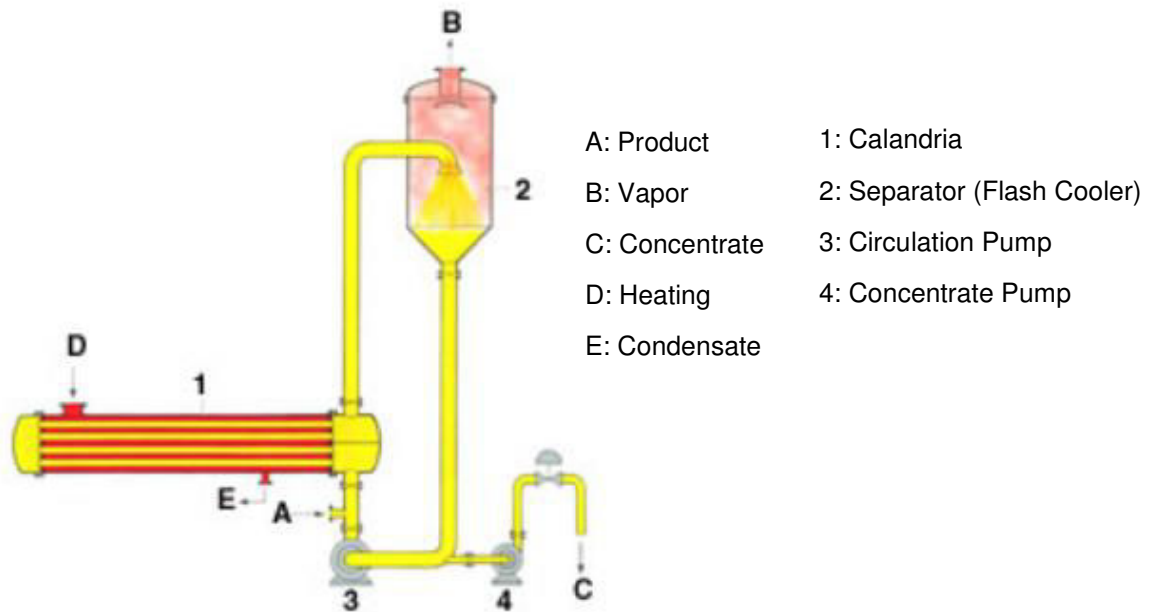
Figure 2.8. Forced circulation evaporator ( www.niroinc.com ).
