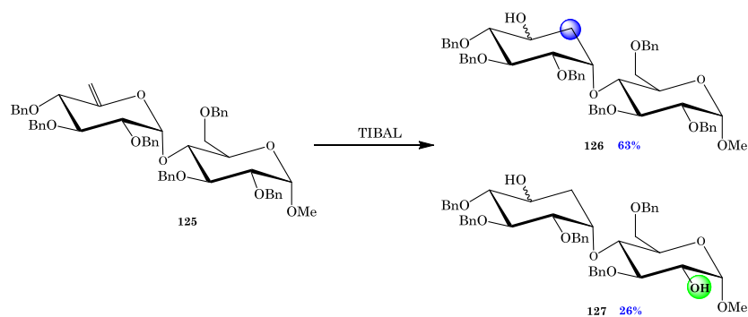
Scheme II-19: Discovery of the debenzylation reaction
