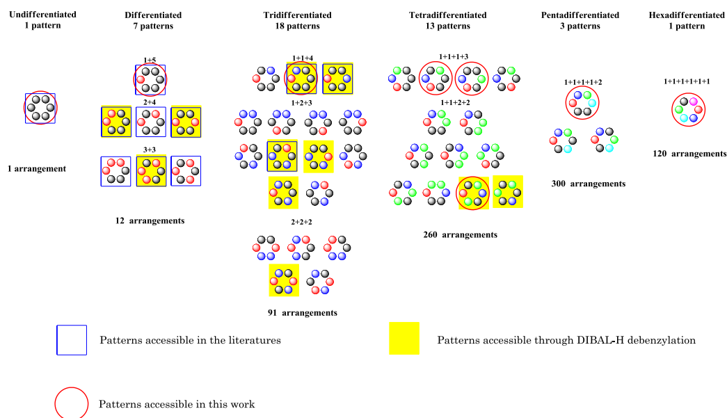
Figure III-4: Functionalization patterns
