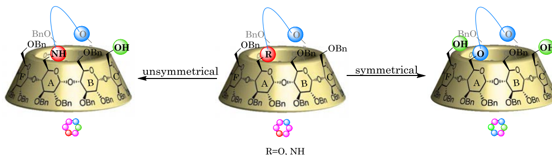
Scheme II-31: Symmetrical/unsymmetrical bridges induced debenzylation
