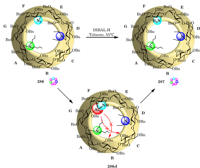
Scheme V-5: DIBAL-H-mediated debenzylation on cyclodextrin 286
