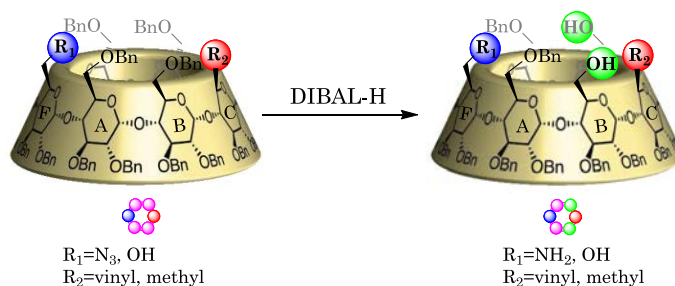
Scheme II-30: “Frustration” strategy induced double-deprotection
