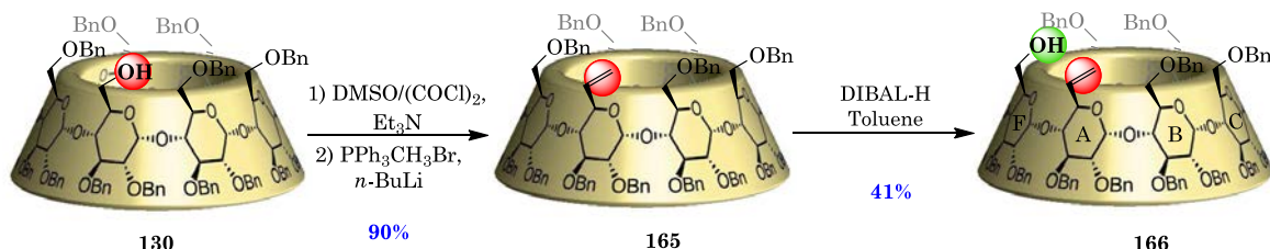
Scheme II-34: Regioselective mono-debenzoylation of vinyl- \alpha -cyclodextrin
