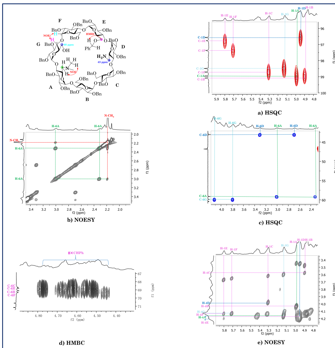
Figure V-4: NMR (600 MHz, 300K, \text{CDCl}_3 ) analysis of cyclodextrin 290
