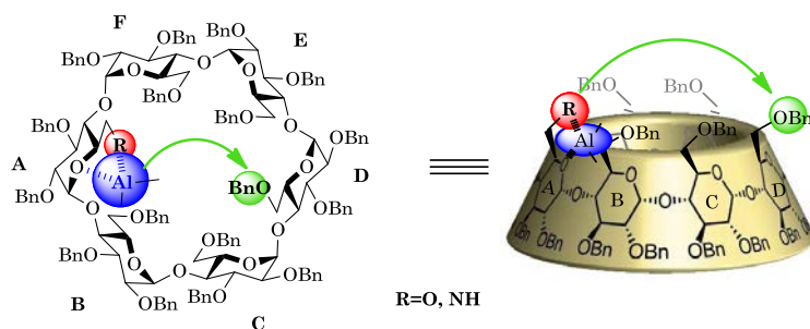
Figure II-7: Steric hindrance orients the farthest debenzoylation
