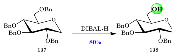
Scheme II-23: DIBAL-H deprotection on 1-deoxy sugar
