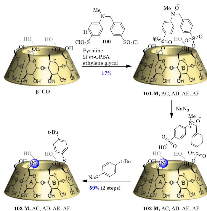
Scheme II-12: “Flamingo” cap used on \beta -cyclodextrin
