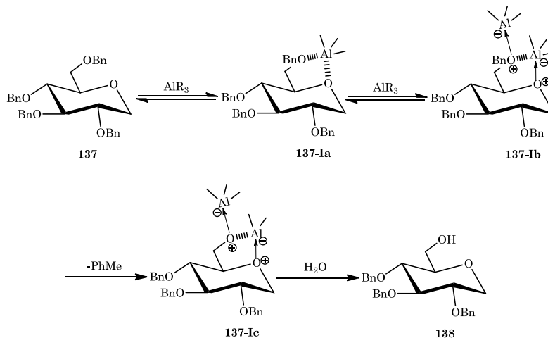
Scheme II-24: Mechanism of DIBAL-H induced debenzilylation on sugar
