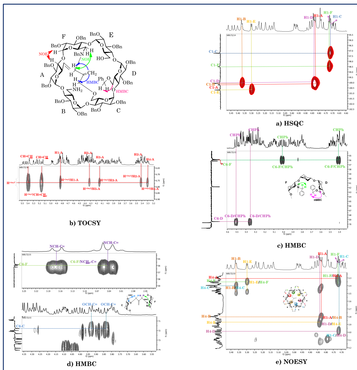
Figure III-3: NMR (600 MHz, 300 K, CDCl 3 ) analysis of cyclodextrin 246
