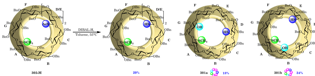
Scheme V-15: Formation of tetradifferentiated cyclodextrins
