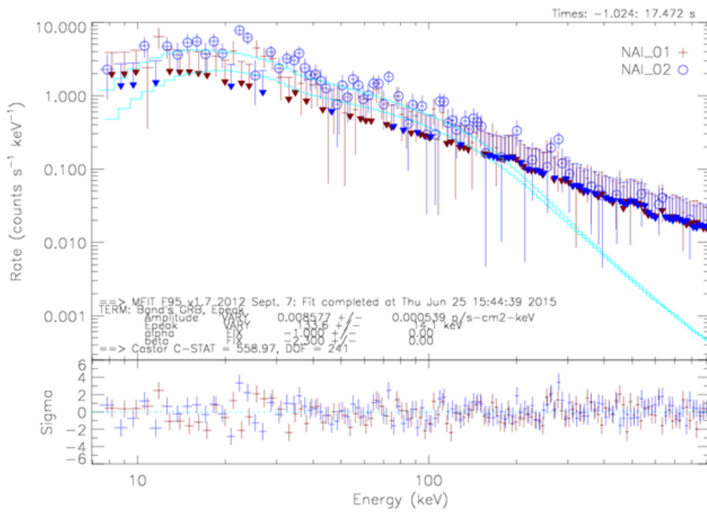
FIGURE 3.6: The spectrum of the prompt emission, included two pulses (indicated as total in Tab. 3.4).
