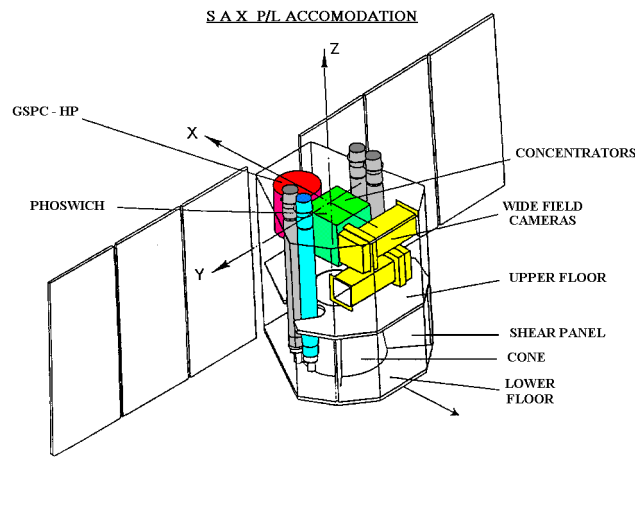
FIGURE 1.4: BeppoSAX instrument. Credit: NASA/BeppoSAX
