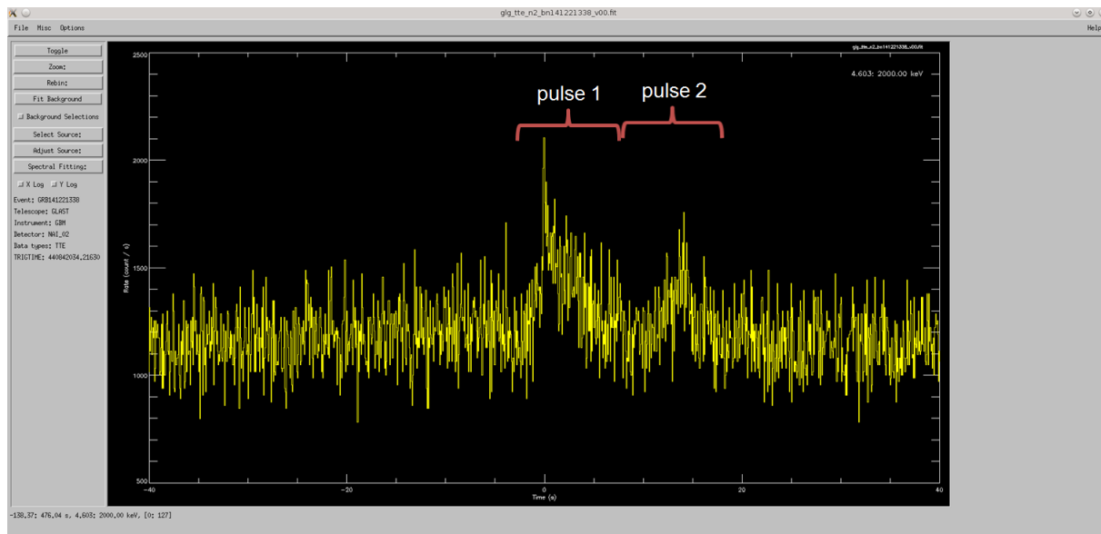
FIGURE 3.5: The two pulses shown from the observation of Fermi satellite for GRB 141221A.
