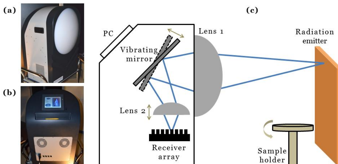
Figure III.2: (a), (b) Photograph and (c) setup of the Millicam90 system from MC2 company.
