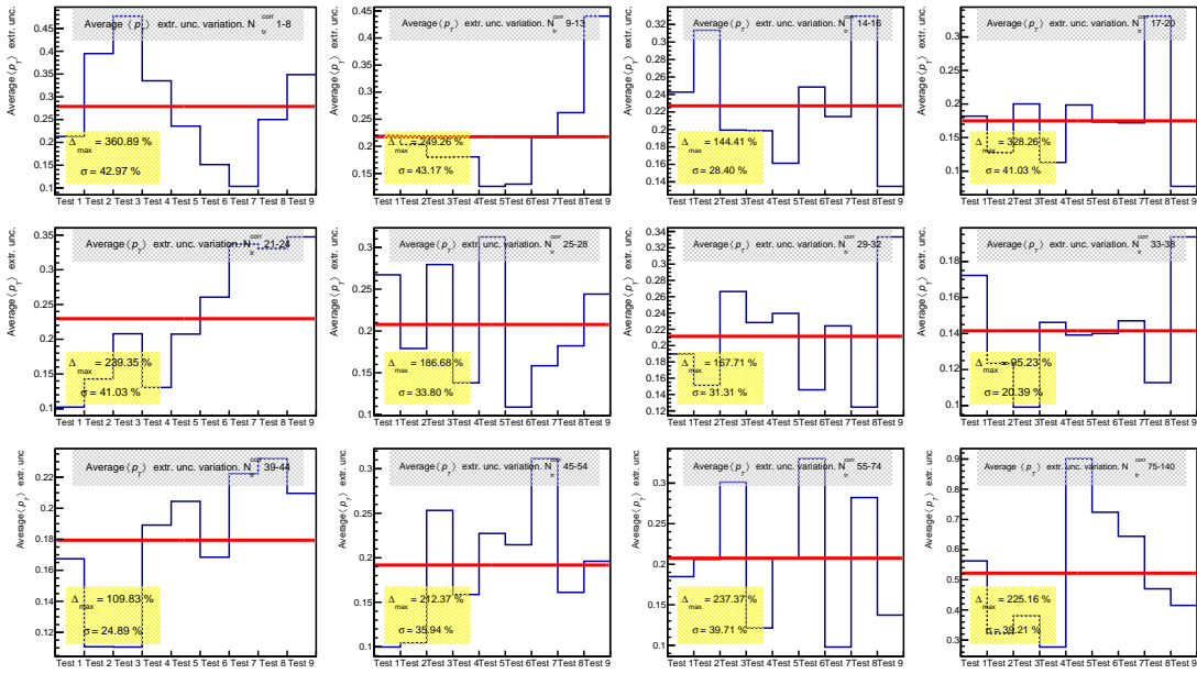
Figure 7.6: Relative J/\psi \langle p_T \rangle extraction systematic uncertainty variations due to bin flow in multiplicity bins in Pb-p. Each value corresponds to the result of a set of extraction tests (Fig. 7.5) for a given execution test. The difference between the most different results ( \Delta_{max} ), mean value (red line) and 1\text{-}\sigma dispersion among the values are shown.
