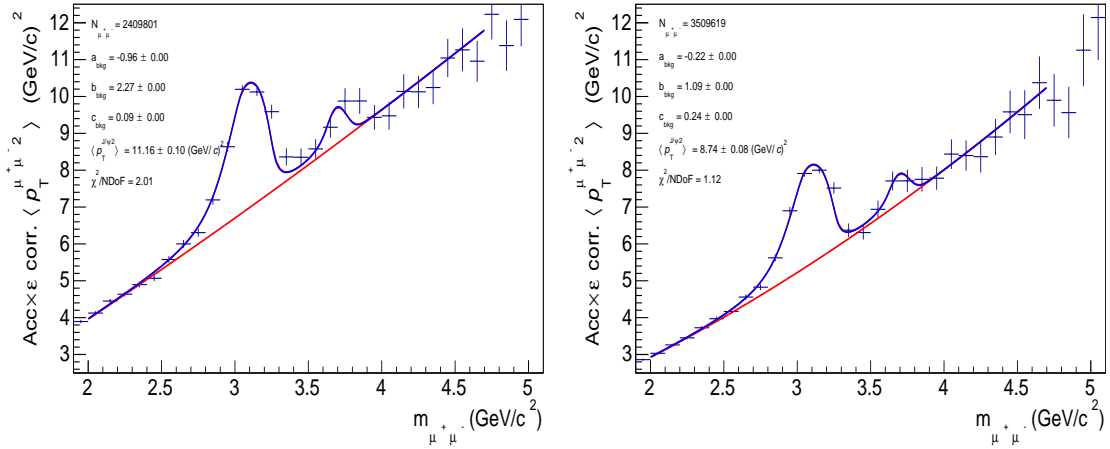
Figure 7.12: Multiplicity integrated \mathcal{A}\times\epsilon corrected di-muon <p T 2 > spectra in p-Pb (left) and Pb-p (right) collisions. The spectra are fitted with a fit combination choice (CB2+VWG+Range inv.mass = 2.0-5.0+σ ψ(2S) = 1.1 · σ J/ψ +Pol2+Range (p T ) = 2.0-5.0 ) and the values of the extracted J/ψ <p T > are shown.
