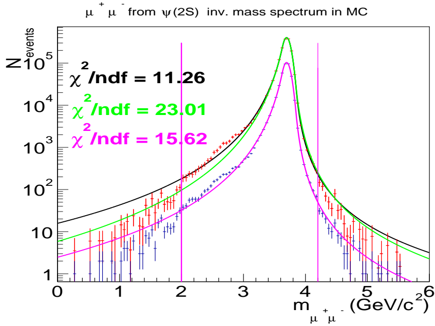
Figure 6.3: Tail fits tests for \psi(2S) on pure signal simulation using an Extended Crystal Ball (CB2) function. The figure shows: raw \psi(2S) spectrum (blue dots), \mathcal{A}\times\epsilon corrected (using J/\psi correction) spectrum (red dots), raw spectrum fit (magenta line), corrected spectrum fit (black line) and corrected spectrum fit using the tails parameters extracted from the corrected J/\psi spectrum (green line). The vertical lines delimit the fitting range.
