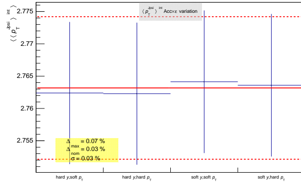
Figure 7.7: Integrated J/\psi \langle p_T \rangle extraction with the four varied \mathcal{A} \times \varepsilon corrections are shown in blue and the nominal result as the red line. The figure also shows the relative difference between the most different results ( \Delta_{max} ), between the nominal value and the more distant value ( \Delta_{nom} ) and the 1-\sigma dispersion among the values ( \sigma ). The systematic uncertainty due to the \mathcal{A} \times \varepsilon is \Delta_{max} which is 0.07%
