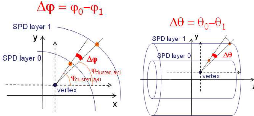
Figure 3.1: Sketch to illustrate the calculation of \Delta\varphi and \Delta\theta used for the tracklet reconstruction. [243]
