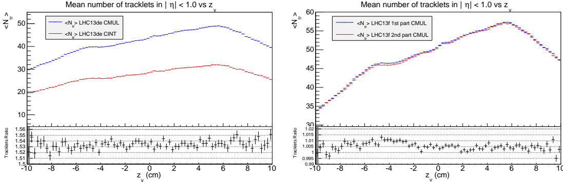
Figure 4.10: Left: Comparison of \langle N_{tr}^{corr} \rangle(z) for MB and CMUL triggers in p-Pb data. Right: Comparison of the two subperiods in Pb-p data for CMUL trigger.
