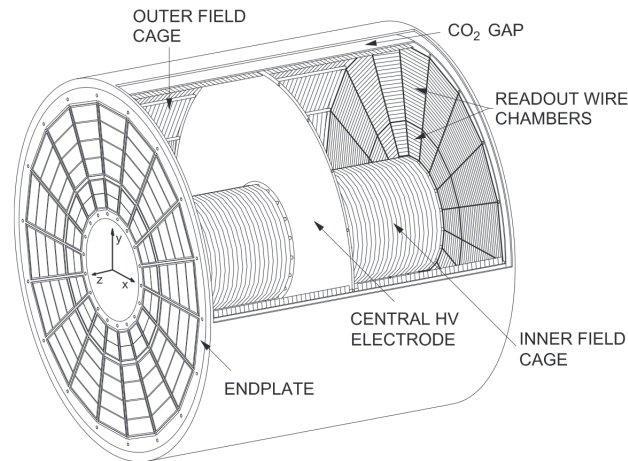
Figure 2.5: The TPC layout. Figure taken from [215] .
