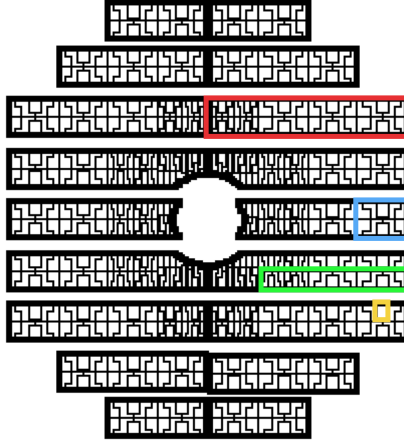
Figure 5.3: Visualization of chamber 6 showing its different substructures: DE (red), PCB (blue), BP (green) and MANU (yellow).
