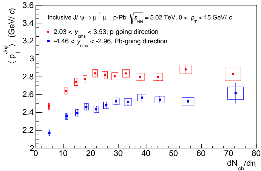
Figure 9.3: J/\psi absolute \langle p_T \rangle as a function of the absolute dN_{ch}/d\eta ( |\eta| < 1 ) in p-Pb collisions at \sqrt{s_{NN}} = 5.02 TeV.
