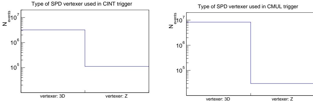
Figure 3.4: Number of events classified depending on the vertexer type used to reconstruct the SPD vertex for CINT (left) and CMUL events (right) in LHC13d+e.
