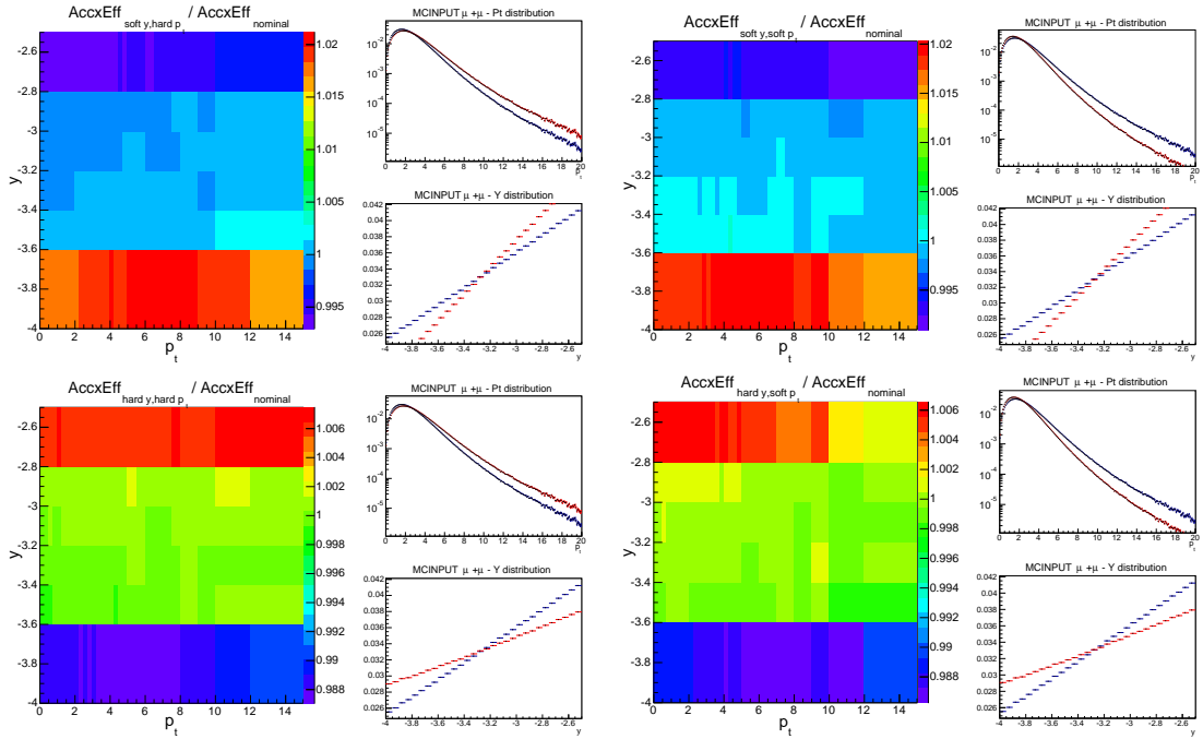
Figure 8.8: \mathcal{A} \times \epsilon variations (ratio of varied over nominal correction) due to changes in the input MC distributions, and the corresponding input distributions (the blue curves represent the nominal and the red curves the varied distributions). The results are shown for four combinations of extreme variations of the p_T and y distributions: soft- y and hard- p_T (top left), soft- y and soft- p_T (top right), hard- y and hard- p_T (bottom left), hard- y and soft- p_T (bottom right).
