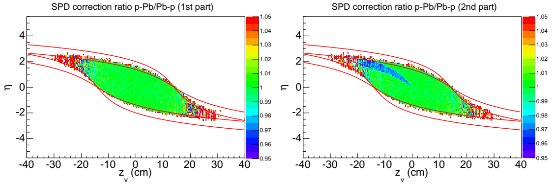
Figure 3.9: SPD \mathcal{A} \times \mathcal{E} ratio to compare the corrections of p-Pb periods with the first (left) and second (right) parts of the Pb-p data-taking periods.
