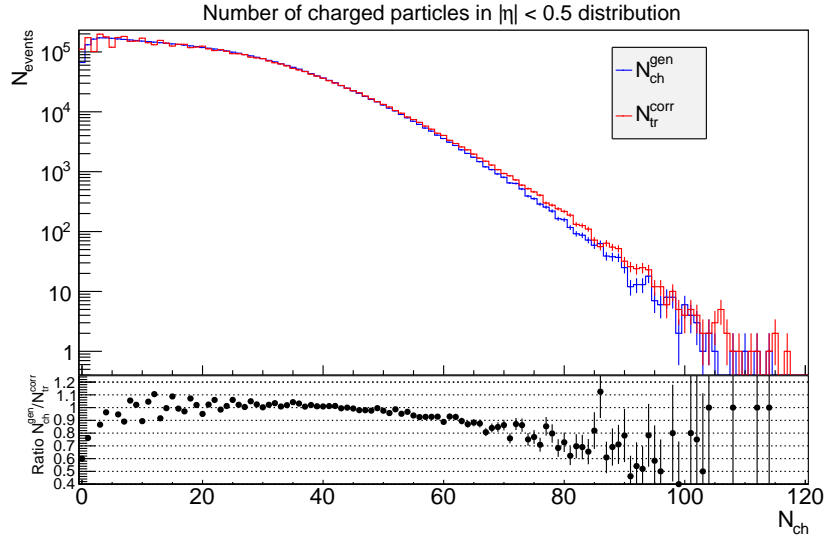
Figure 3.20: N_{tr}^{corr} distribution (red) in p-Pb simulation compared to the generated N_{ch} distribution (blue) and its ratio.
