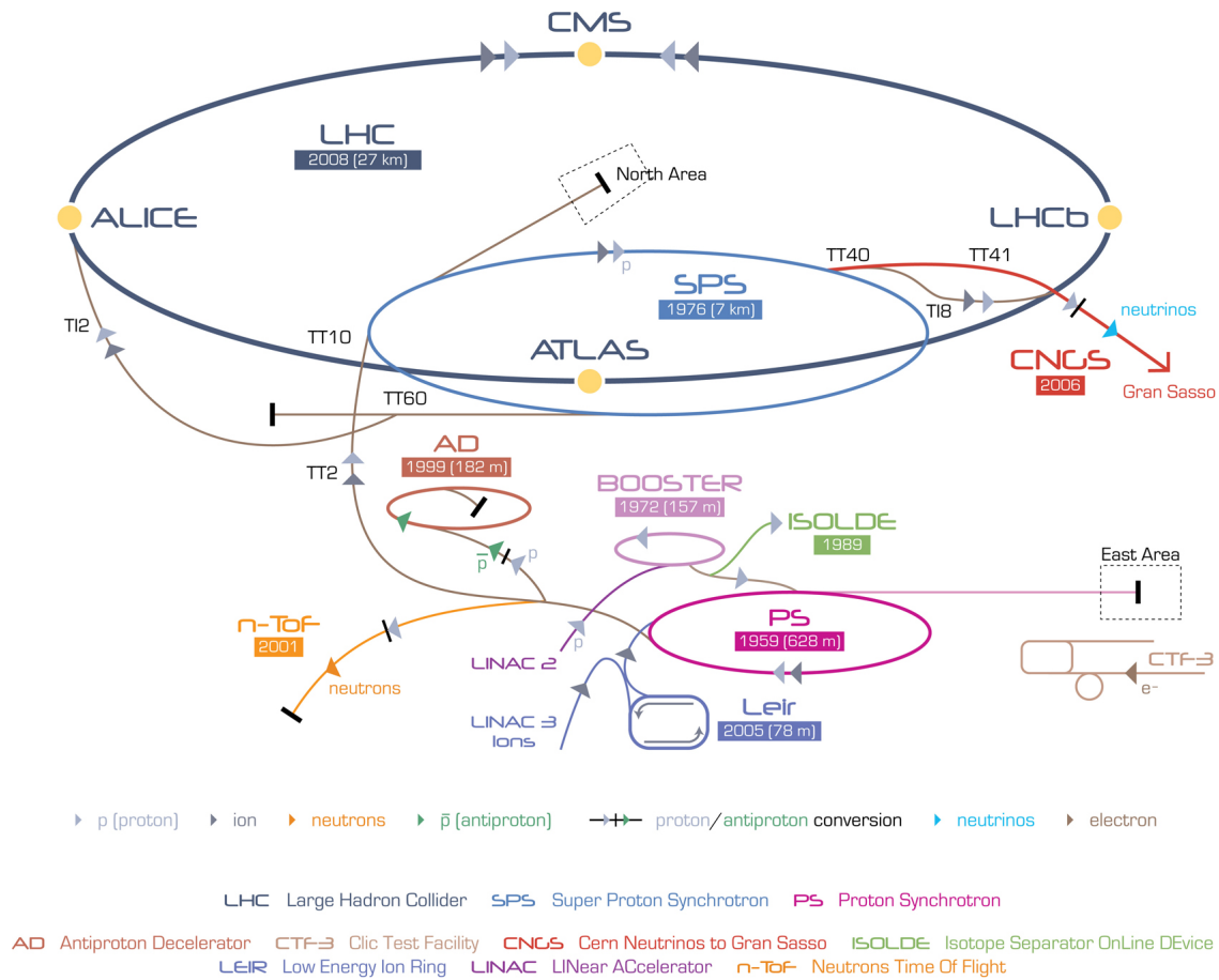
Figure 2.1: The CERN accelerator complex .
