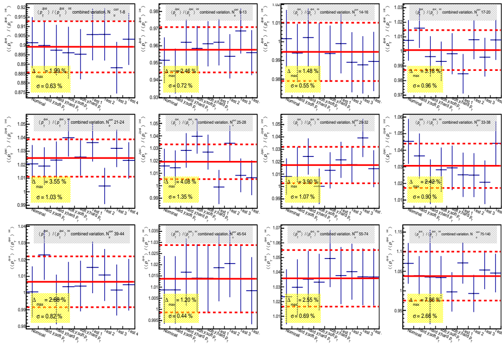
Figure 7.8: Variation on the relative J/\psi \langle p_T \rangle in multiplicity bins due to bin-flow, \mathcal{A} \times \mathcal{E} and signal extraction. The blue points are the average values of the relative \langle p_T \rangle obtained with Eq. 7.4 in each execution test. The red line shows the average of the values obtained from the execution tests in each bin. The dotted line is the statistical error. \sigma is the value of the 1-\sigma dispersion of the values for each execution test in a bin.
