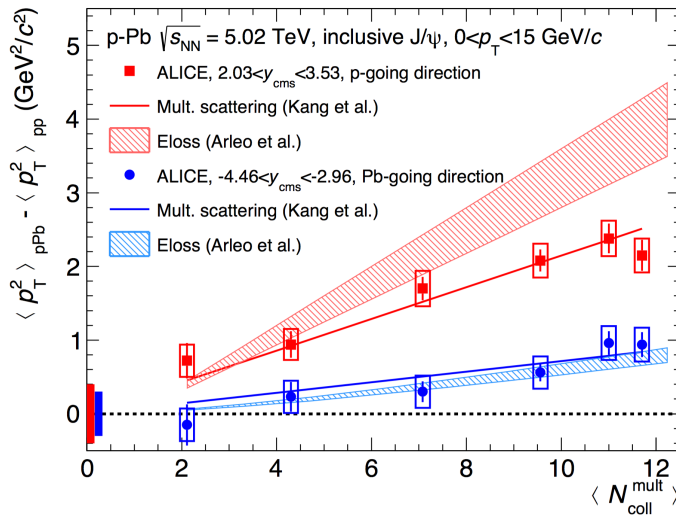
Figure 1.28: J/\psi transverse momentum broadening as a function of N_{coll}^{mult} at backward (blue dots) and forward (red dots) rapidity. The results are compared with theoretical calculations (see text). Figure taken from [5].
