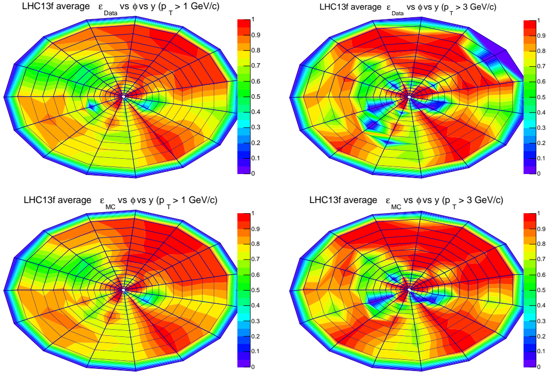
Figure 5.15: Single muon efficiency polar maps ( y, \phi ), for two different p_{\text{T}} cuts, p_{\text{T}} > 1 \text{ GeV}/c (left) and p_{\text{T}} > 3 \text{ GeV}/c (right). The top plots show the efficiency maps for data, and the bottom ones the corresponding maps for MC.
