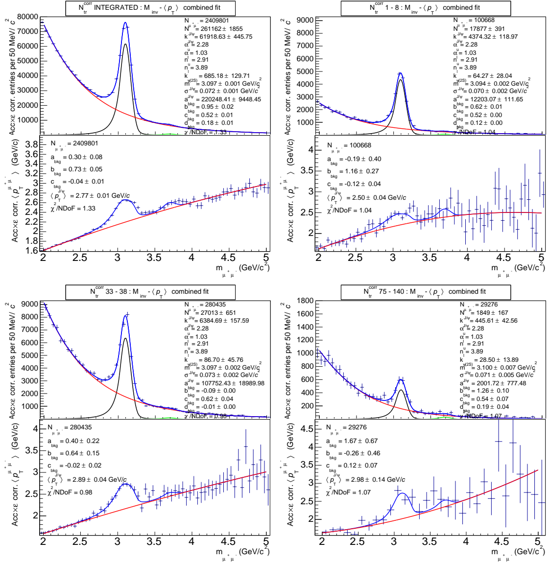
Figure 7.11: Combined fits of invariant mass and di-muon \langle p_T \rangle invariant mass spectra in p-Pb for integrated (top left) and multiplicity bins. The fit combination used is (CB2+VWG+Range inv.mass = 2-5 + \sigma_{\psi(2S)} = 1.1 \sigma_{J/\psi} + Pol2 + Range \langle p_T \rangle = 2-5).
