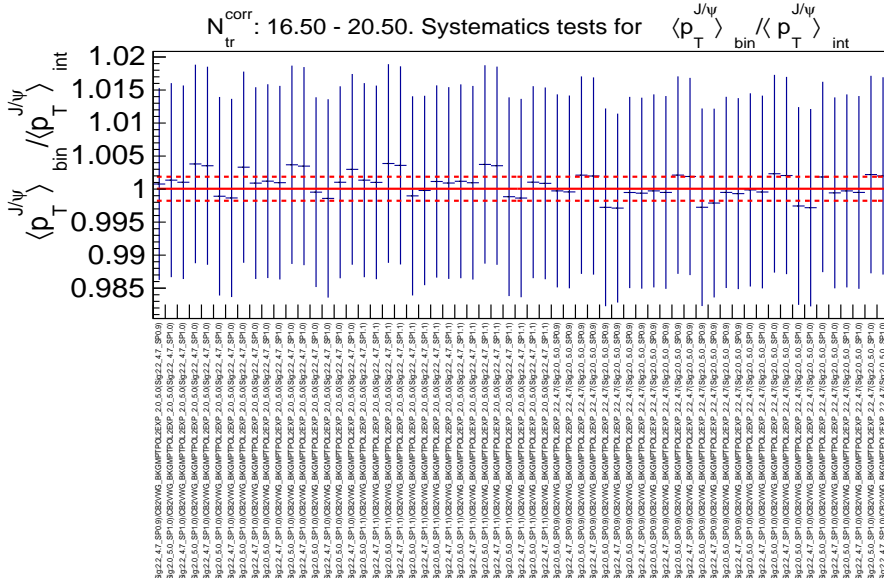
Figure 7.4: Values of \left(\frac{\langle p_T^{J/\psi} \rangle_i}{\langle p_T^{J/\psi} \rangle_{int}}\right)_j relative \langle p_T \rangle extraction tests as a function of j -th test for the J/\psi \langle p_T \rangle systematic uncertainty computation in a multiplicity bin in Pb-p. The unweighted average and the 1\text{-}\sigma dispersion are shown as the red solid and dotted lines respectively. The test-axis is zoomed-in to show only a fraction of the total 1536 tests.
