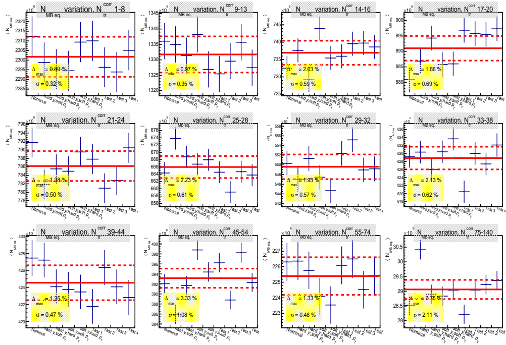
Figure 6.11: p-Pb variation on the number of equivalent MB events in multiplicity bins due to bin-flow. The figure shows the relative difference between the most different results, \Delta_{max} , the mean value (red line), the error on the mean (dotted line) and the 1- \sigma dispersion among the values \sigma .
