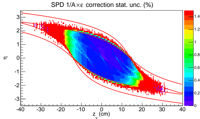
Figure 3.12: Statistical uncertainty of the 1/\mathcal{A} \times \varepsilon(\eta, z_v) correction
