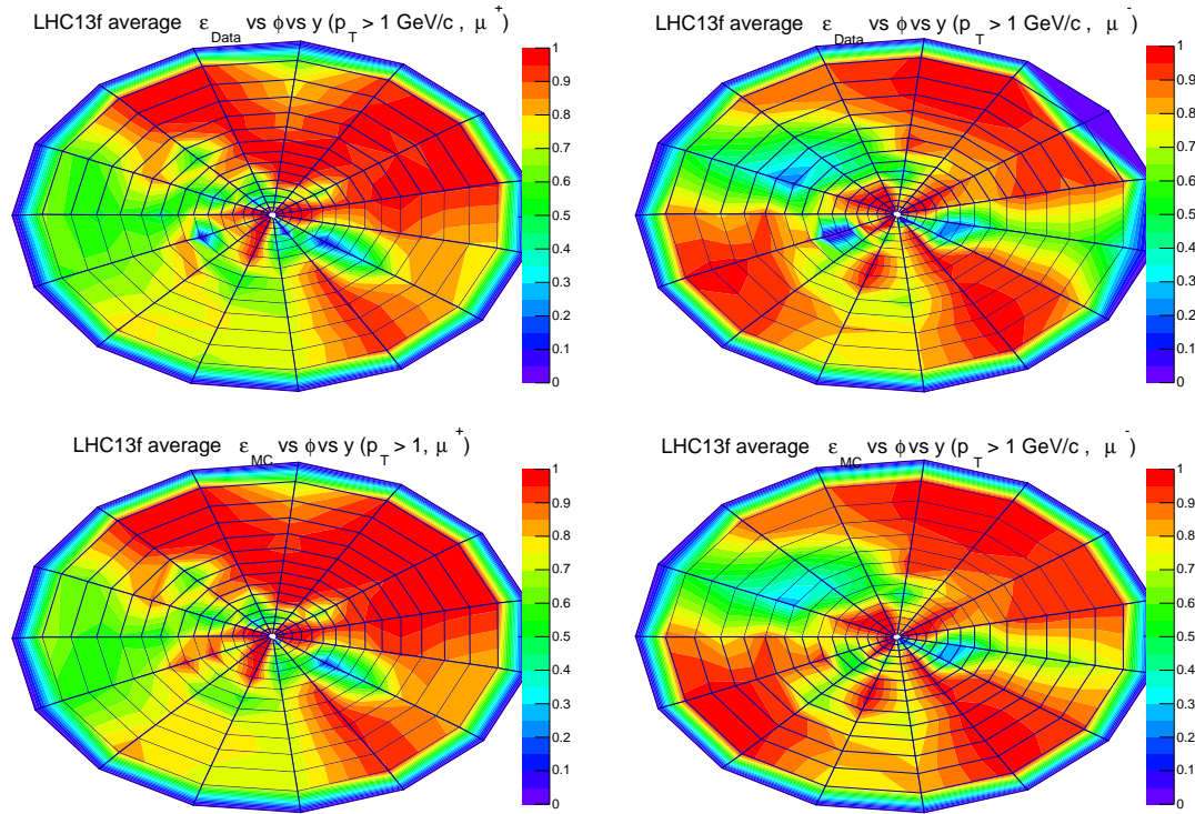
Figure 5.16: Single muon efficiency polar maps ( y, \phi ) (for p_T > 1 \text{ GeV}/c ) for \mu^+ (left) and \mu^- (right). The top plots show the efficiency maps for data, and the bottom ones the corresponding maps for MC.
