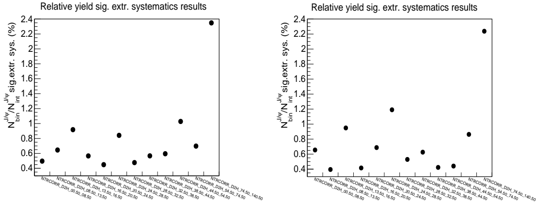
Figure 6.9: (Left) Relative signal extraction systematic uncertainty in multiplicity bins in p-Pb. (Right) Relative signal extraction systematic uncertainty in multiplicity bins in Pb-p. These values are for one single execution of the multiplicity analysis. See also Fig. 6.10 for the final values.
