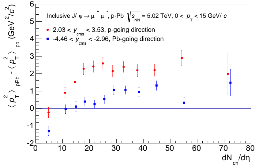
Figure 9.8: J/\psi transverse momentum broadening as a function of charged particle multiplicity ( |\eta| < 1 ) at forward and backward rapidity in p-Pb collisions at \sqrt{s_{NN}} = 5.02 TeV.
