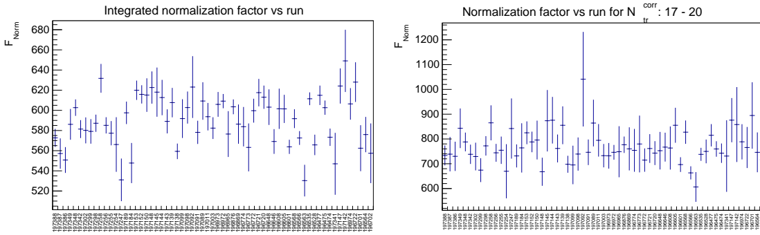
Figure 6.7: Di-muon trigger normalisation factor in Pb-p as a function of run. Left: Integrated in multiplicity. Right: Multiplicity bin N_{tr}^{corr} 17-20.
