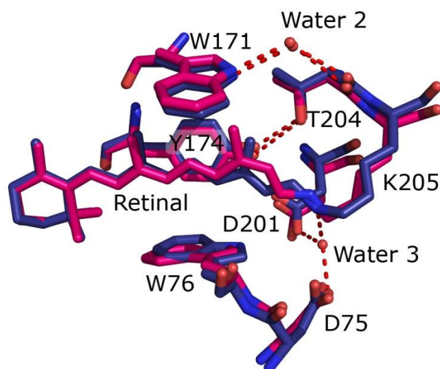
Figure 3.4.5. Comparison of the retinal environment in the NpSR II ground state (blue) and active state (magenta) structures. Note that the active state is a mix of the M and O states, and retinal is shown only as it would be in the M state in 13- cis conformation. Positions of other residues represent the averages of those in the M and O states and reflect the general conformational changes in this region. Hydrogen bonds are shown by dashed lines. Water molecule 3 disappears in the active state.
