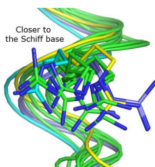
Figure 3.2.10. Conformations of the Arg-82 homologs' side chains in the retinylidene proteins of known structure. The figure is a magnification of a part of the Figure 3.2.2. ESR is shown in dark blue, XR in light blue, ChR in yellow and the other proteins in green. In ESR, Arg-82 occupies the outermost position among the presented proteins.
