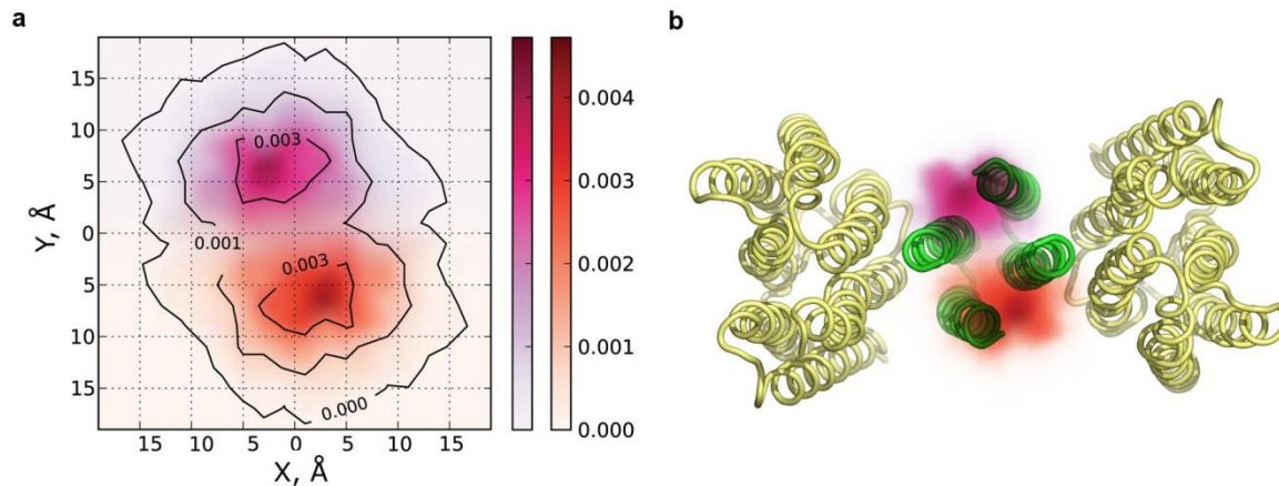
Figure 3.5.10. Displacement of the second HAMP domain in the membrane plane. a) Computed probability of finding the projection of the NpHtrII second HAMP domain center of mass on the membrane plane at the corresponding X, Y coordinates, in 1/\text{\AA}^2 units. View from the cytoplasm. X axis is directed along the centers of mass of the HAMP1 AS1 helices, Y axis is perpendicular to it, and both axes lie in the membrane plane. The initial structure was symmetric, and the tilt and the longitudinal shift in the inter-HAMP region have developed later. Two regions with the highest probability correspond to the two possible signs of longitudinal shifts and are colored red and magenta, correspondingly, to guide the eye. b) The same probability density distribution laid over the structure of NpSRII-NpHtrII 2:2 complex in a proper scale (PDB ID 1H2S).
