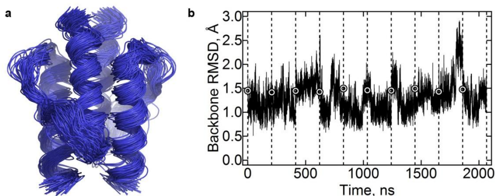
Figure 3.6.1. Stability of the HAMP domain in molecular dynamics simulations. a) Superposition of the conformations observed in the simulations with CHARMM22-CMAP forcefield. The snapshots taken each 20 ns are shown. The domain remains stable during the simulations. b) Root-mean square deviation of the backbone atom positions relative to the average observed in the simulations with CHARMM22-CMAP forcefield. The mean value is 1.3 Å. The data for ten trajectories are shown consecutively; they are separated by the dashed lines. The circles denote the value at the start of each trajectory.
