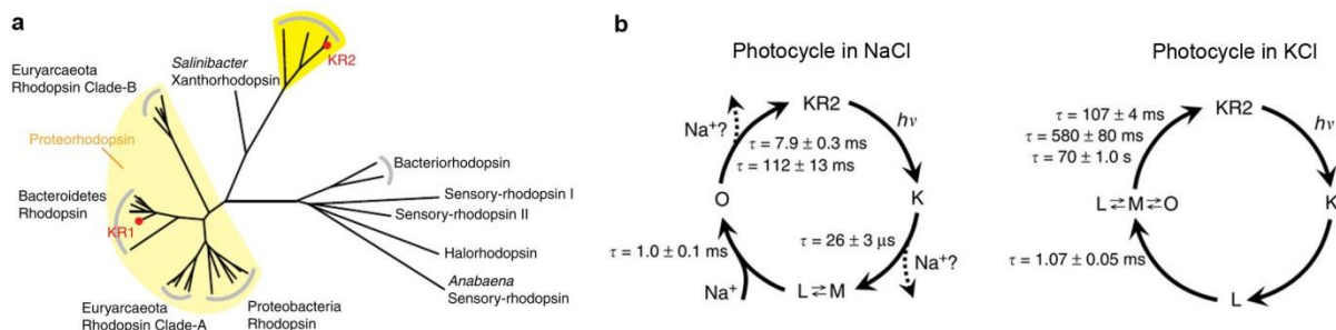
Figure 1.1.6 Position of Krokinobacter rhodopsins in the phylogenetic tree (a) and KR2 photocycles in NaCl and KCl (b) 58 .
