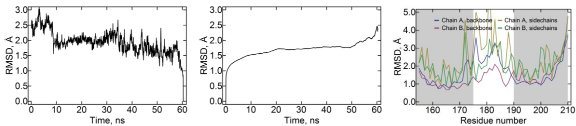
Figure 2.5.10. Structure stability of the NpHtrII HAMP2 domain as a part of the whole HAMP domain region (model 10 in section 2.5.3).
