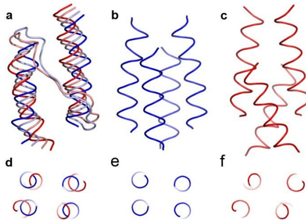
Figure 3.6.4. Conformational changes associated with the first principal component. a,b,c) Side view of the HAMP domain. d,e,f) View along the HAMP domain axis. The extreme projections are shown in blue (resting state) and red (signaling state), and the state averages are shown in light blue and pink correspondingly (A). In the resting state (B, E), the alpha-helices AS1 and AS2 are more parallel and the HAMP domain cross-section is rectangular. In the signaling state (C, F), AS1 and AS2 are displaced in opposite directions along the HAMP domain axis, are no longer parallel and the cross-section is rhombic. The extreme projections are shown as they illustrate best the conformational changes involved.
