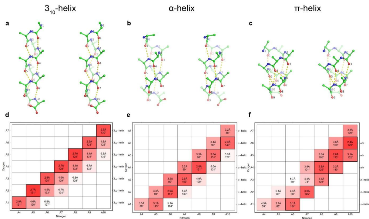
Figure 3.2.6. Analysis of the hydrogen bonds of the “ideal geometry” polyalanine 3 10 -, α- and π-helices. a,b,c) Cross-eyed stereographic images of the helix F and the residues stabilizing the secondary structure. d,e,f) Distances between the backbone O and N atoms and the angles between the C=O and O···H bonds, separated by 3, 4 and 5 residues. The cells corresponding to the putative hydrogen bonds are emphasized. The assigned secondary structure is listed at the right side of the table. The atomic coordinates were taken from Justin Lorieau website ( http://www.lorieau.com/methods-and-reference/biophysics-and-biochemistry/9-model-protein-helix-structures ) and are based on the data obtained from the high-resolution crystallographic structures 227 . The average values for the i→i+3, i→i+4 and i→i+5 bonds and angles are 2.78 Å, 4.51 Å, and 6.78 Å and 126°, 131° and 131°.
