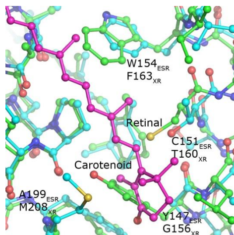
Figure 3.2.8. Comparison of the XR carotenoid-binding site with the same region of ESR. ESR is shown in green, XR in blue and the carotenoid salinixanthin in magenta. This binding mode of the carotenoid is impossible in ESR. Most importantly, there is a direct access to the retinal \beta -ionone ring in XR that is made possible by Gly-156. In ESR the retinal is covered by the bulky Tyr-147. Other notable residues with larger sizes are Trp-154 of ESR (compared to Phe-163 of XR) and Cys-151 of ESR (compared to Thr-160 of XR). Also, in the XR structure the carotenoid interacts with Met-208, which is mutated to alanine in ESR.
