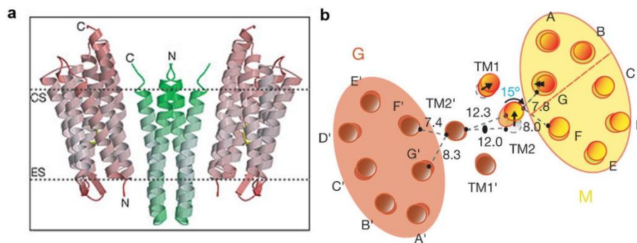
Figure 1.2.7. Structure of the sensory rhodopsin-transducer complex and conformational changes during the photocycle. a) Structure of 2:2 NpSRII:NpHtrII complex in the membrane 125 .
