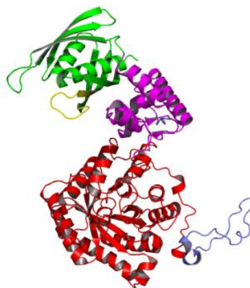
Figure 1.13: Representation of the monomer 2-isopropylmalate synthase. Green: regulatory domain; Magenta: linker; Red: catalytic domain.; Yellow: the flexible loop involved in the onset-step inhibition (PDB 3FIG).
