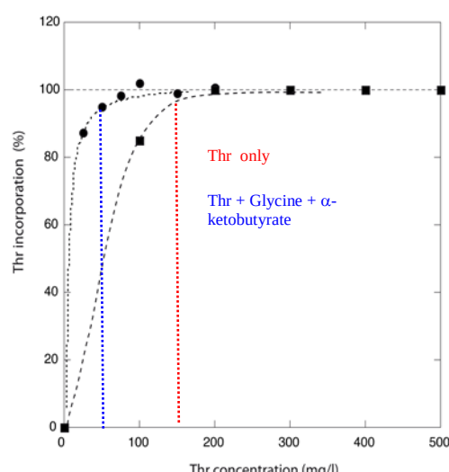
Figure 1.19: Optimization of the incorporation of Thr [\alpha,\beta\text{-}^2\text{H}, \gamma_2\text{-}^{13}\text{C}^1\text{H}_3] -L-Thr. The Threonine curve incorporation was performed using [U\text{-}^2\text{H}] ubiquitin. Met was used as internal reference for the quantification of Thr incorporation.
