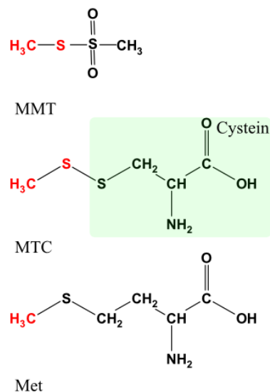
Figure 1.23: Introduction of an artificially labeled methyl groups through the MMTS molecule. MMT: methylsulfonylsulfanylmethane, MTC: (S)-methylthiocysteine, Met: Methionine. The labeled methyl group is highlighted in red.
