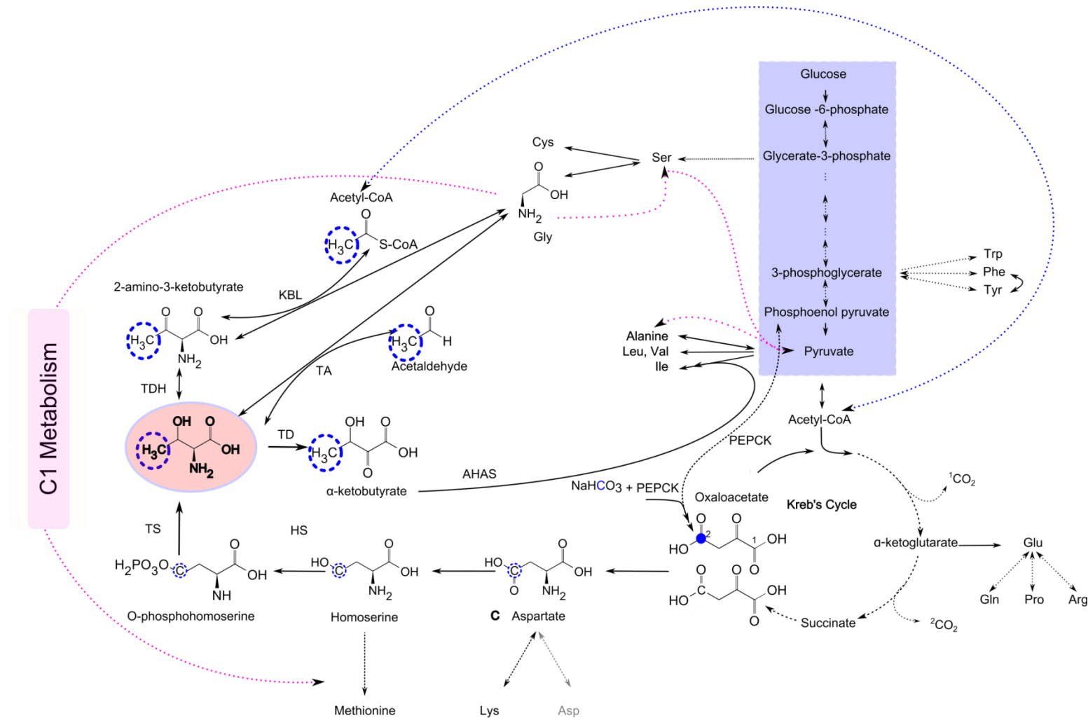
Figure 1.17: E. coli metabolic pathways for Threonine biosynthesis and degradation. Arrows depicted in pink represent reactions through which 13 C scrambling, via glycine, is obtained when U- 13 C- Thr is used. Carbons highlighted in blue represent a parallel pathway of the Thr methyl group origin (Sinha et. al, 2011). The carbons surrounded with dashed blue circles represent atoms that can be either from the TCA oxaloacetate or from phosphoenolpyruvate. The 1, 2 numbers in oxaloacetate molecule indicate the carbon atoms that are lost in the TCA. Enzyme abbreviation: TD:Threonine Deaminase; CP:Pyruvate Carboxylase; HS: Homoserine Kinase; TS: Threonine Synthase; TD: Threonine Deaminase; AHAS: Aceto-hydroxy-acid synthase; TDH: Threonine Deshydrogenase; TA: Threonine Aldolase; KBL: 2-amino-3-ketobutyrate ligase. Dashed arrows represent multi-steps reactions
