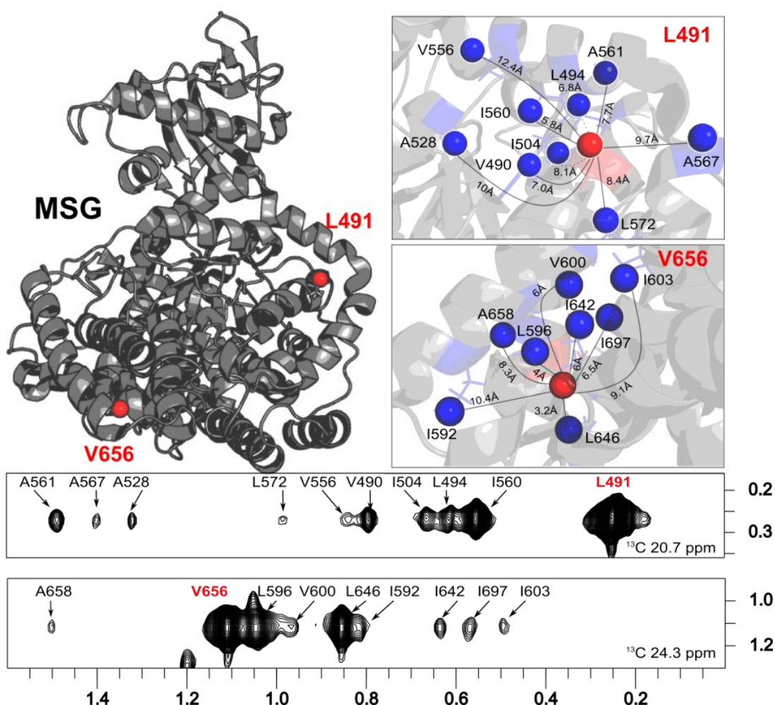
Figure 8: Detection of long-range nOes in the [U-D], A-[ ^{13}\text{CH}_3 ] ^\beta , I-[ ^{13}\text{CH}_3 ] ^{\delta 1} , (LV)-[ ^{13}\text{CH}_3 ] ^{\text{proS}} -MSG sample (82 kDa). 2D extracts of the 3D ^{13}\text{C} -HMQC-NOESY spectrum are presented along with the extracted distances between each pair of methyl groups from the 3D structure of MSG (1D8C). The experiment was acquired on a 800 MHz spectrometer equipped with a cryoprobe at 37°C for 3.5 days with recycling delay d_1 = 1.3 s and NOE mixing time \tau_m = 500 ms. The [ U\text{-}^2\text{H} , A^{\beta 1\delta 1} ](LV) ^{\text{proS}} ]-MSG sample was at 1 mM in a ^2\text{H}_2\text{O} buffer containing 20 mM MES, pH 7.1, and 25 mM \text{MgCl}_2 . Diagonal peaks are highlighted in red.
