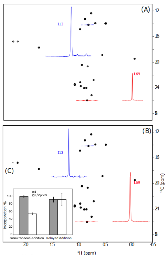
Figure 1: The co-incorporation of I \delta^1 and (LV) ^{\text{proS}} precursors in a ubiquitin sample: 2D HSQC NMR spectra were recorded at 37°C in ^2\text{H}_2\text{O} buffer (20 mM Tris, pH 7.4, and 20 mM NaCl) on a 800 MHz NMR spectrometer equipped with a cryogenic probe. The [ U\text{-}^2\text{H} ], A- ^{13}\text{CH}_3 ] ^\beta , I- ^{13}\text{CH}_3 ] ^\delta -ubiquitin sample was prepared using 2- ^{13}\text{CH}_3 , 4- ^{13}\text{H}_3 ] acetolactate and 3,3- ^{13}\text{H}_2 , 4- ^{13}\text{C} -2-ketobutyrate. A) Both precursors were added simultaneously to the culture 1 hour before induction (3 h). B) Labeled acetolactate was added to the culture 1 hour before induction (3 h), while the labeled 2-ketobutyrate was added 20 minutes before induction. C) Quantification of the I- \delta^1 and (LV)-pro-S signals in both cases using the Met- \epsilon methyl groups were used as an internal reference. The experimental I- \delta^1 /Met- \epsilon and LV-pro-S/Met- \epsilon ratios were compared to those obtained for conditions with complete incorporation of each precursor.
