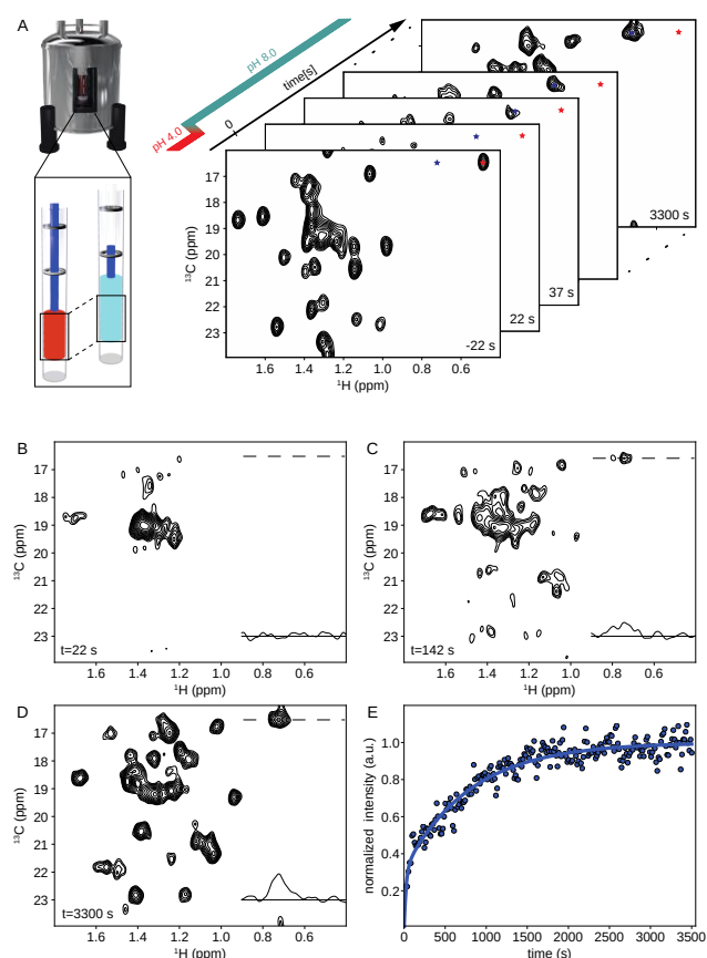
Fig. 1. Real-time kinetic NMR and progress of TET2 self-assembly. (A) In situ stopped flow pH jump and real-time NMR spectra acquisition (see supplementary information). (B) Ala ^\beta - ^{13}\text{CH}_3 TET2 spectrum after assembly initiation upon basic pH jump. (C) Ala ^\beta - ^{13}\text{CH}_3 TET2 intermediate spectrum. (D) Spectrum of the reassembled TET2. Traces in NMR spectra show 1D projection of A192. (E) Build of the non-overlapping peak intensity evolution (blue dots) with fit of double exponential (solid line).
