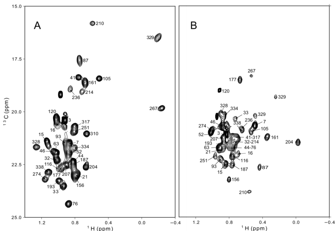
Figure 2.2: Comparison of 2D [U- ^2\text{H} , ^{13}\text{CH}_3\text{-Val}^{\text{proS}} ]-PhTET-2 and [U- ^2\text{H} , ^{13}\text{CH}_3\text{-Val}^{\text{proR}} ]-PhTET-2 NMR spectra. From Mas, Crublet et al., 2013.
