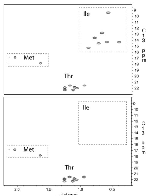
Figure 1.19: : [^1\text{H}, ^{13}\text{C}] HSQC spectra of [U\text{-}^2\text{H}, \text{Thr-C}\gamma_2] human ubiquitin. Ubiquitin was produced using (A) [\alpha,\beta\text{-}^2\text{H}, \gamma_2\text{-}^{13}\text{C}^1\text{H}_3] -L-Thr (50 mg/L) + Met (100mg/L) and (B) [\alpha,\beta\text{-}^2\text{H}, \gamma_2\text{-}^{13}\text{C}^1\text{H}_3] -L-Thr (50 mg/L) + [U\text{-}^2\text{H}]\text{-}\alpha -ketobutyrate (100 mg/L) + [U\text{-}^2\text{H}]\text{-glycine} (500mg/L) + Met (100mg/L). Met was used as an internal reference for the quantification of Thr incorporation.
