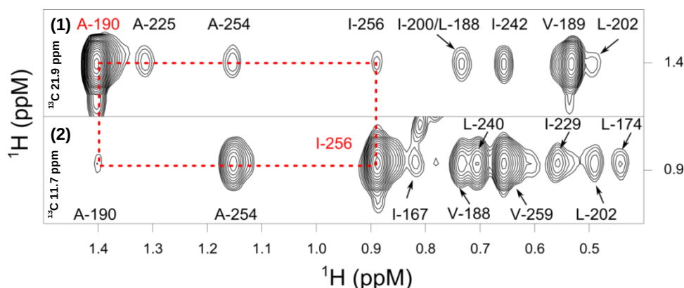
Figure 4.2.3: Detection of long-range nOes in a [\text{U-}^2\text{H}, \text{Al}^{\delta 1}(\text{LV})^{\text{proS}}]\text{-MSG} sample (82 kDa). 2D strip plot of 3D ^{13}\text{C} -HMQC-NOESY spectrum. The extracted distances from the MSG crystallographic structure (1D8C) between each pair of methyl groups are: (1) 190-225 : 7.6 Å; 190-254 : 6.8 Å; 190-256 : 9.8 Å; 190-200 : 10 Å; 190-188 : 8.9 Å; 190-189 : 3.6 Å; 190-202 : 8.8 Å. (2) 256-174 : 8 Å; 256-229 : 9.6 Å; 256-259 : 3.5 Å; 256-240 : 5 Å; 256-188 : 6.3 Å; 256-167 : 8 Å; 256-254 : 3.4. The experiment was acquired at 37°C on a 800 MHz spectrometer equipped with a cryoprobe for 3.5 days with d_1 = 1.3 s and \tau_m = 500 ms. The [\text{U-}^2\text{H}, \text{Al}^{\delta 1}(\text{LV})^{\text{proS}}]\text{-MSG} sample was at 1 mM concentration in 20 mM MES, 25 mM \text{MgCl}_2 pH 7.1 ^2\text{H}_2\text{O} buffer. Diagonal peaks are highlighted in red.
