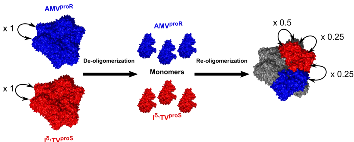
Figure 4.3.2: Scheme representing the sample preparation for the filtering of inter-monomeric nOes. In red, PhTET-2 is [ U\text{-}^2\text{H} , I^{\delta 1}\text{V}^{\text{proS}} T] labeled and in blue, the protein is [ U\text{-}^2\text{H} , \text{MAV}^{\text{proR}} ] labeled. The probability of the occurrence of each type of inter-monomeric nOe (from equivalently or differentially labeled monomers) in the native and reoligomerized particles is indicated.
