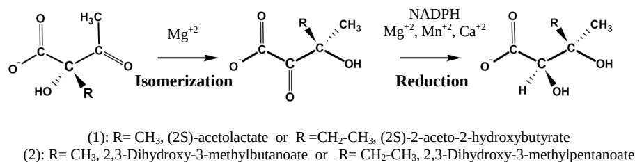
Figure 1.9: Scheme of Ketol-acid reductoisomerase reaction catalysis.
