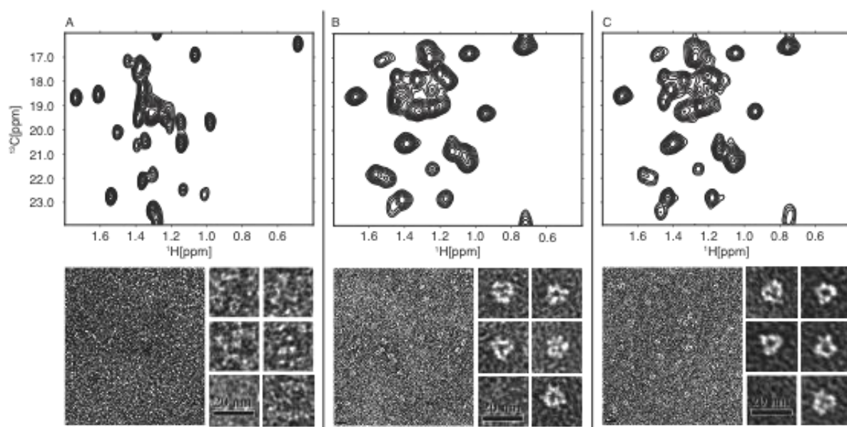
fig. S1. TET2 Ala \beta -[ ^{13}\text{CH}_3 ] HMQC spectrum and EM projection of (A) diassembled monomer, (B) resassembled dodecamer, and (C) native dodecamer.
