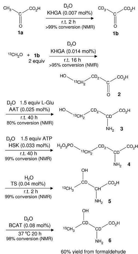
Figure 1.16: Scheme representing the enzymatic biosynthesis of U\text{-}[^2\text{H}],\text{Thr-}\gamma_2\text{-}^{13}\text{CH}_3 . 1a. pyruvate. 1b. [\text{U-}^2\text{H}]\text{-pyruvate} . 2. 2-keto-4-hydroxybutyrate. 3. Homoserine. 4. O-phospho-L-homoserine. 5-6 Threonine. Enzyme name abbreviations: 2-keto-4-hydroxyglutarate aldolase (KHGA), aspartate aminotransferase (AAT), homoserine Kinase (HSK), threonine synthase (TS), branched-chain-amino-acid Aminotransferase (BCAT). From (Velyvis, Ruschak et al. 2012)
