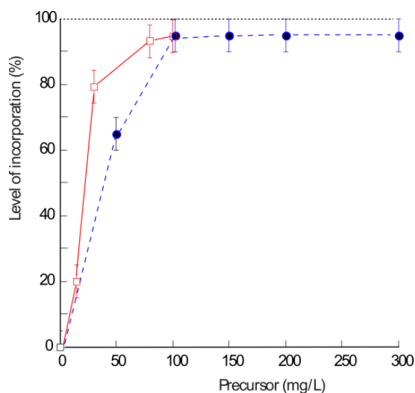
Figure 6. Incorporation level of the chemically and enzymatically synthesized precursors in overexpressed ubiquitin as a function of the amount of exogenous labeled precursor added.
