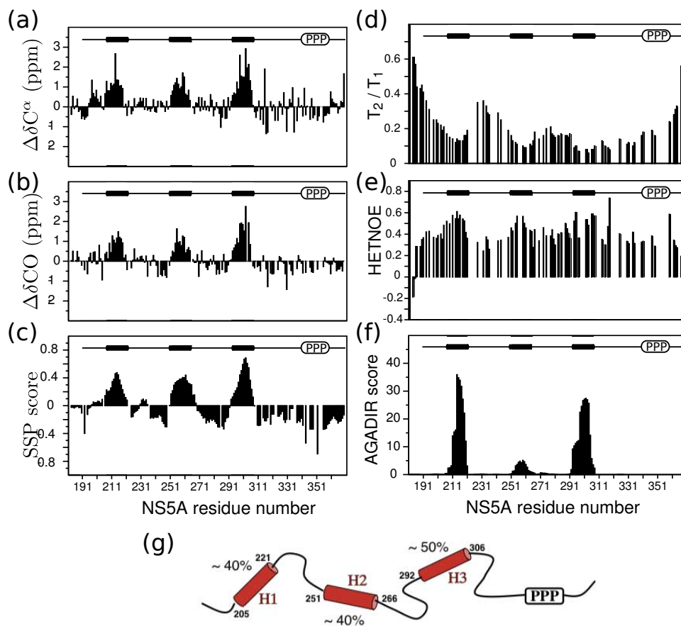
Figure 8.6: “Structural and dynamic characterization of NS5A(191369) (D2) at 5 °C from NMR chemical shift, and ^{15}\text{N} relaxation data. (a) \text{C}^\alpha and (b) CO secondary chemical shifts calculated as the difference between measured and random-coil chemical shifts from the refDB database [60] and corrected for next-neighbor effects [64]. (c) Structural propensities calculated with the SSP program [146]. All available chemical shifts (HN, N, \text{C}^\alpha , \text{C}^\beta , and CO) have been used as input data for the SSP calculation. Positive score values indicate the amount of \alpha -helical conformation present along the sequence, while negative values are indicative of extended or \beta -strand conformations. (d) Ratios of measured transverse and longitudinal ^{15}\text{N} relaxation times ( T_2/T_1 ) providing an estimate of the local rotational correlation times \tau_c along the peptide chain. (e) \{^1\text{H}\}^{15}\text{N} NOE (HETNOE) values indicative of the amplitude (order parameter) of local subnanosecond motions (high values: restricted motion, low values: high-amplitude motions). (f) Prediction of helical propensities based on the physical chemistry of the polypeptide chain using the program AGADIR [145]. (g) Structural model derived from the recorded NMR data showing three \alpha -helical segments of similar length that are formed with propensities of \sim 40\% for H1 and H2 and \sim 50\% for H3, connected by flexible linker regions.” As published in Ref. [112].
