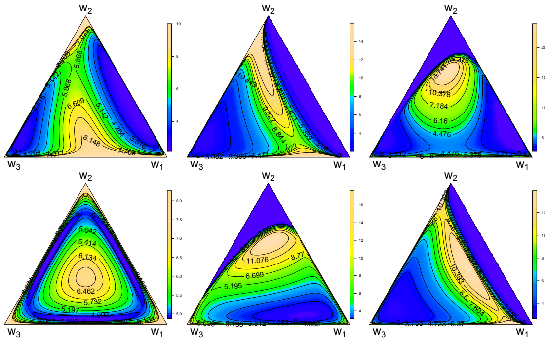
Figure 4.4: Trivariate extremal skew- t angular densities with \nu = 2 degrees of freedom. Correlation coefficients are \omega = (0.52, 0.71, 0.52)^\top for the top row and \omega = (0.95, 0.95, 0.95)^\top for the bottom. Left and centre columns respectively have skewness \alpha = (0, 0, 0)^\top and \alpha = (-2, -2, 5)^\top . Right column has \alpha = (-10, 5, 1)^\top (top) and \alpha = (-2, -2, -2)^\top (bottom). In all cases \tau = 0 for simplicity.
