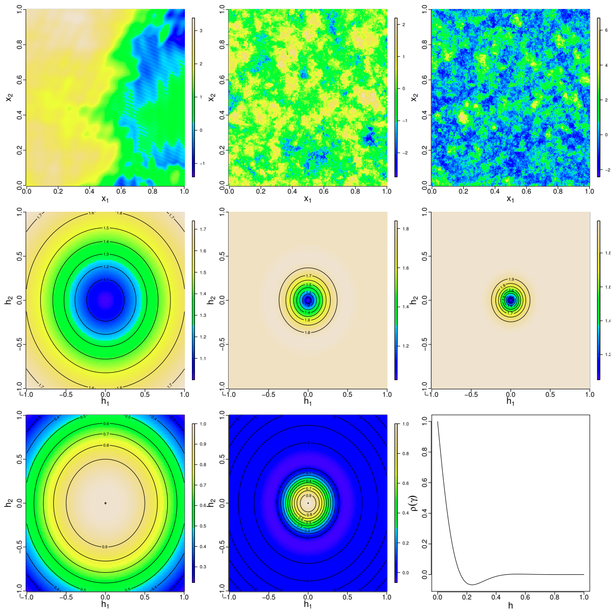
Figure 2.4: Representation of Extremal- t processes on \mathbb{S} = [0, 1]^2 . The top row represents some realizations of the process while the second and third row shows respectively the extremal coefficient and the correlation function. The first column considers a Whittle-Matérn correlation function \rho(h) with smoothness parameter 0.8 and degree of freedom \nu = 2 . The second and third column display the process with degrees of freedom respectively \nu = 2 and 8 and the same damped cosine correlation function \rho(h) with scale \lambda = 0.1 and smoothness 1. The middle and right panels of the bottom row respectively provide the two and one-dimensional representations of the isotropic correlation function. The margins are transformed to be Gumbel.
