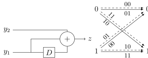
Figure 2.3: Syndrome former and one trellis section for the convolutional code with generator matrix [1, 1 + D] : dashed lines correspond to z = 0 and solid line to z = 1 .
