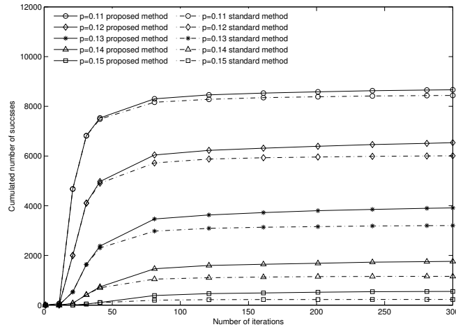
Figure 3.3: Comparison between the standard and the proposed method using a rate-0.1 LDPC code, the rate-1/2 convolutional code (5,7) and the Viterbi algorithm to perform the projection: Cumulated number of decoding successes as a function of the number of iterations.
