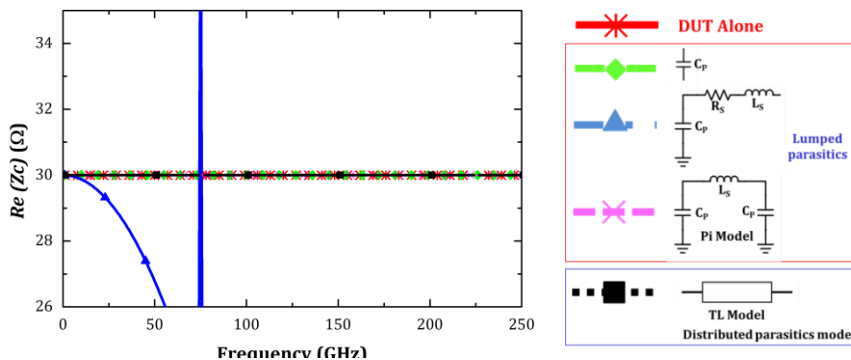
Figure 2.25. Characteristic Impedance of the DUT – Hernandez Method
