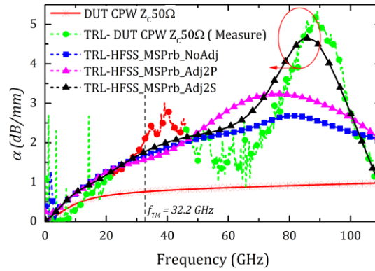
Figure 4.26. Attenuation coefficient of DUT CPW Z_c=50 \Omega : Measure vs HFSS Model with MSprobe
