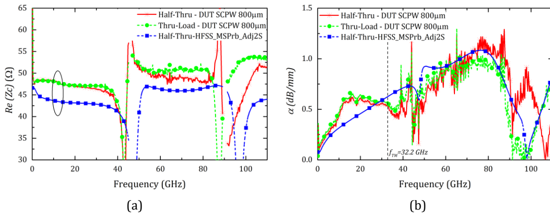
Figure 4.28. Half-Thru and Thru-Load de-embedding: DUT SCPW 800 μm, Z_c=50 \Omega (a) Characteristic Impedance (b) Attenuation coefficient
