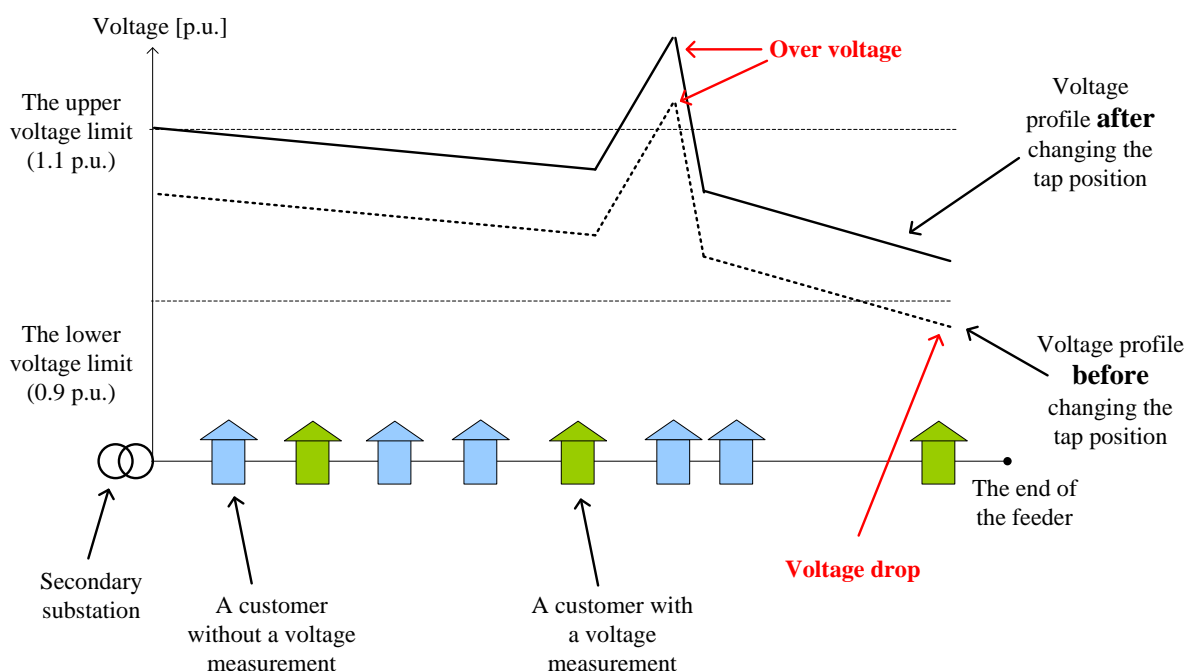
Figure 55: Voltage profile of a feeder before and after a change in a tap position by the on-load tap changer. Three of eight customers are equipped by a voltage measurement in order to control the on-load tap changer. Before the change in the tap position, the last (the rightmost) customer experiences a voltage drop. After the tap change, the sixth customer (from the left) experiences an over voltage because it is not equipped by a voltage measurement. The purpose of the figure is to support the idea presented in the text and not to be exactly realistic.
