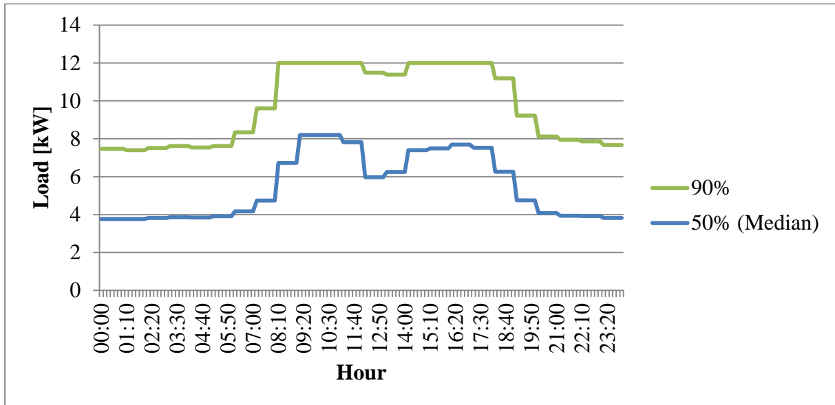
Figure 33: The curves of the 90 th (the green curve) and the 50 th (the blue curve) percentile of a single-phase customer during a winter working day. These curves are given as an input to the algorithm that creates a new load curve. The new load curve is illustrated in Figure 34.
