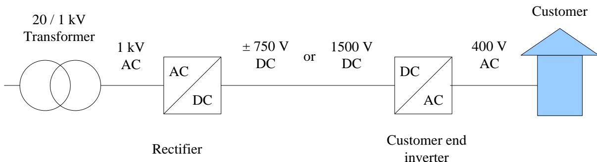
Figure 16: The principal components of an LVDC connection [159].
