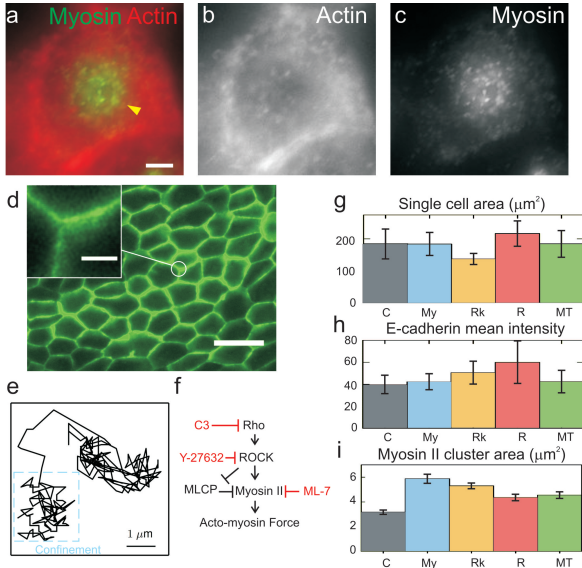
FIG. 1. (Color online) Study of vertex fluctuations. (a) Actin (red) and myosin (green) structures at the apical surface of a MDCK cell (scale bar 3 \mu\text{m} ). The myosin is concentrated in dense contractile units (yellow arrow) referred to as myosin clusters. (b) Actin structure alone. (c) Myosin structure alone. (d) We visualise MDCK cell monolayer by GFP E-cadherin (scale bar 30 \mu\text{m} ). (Inset) We identify the meeting points between three cells as the privileged point for our analysis (scale bar 4 \mu\text{m} ). (e) Extraction of a typical transition between two locally stable positions in the vertex trajectory (total time 8 hours). (f) Simplified diagram of the Rho pathway installing a order relation in myosin activation; in red the specific inhibitors and their targets. (g) Area of individual cells in each condition. C: Control; My: Myosin inhibitor; Rk: Rho kinase (ROCK) inhibitor; R: Rho inhibitor; MT: Depolymerised microtubules. (h) Mean GFP E-cadherin intensity of individual cell-cell contacts. (i) Area of myosin clusters [24].
