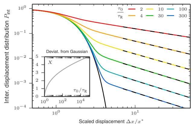
FIG. 2. Distribution of small displacement scaled by x^*(t) = \sigma\sqrt{2f_t/(1 - \tau_R/\tau_0)} in Eq. (18). The central part is Gaussian (solid black line) with power-law tails (dashed lines). (Inset) Crossover value X between the central Gaussian part and the tails of the distribution as a function of \tau_0/\tau_R .
