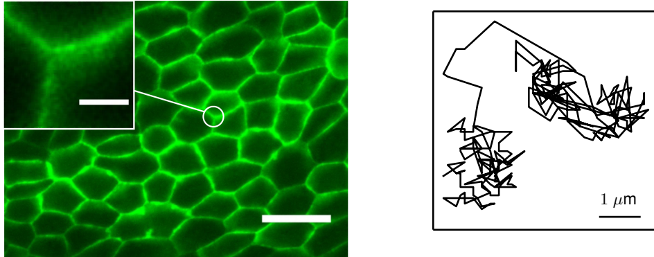
Figure 6.2 – Left: MDCK cell monolayer visualized by GFP E-cadherin. Scalebar 30 \mu\text{m} . (Inset) Tricellular junction named as vertex. Scalebar 4 \mu\text{m} . Right: Typical trajectory of a vertex. Time between two successive measurements 5 \text{ min} . Taken from paper E .
