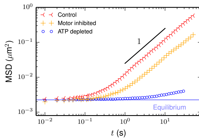
Figure 4.1 – Top: Typical trajectories of colloidal tracers in living melanoma cells under three conditions: ATP depleted cells, blebbistatin treated cells for which the activity of myosin-II motors is inhibited, and untreated cells as a control. Bottom: Mean square displacement as a function of time for the three conditions. Taken from paper B.
