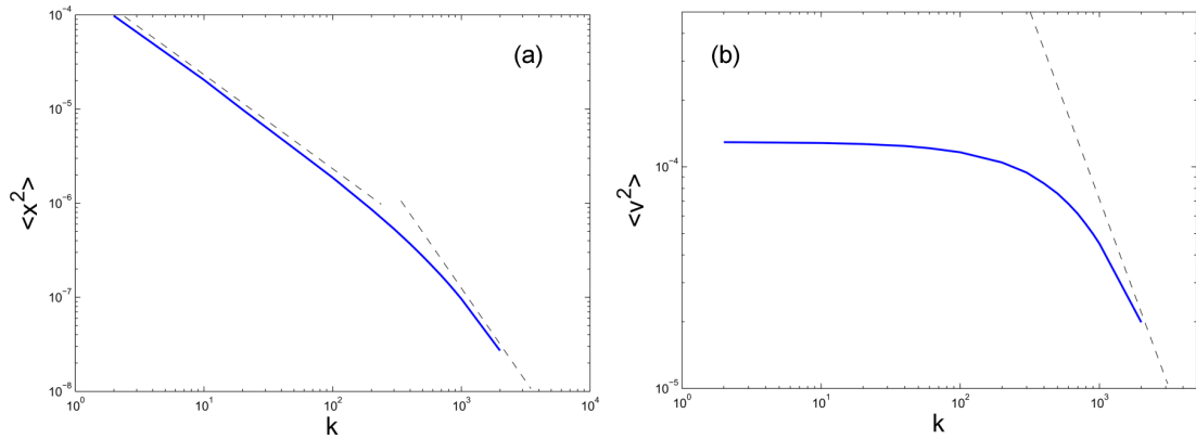
FIG. 4. (Color online) Simulated mean-square particle displacements (a) and velocity (b) in the limit of \lambda \Delta \tau \gg 1 , using \Delta \tau = 1 , \lambda = 50 , f_0 = 1 , p_{on} = 0.1 . The dashed lines indicate the power laws with exponents -1 , -2 in (a) and -3/2 in (b).
