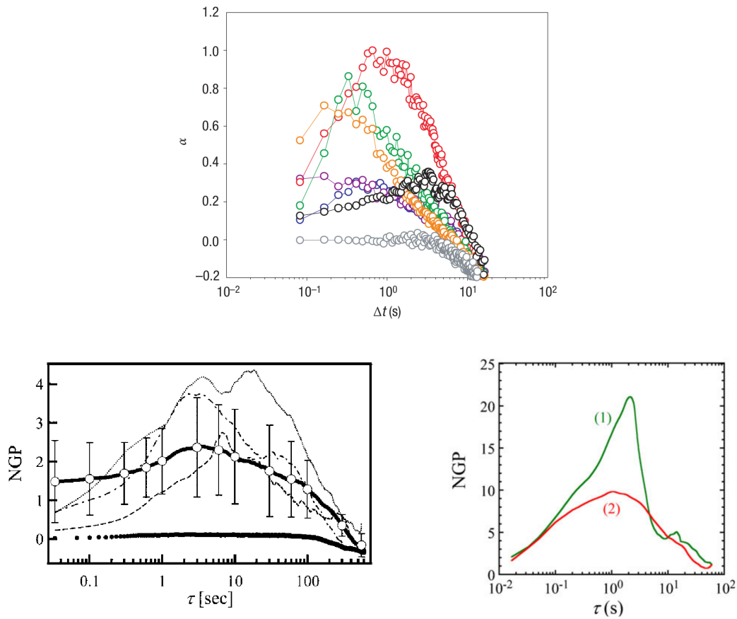
Figure 2.6 – Typical measurements of the non-Gaussian parameters defined in Eq. (2.1). Up: Beads attached to the cell cortex. Taken from [53]. Bottom left: Beads injected in an acto-myosin gel. Taken from [42]. Bottom right: Beads injected in living cells. Taken from [8].
