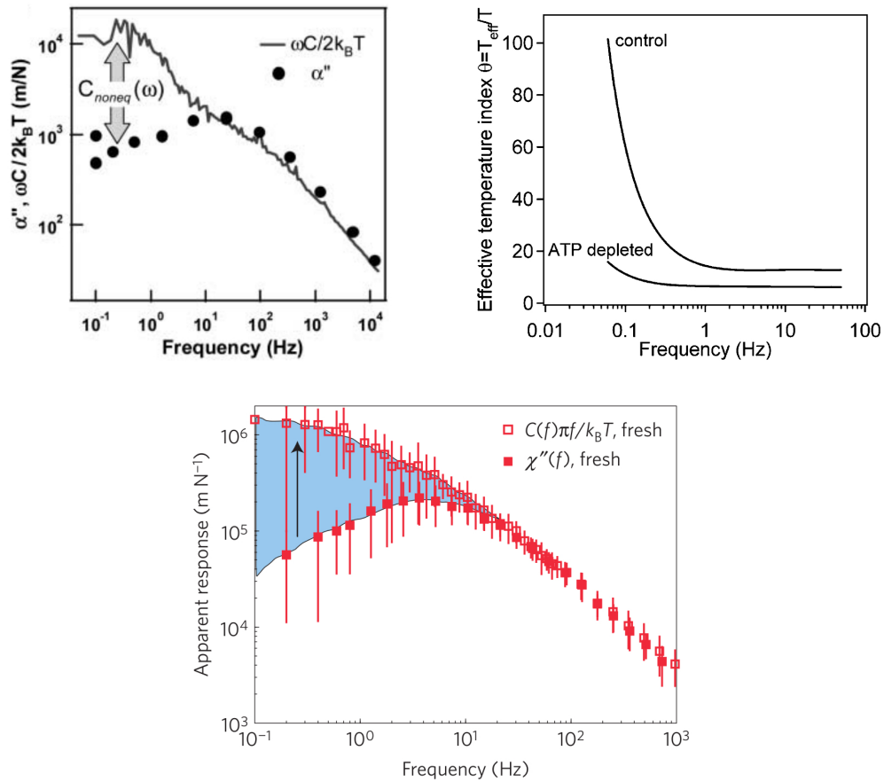
Figure 2.7 – Experimental measurements of the FDT violation. Upper left: Comparison between spontaneous fluctuations and response for beads injected in acto-myosin gel. Taken from [74]. Upper right: Effective temperature extracted from response and fluctuations of tracers attached the membrane of living cells. Taken from [54]. Bottom: Comparison between spontaneous fluctuations and response for the membrane of red blood cells. Taken from [64].
