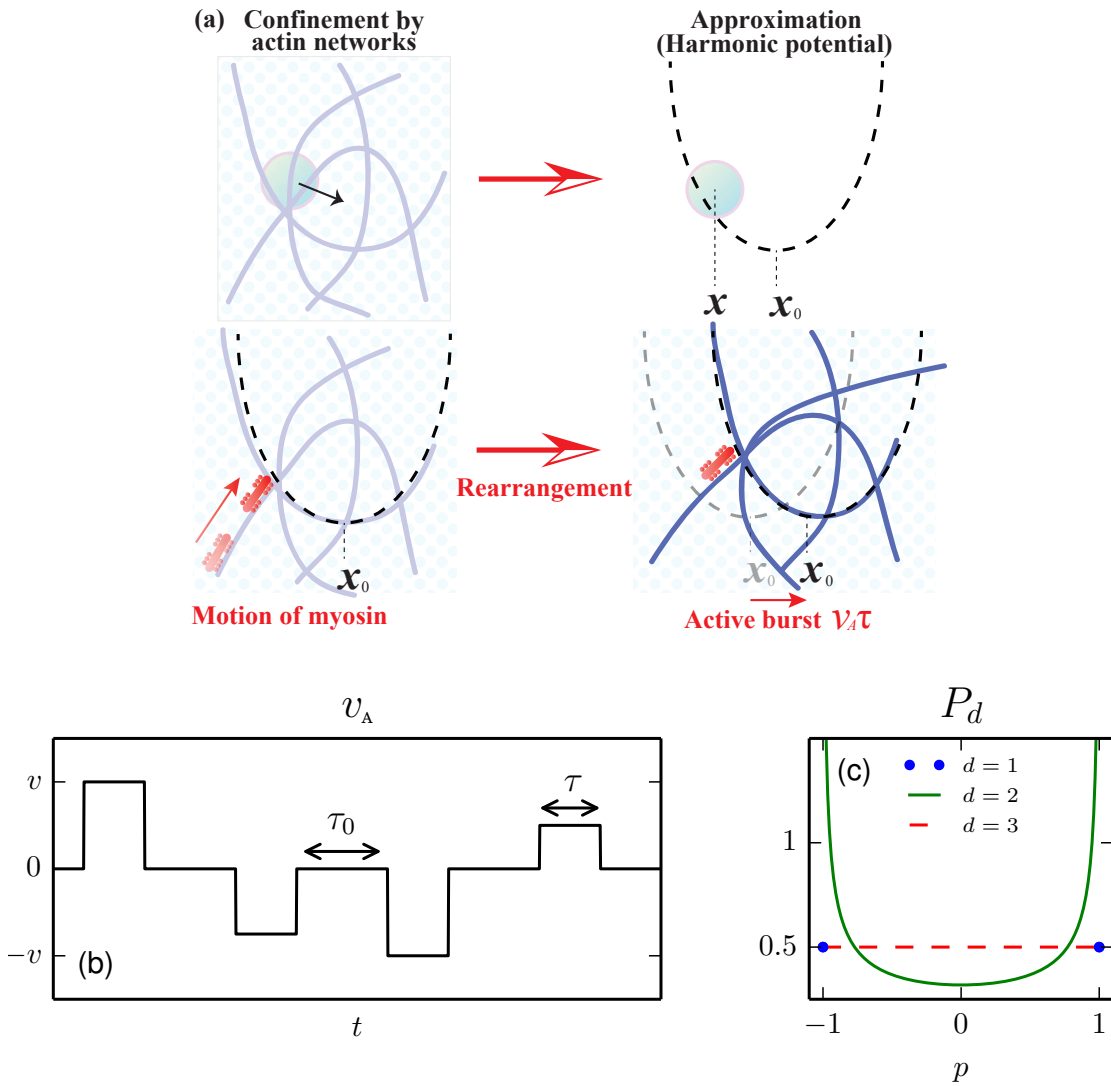
Figure 3.1 – (a) Schematic representation of the network remodelling induced by motor activity. (b) Typical realization of the active burst. (c) Distribution P_d of the one-dimensional projection p of a random direction in d dimensions for d = \{1, 2, 3\} in dot blue, green solid, and red dashed line, respectively. Taken from paper A .
