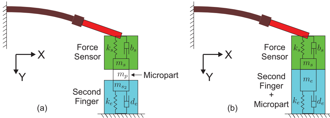
FIGURE 3.17: The equivalent scheme of microgripper manipulating a rigid micropart: (a) the mass of finger ( m_{s_2} ) is separated of the mass of the micropart ( m_p ) and (b) the mass of the finger is combined with the mass of the micropart ( m_e = m_{s_2} + m_p ).
