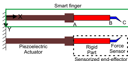
FIGURE 3.3: Complete scheme of the two-smart-fingers microgripper (TSFM).
