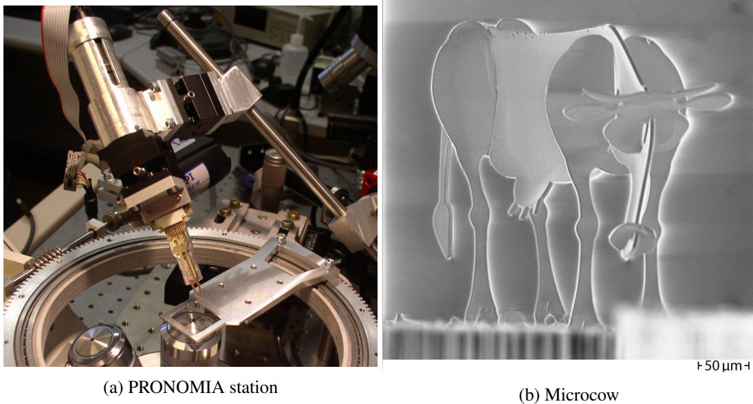
FIGURE 1.13: PRONOMIA microassembly station [62] and the assembled microcow.
