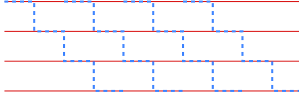
Figure 6.1: The 4 \times 4 skewed grid, with horizontal (red) and vertical paths (thick dashed blue) in the proof of Lemma 6.4.14
