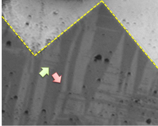
Figure 1.22: Cross polarized optical image of ferroelectric domains in a BiFeO_3 crystal. Yellow dash line indicates the edge of a gold electrode. Green and red arrows show the possible in-plane orientation of the polarization in two adjacent domains which leads to an observable optical contrast.
