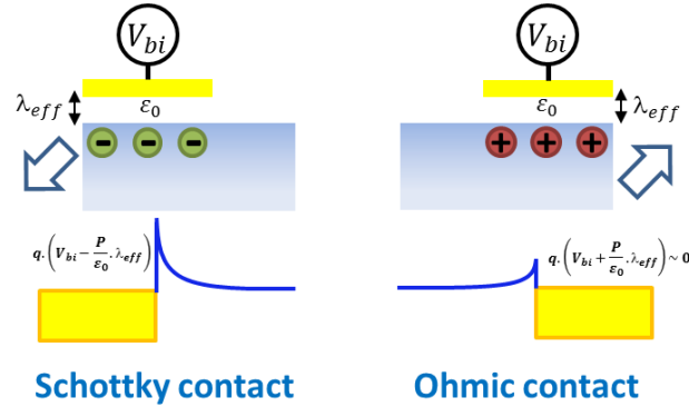
Figure 2.21: Imperfect screening at the Au/BiFeO_3 interface. Depending on the orientation of the polarization under the electrode, the contact can be Schottky or Ohmic.
