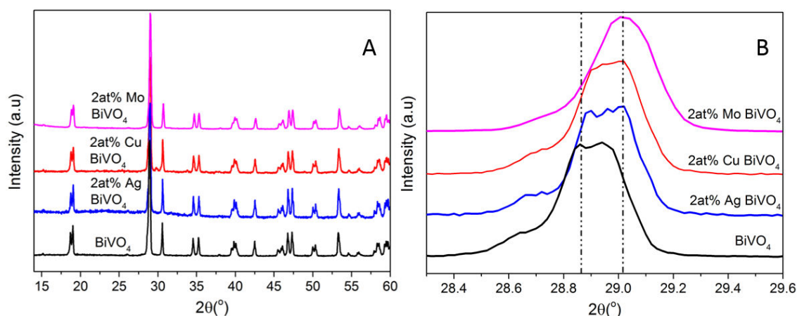
Fig.4.1. (A) XRD pattern of pristine and M-BiVO 4 (M - Mo, Cu and Ag) synthesized by sol-gel method in comparison with diffraction pattern of JCPDS No-14-0688. (B) The characteristic peak shift to higher 2θ angle.
