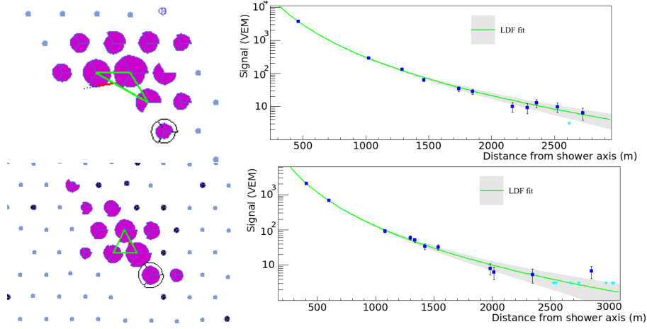
Figure 5.3: Two examples of 4T5 events. Event 201130905216 (top) fell at the border of the array, while event 201017300252 (bottom) fell in an area where a few stations were inactive.
