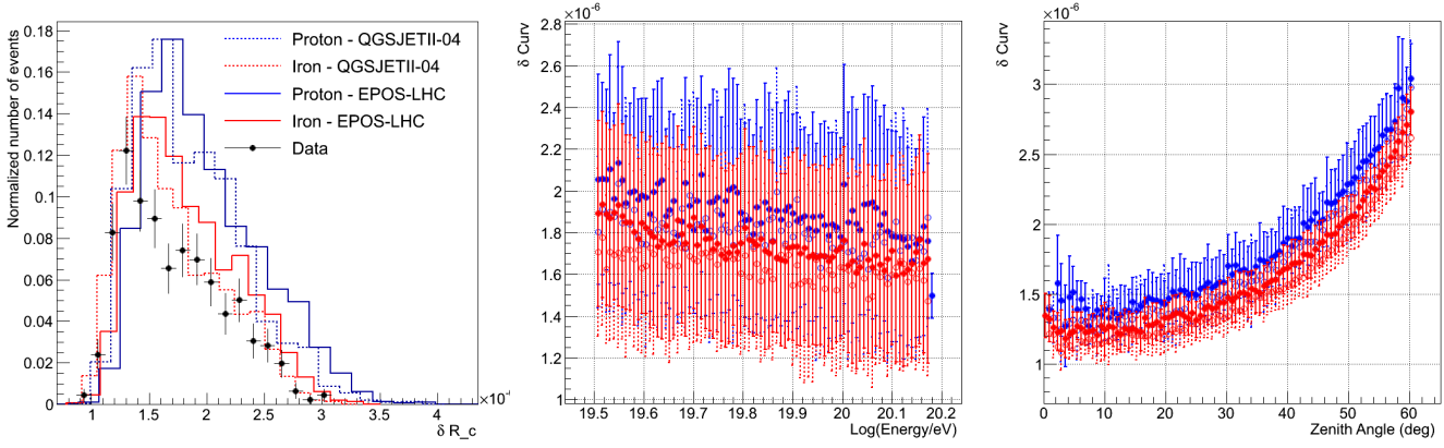
Figure 7.3: Left: distribution of \delta R_c (see text) for simulated events with E > 32 EeV (histograms) and data (dots). Center and right: its dependency on energy and zenith angle, respectively.
