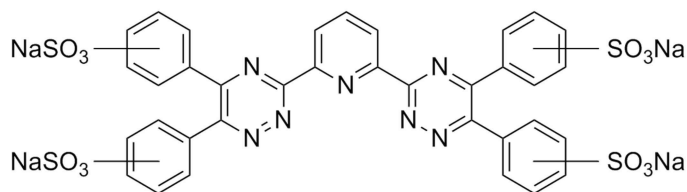
Figure 15 : 2,6-bis(5,6-di(sulfophenyl)-1,2,4-triazin-3-yl)pyridine ( SO_3 -Ph-BTP)
