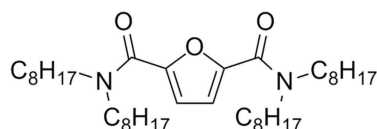
Furane-TODGA
