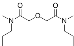
DMDnPDGA (N,N'-diméthyl-N,N'-dipropyl-diglycolamide)
