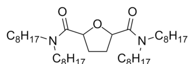
THF-TODGA
