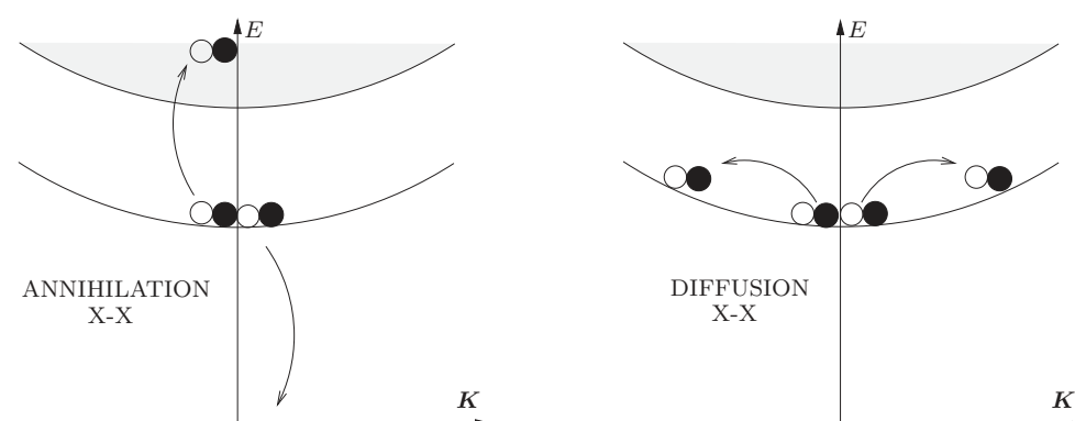
FIGURE 1.29 – interactions exciton-exciton
