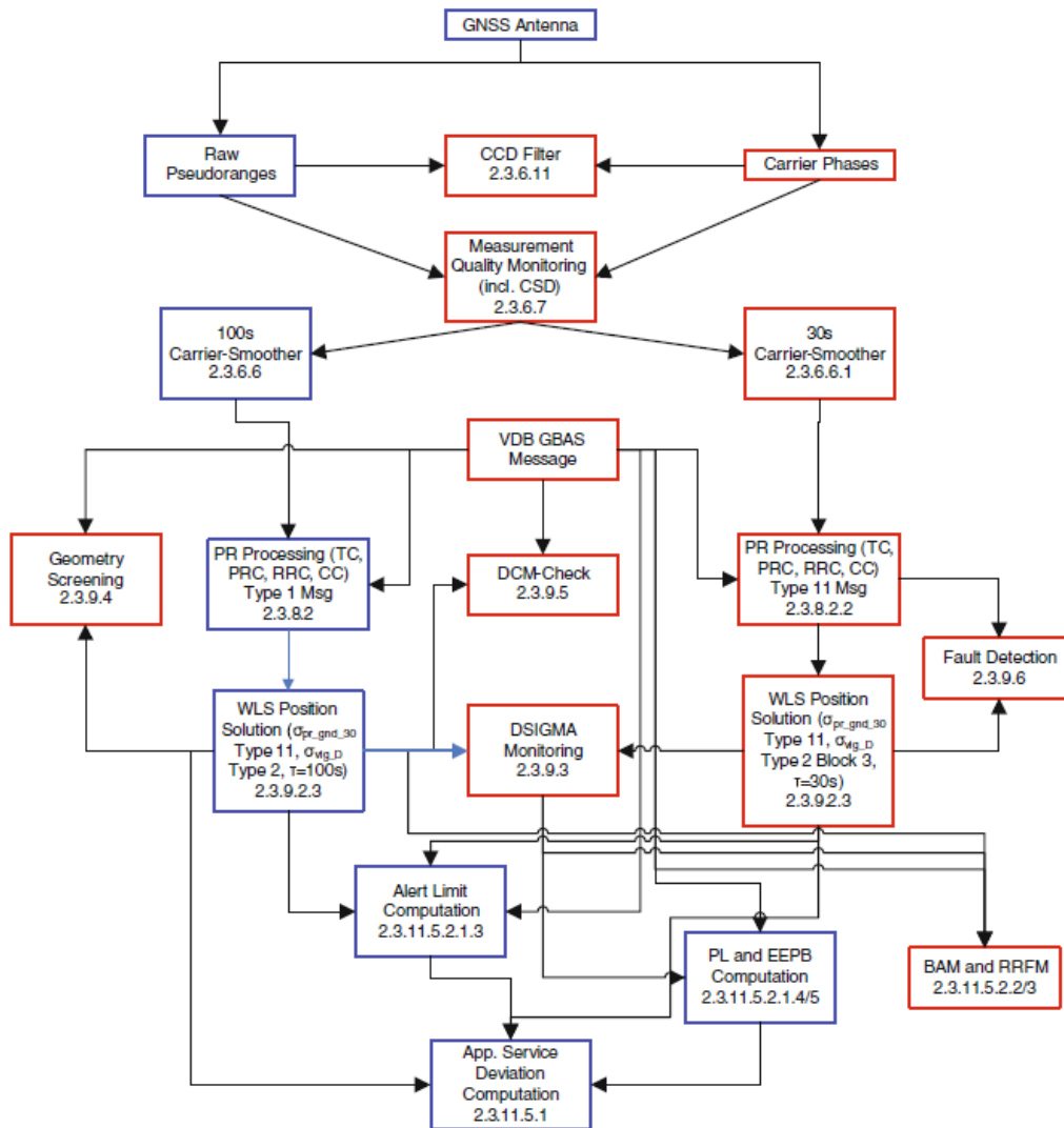
Figure 33-GAST D Aircraft Architecture [16]
