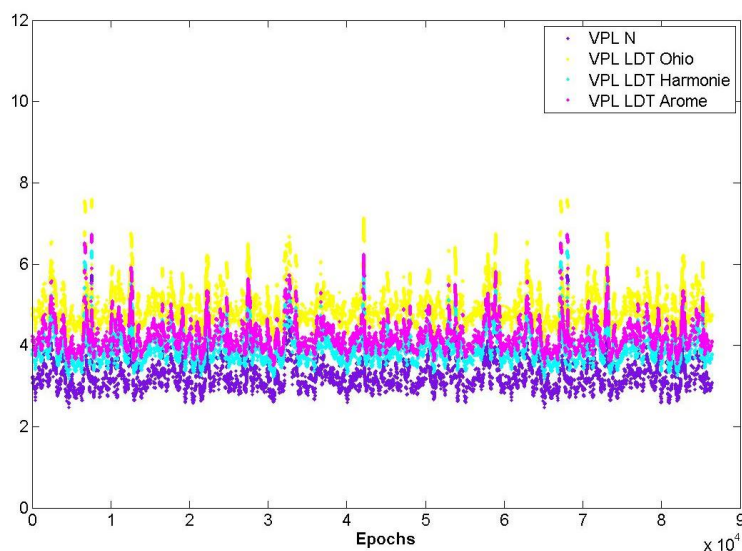
Figure 127-VPLs for GPS and GAL constellations
