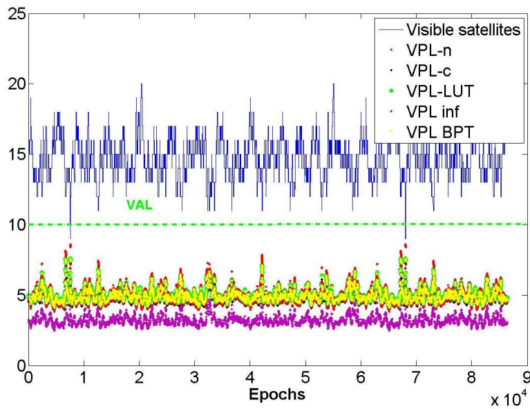
Figure 143-VPLs Seattle Dth=5km, GPS and GAL N=12
