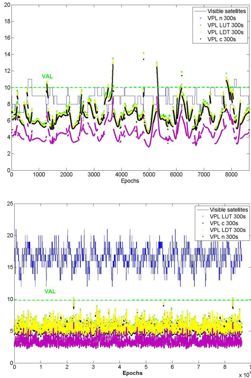
Figure 186-VPLs IF Anchorage 300s , GPS (left) and GPS and GAL (right), Dth10km
