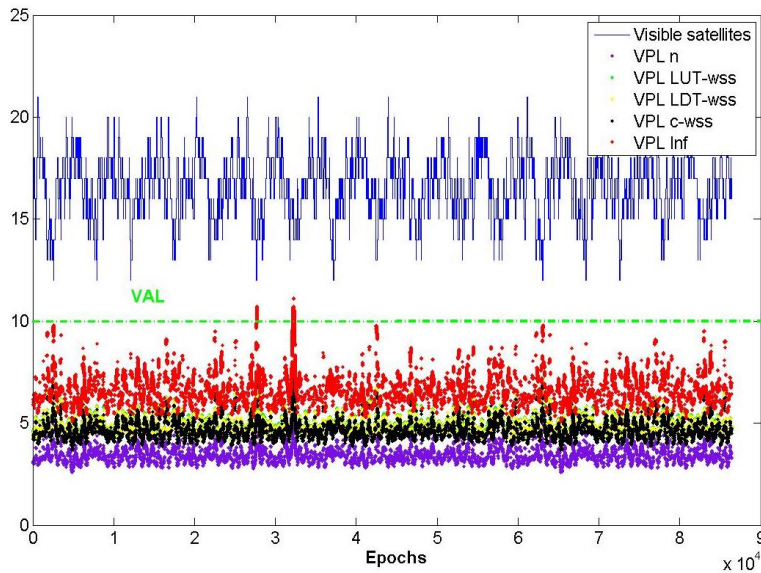
Figure 161-VPLs Anchorage geometry improved GPS (left) and the GPS and GAL (right), Dth=5km
