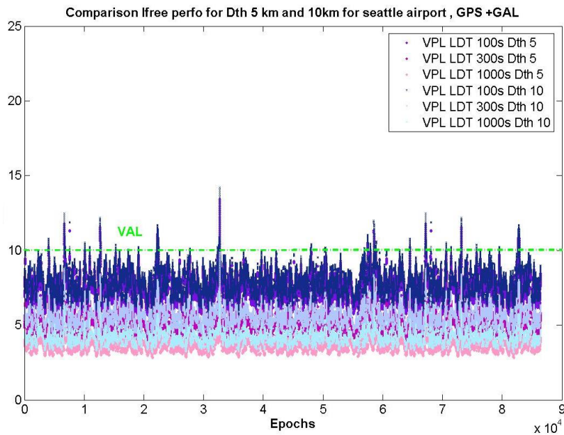
Figure 169-Comparison VPLs IF performance for Seattle
