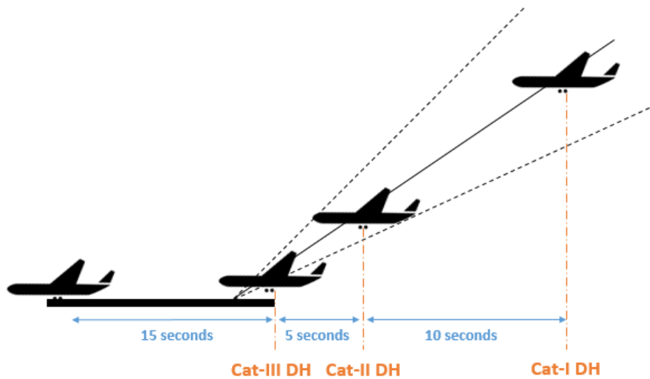
Figure 4-ILS Look-Alike Method
