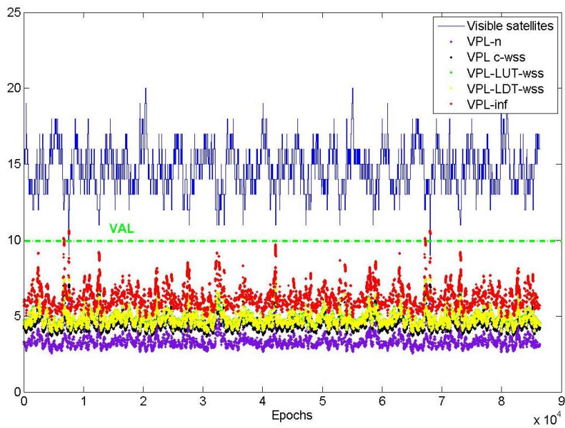
Figure 151-VPLs with WSS methodology for Seattle, GPS (left) and the GPS and GAL (right), Dth=10km
