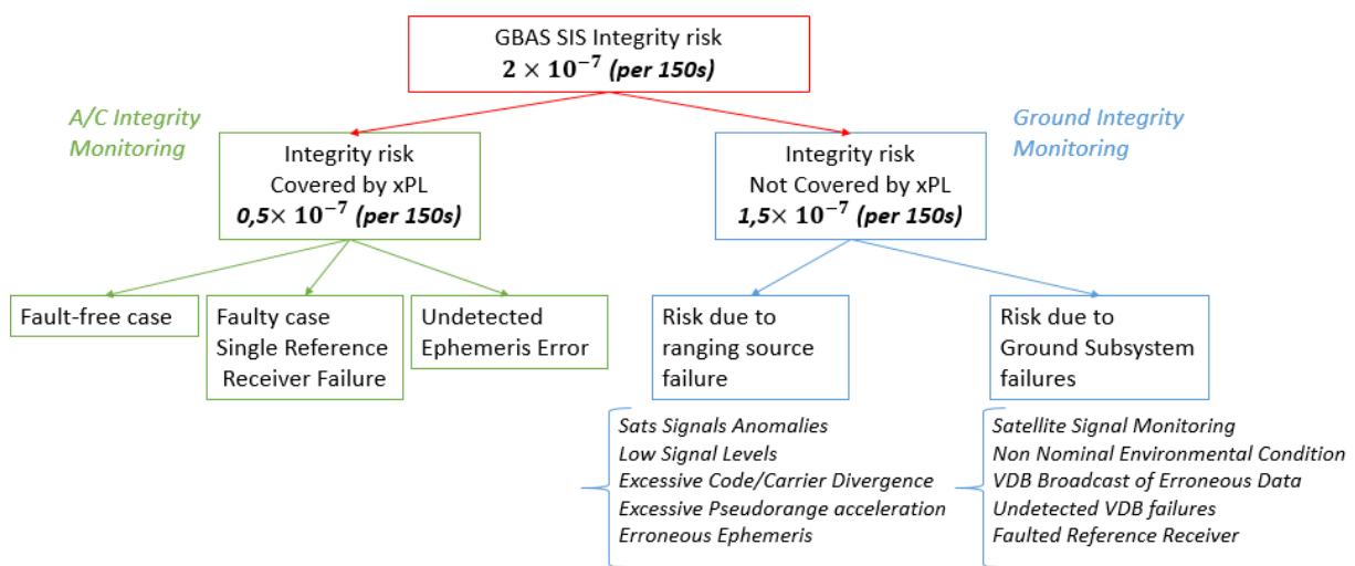
Figure 32-GBAS Integrity tree
