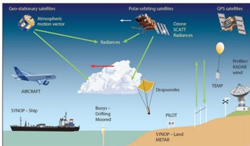
Figure 57-Sensors for NWM [119]
