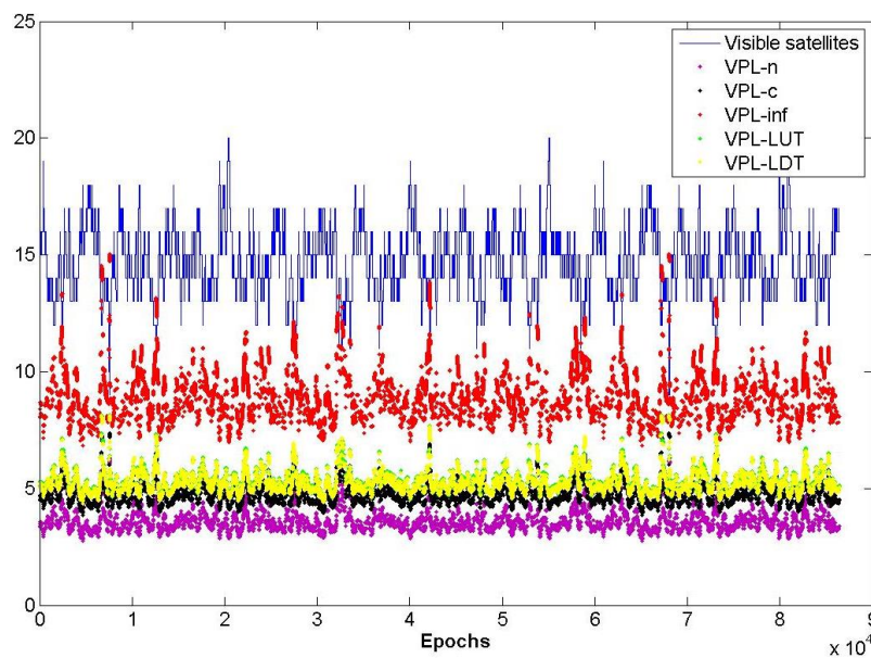
Figure 147-VPLs Seattle, D=10NM, Dth=5km, GPS (figure above) and GPS and GAL(figure below)
