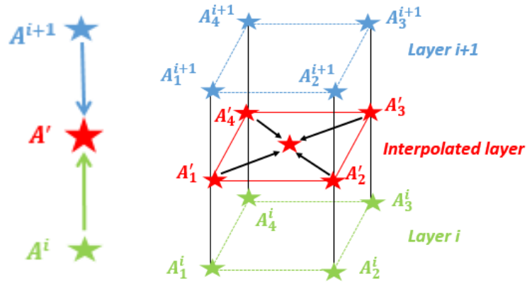
Figure 71-(a) -Vertical Interpolation - (b) Additional Horizontal Interpolation
