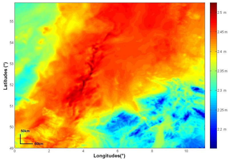
Figure 77-ZTD computed with Harmonie data
