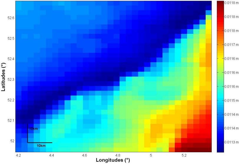
Figure 98-Difference between TC and ZTD for Schiphol
