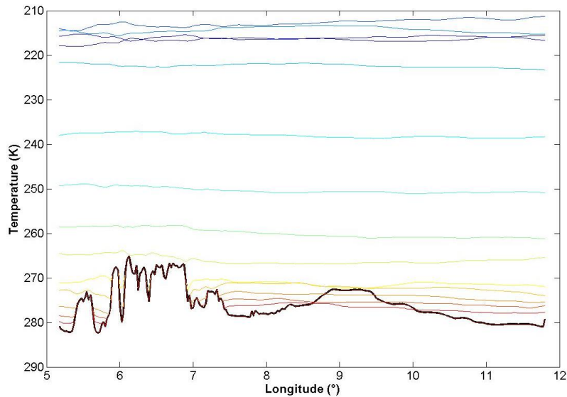
Figure 63-Temperature levels of NWM
