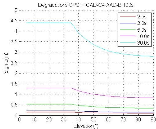
Figure 51-I-free Smoothed Error Degradation with Update Period
