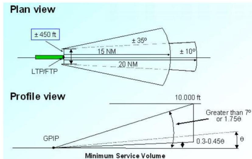
Figure 7-GBAS volume Coverage [1]
