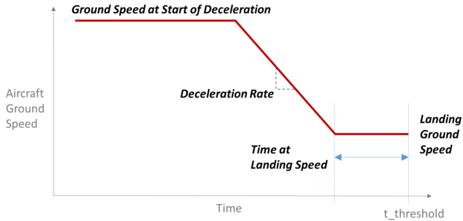
Figure 23-Velocity profile Model [88]
