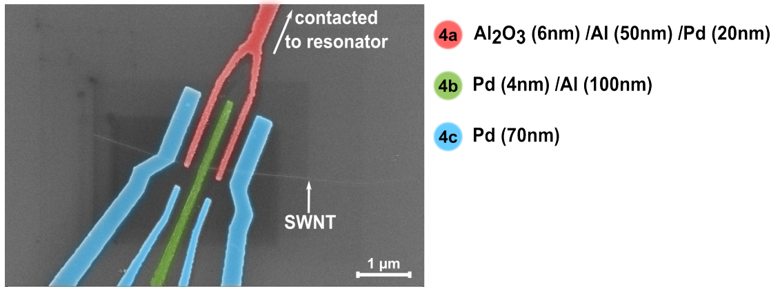
FIGURE 3.6: Device electrodes patterning steps for our final CPS design. The SEM picture is colorized with the same colour code as 3.1. The SWNT contrast is artificially enhanced. Three successive processes of lift-off positive electronic lithography are performed on the CNT, one for each material. The coupling fork-shape top gate (red) is fabricated first. Then the superconducting central electrode (green) is patterned. Finally normal outer contacts and side gates are made simultaneously.
