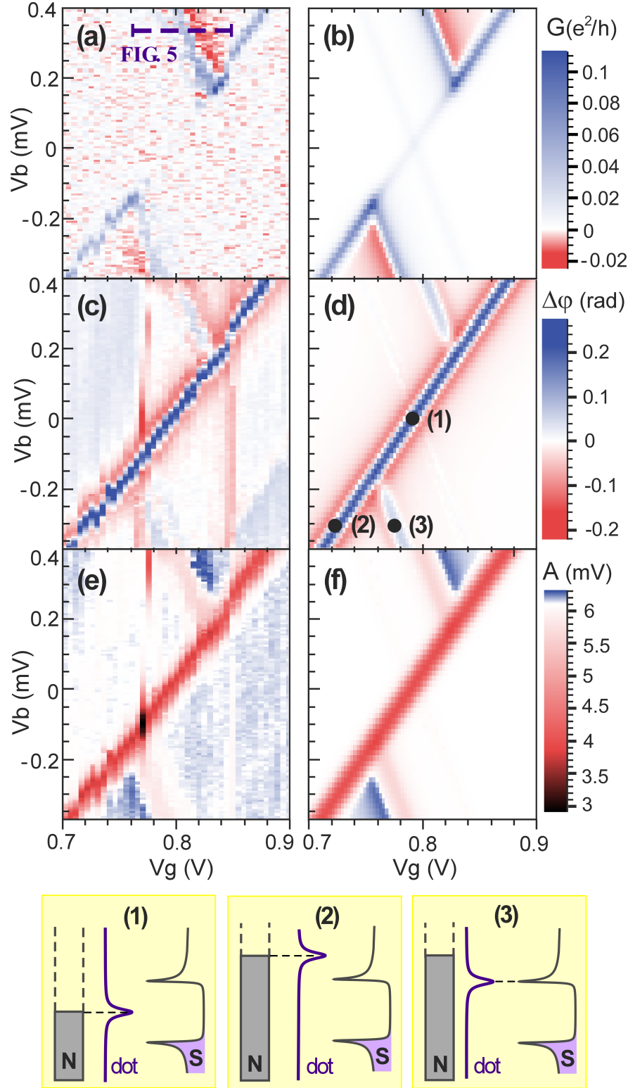
FIGURE 5.4: Panels (a), (c) and (e): Measured linear conductance G , phase shift \Delta\phi and total amplitude A of the transmitted microwave signal, versus the dot gate voltage V_g and the bias voltage V_b . Panels (b), (d) and (d): Predictions from equations E.2, 5.3 and E.12, for \Gamma_N/2\pi = 0.6 GHz, \Gamma_S/2\pi = 65 MHz, \Gamma_n/2\pi = 8 GHz, g/2\pi = 99 MHz, \Delta = 0.17 meV, T = 90 mK, \omega_0/2\pi = 6.65 GHz, A_0 = 6.1 mV, and \Lambda_0/2\pi = 0.259 MHz. The white colour corresponds to A = A_0 in panels (e) and (f). Panels (1), (2) and (3):
