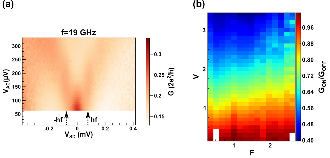
FIGURE 1: (a) Phenomenology of the finite-frequency response of the Kondo conductance vs bias voltage V_{SD} , as a function of the microwave excitation amplitude V_{AC} , at f=19 GHz. (b) Scaled Amplitude-frequency evolution of Kondo resonance. G_{ON}/G_{OFF} is the ratio between the Kondo conductances at zero-bias, with and without microwave excitation. The axis are the scaled amplitude V = eV_{AC}/k_B T_K and scaled frequency F = hf/k_B T_K .
