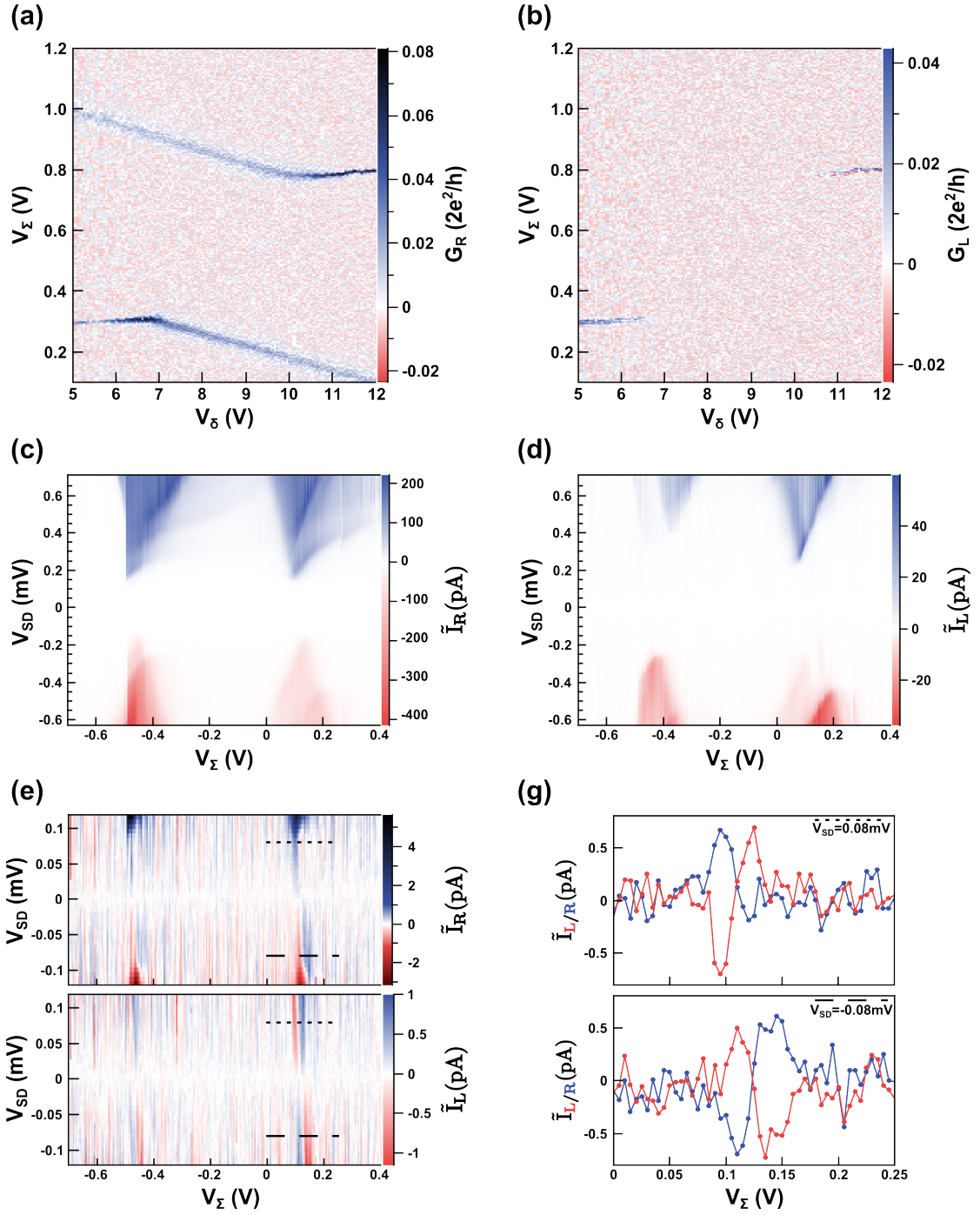
FIGURE 6.2: Device transport measurements. (a) and (b) are colour plots of the right and left differential conductance in the rotated gate-gate plane V_\Sigma - V_\delta for V_{SD} = -0.16 mV. To make comparison easier, colours for G_R and G_L are the same on the common range. (c) and (d) show the right and left currents dependence versus bias voltage V_{SD} and V_\Sigma . \tilde{I} refers to the current calculated from the numerical integration of the measured conductance G . (e) show \tilde{I}_{L/R} colour plots zoomed onto the sub-gap area. To make comparison easier, colours for G_R and G_L are the same on the common range. The dashes indicate the linear cuts plotted in (g).
