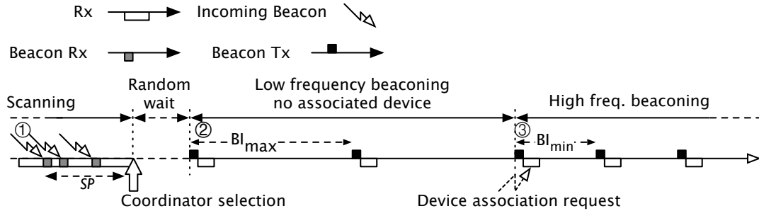
Figure 6.11: Principle of BFT: a node first scans for beacons from neighbors (1) and then chooses a coordinator. It then sends beacons to enable other nodes to join the network: at first, it sends beacons at a small rate (2) and switches to a higher rate if it becomes a coordinator for at least one node (3).
