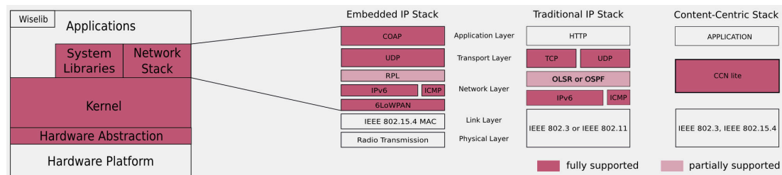
Figure 4.2: RIOT architecture
