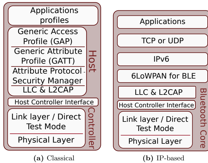
Figure 2.15: BLE Stacks
