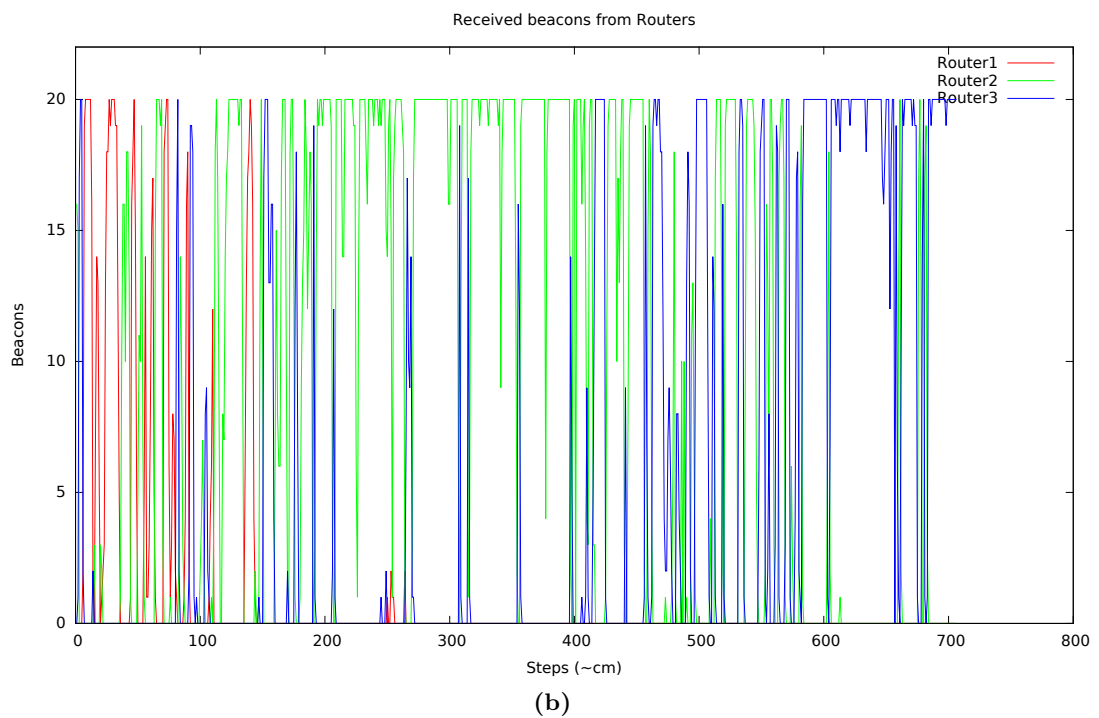
Figure 6.6: Beacons received from 3 synchronized coordinators. Each color represents a coordinator. In most positions, a large fraction of the beacons are successfully received, even though they all collide with each other at similar power.
