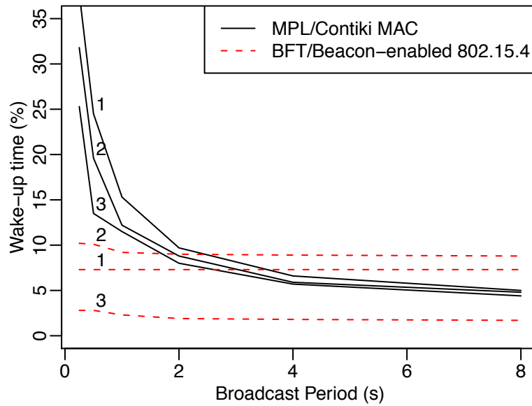
Figure 6.15: Proportion of time the radio is up for a chain of 3 sensors.
