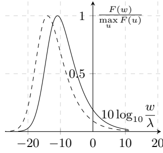
Figure 2.3: F(w)/\max_u F(u) vs. w/\lambda (dB) for the single-cluster channel model and different (\lambda, \gamma, \sigma_r) configurations. Solid curve: (2, 2, \frac{1}{2}), (2, 2, \frac{1}{4}) . Dashed curve: (4, 2, \frac{1}{2}), (2, 4, \frac{1}{2}) . 1/\lambda and \gamma are expressed in nanoseconds. F(w) is positive, showing that eq. (2.10) is verified.
