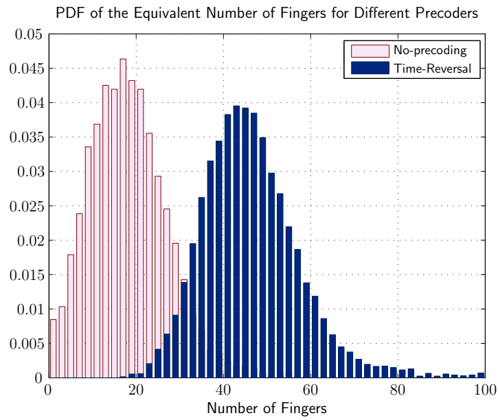
Figure 5.7: Estimation of the PDF of that number of fingers such that different precoders have same performance (see also Fig. 5.6). The histogram on the left (with the lighter background) refers to Optimum Prefilter (All-Rake) and No-prefiltering; the histogram on the right (with the darker background) refers to Optimum Prefilter (All-Rake) and time reversal.
