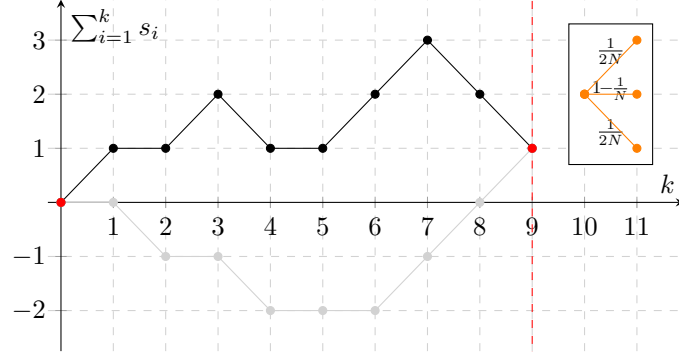
Figure 6.2: Two simple lattice walks are shown. In the two cases, K = 10 , and therefore the walk length is 9, and steps are \mathcal{S} = \{-1, 0, 1\} , as shown in the box at the north-east corner. Both walks start from (0, 0) and end at (9, 1) : the darker corresponds to the sequence (1, 0, 1, -1, 0, 1, 1, -1, -1) , while the lighter corresponds to (0, -1, 0, -1, 0, 0, 1, 1, 1) .
