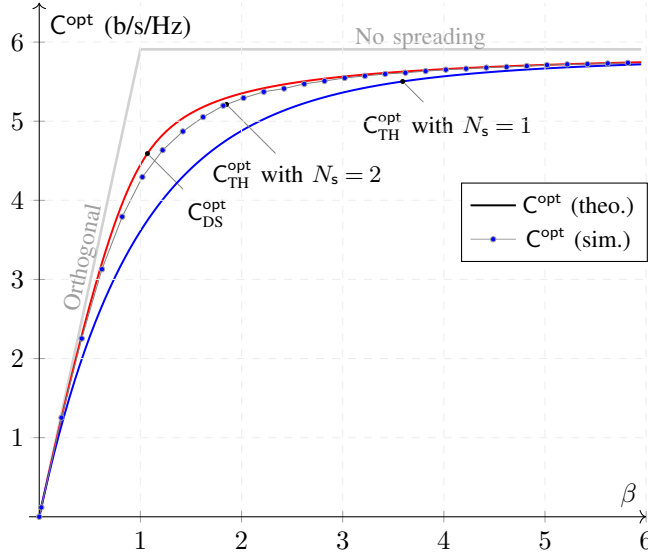
Figure 1.5: Spectral efficiency C^{\text{opt}} (b/s/Hz) as a function of \beta , for \mathcal{E}_b/N_0 = 10 dB. DS and TH with N_s = 1 are shown in solid lines, indicating that curves derive from closed form expressions, while values for TH with N_s = 2 are shown in dots, indicating that they derive from simulations. Orthogonal access is also reported for reference (gray solid line).
