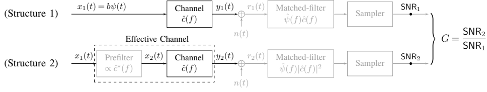
Figure 2.1: The two reference system models. Structure 1 corresponds to a traditional transmission with no prefiltering at the transmitter and matched-filtering at the receiver. Structure 2 corresponds to prefiltering at the transmitter with transmit matched-filter, and matched-filtering at the receiver. In both structures, \psi(t) is a zero-excess bandwidth waveform. It is assumed that prefiltering does not alter energy, that is, x_1(t) and x_2(t) have same energy \mathcal{E} .
