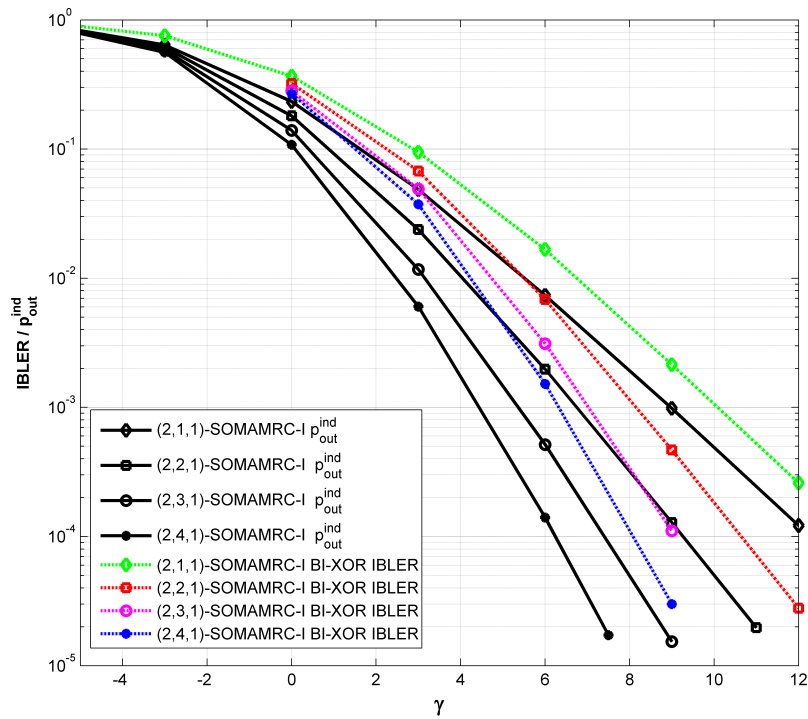
Figure 3.16: IBLER and p_{\text{out}}^{\text{ind}} , (2, L, 1)\text{-SOMAMRC-I} , where L = 1, 2, 3, 4 , R = 2/3 (b./c.u), \alpha = 2/3 and m_d = 2 .
