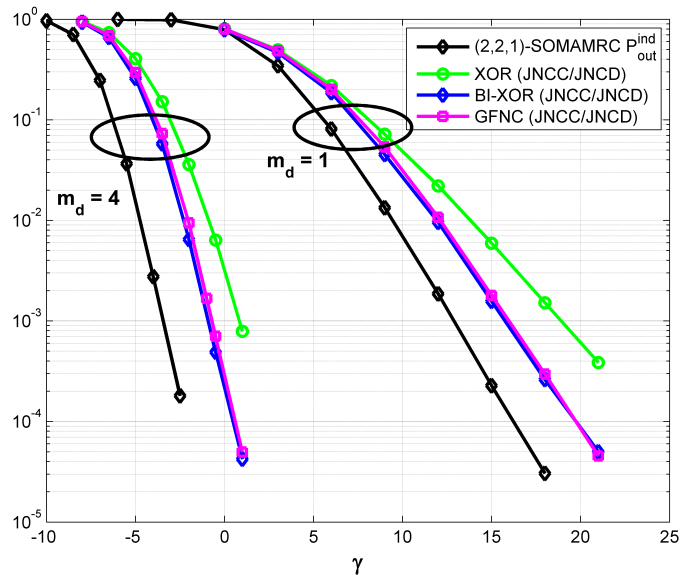
Figure 3.15: IBLER and p_{out}^{ind} , (2, 2, 1) -SOMAMRC-I, R = 2/3 (b./c.u), \alpha = 2/3 .
