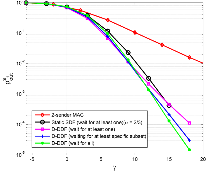
Figure 4.5: p_{out}^{ind} for an (2, 2, 1) -MAMRC, where m_d = m_r = 1 , \gamma_{r,d} = \gamma_{s,d} = \gamma , \gamma_{s,r} = 2\gamma , and R = 1(b.c.u) .
