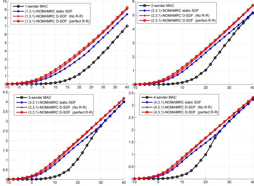
Figure 4.4: R_c^{ind}(\gamma) of waiting for all D-SDF vs static SDF in (M, 3, 1) -MAMRC, where M = 1, 2, 3, 4 , \gamma_{r,d} = \gamma_{s,r} = \gamma_{s,d} = \gamma .
