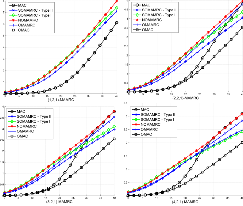
Figure 3.7: R_\epsilon^{ind}(\gamma) with M = 1, 2, 3, 4 , L = 2 , n = m_r = m_d = 1 .
