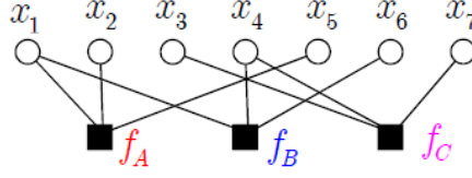
Figure 2.1: An FG for the product in example 1.
