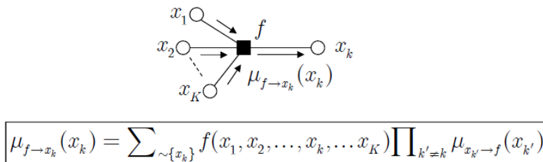
Figure 2.3: SPA update rule 2
