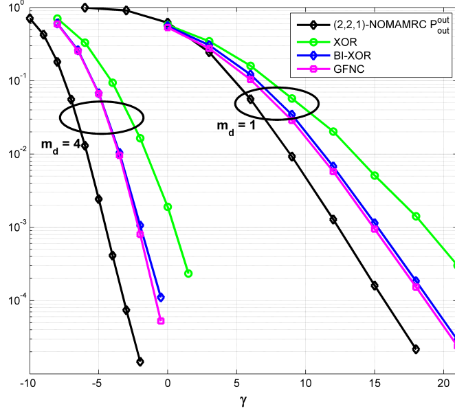
Figure 3.14: IBLER and p_{out}^{ind} , (2, 2, 1) -NOMAMRC, R = 2/3 (b./c.u), \alpha = 2/3 .
