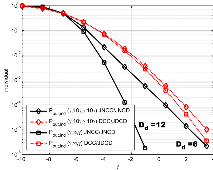
Figure 3.4: P_{out}^{ind} of JNCC/JNCD vs DCC/JDCD for (4, 2, 1)-OMAMRC, where m_d = 4 , m_r = 1 , R = 0.2 , and \alpha = 0.8 .
