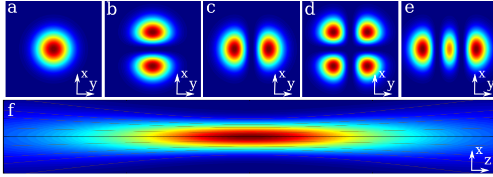
Figure 2.1.: (a) to (e) are transverse Hermitian mode intensities (from left to right TEM00, TEM10, TEM01, TEM11 and TEM02). f) is the intensity projection of a Gaussian beam in a plane containing the propagation axis.
