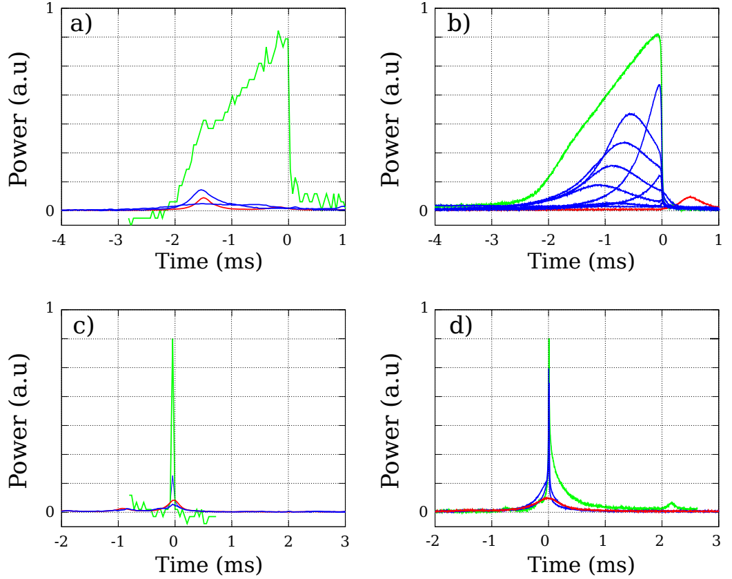
Figure 8.2.: Amplification and de-amplification for (a) and (c) the standard fiber and (b) and (d) the photonic fiber during the scan of the cavity. The scan is in the direction of self locking for (a) and (b), and in the direction of anti-self locking for (c) and (d). The green traces are the green peak, the red peaks are the red light with the pump blocked, and the blue peaks are the amplification and de-amplification of the red peak due to the pump when both frequencies are resonant.
