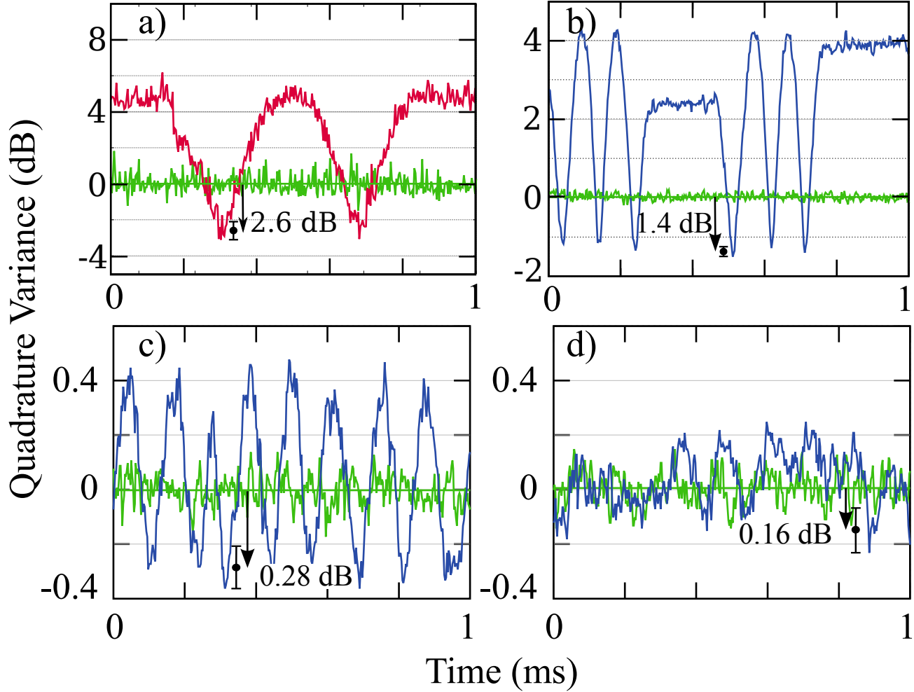
Figure 13.2.: Squeezing and anti-squeezing during scanning of the local oscillator phase at 1 Hz with a red calcite prism as an output coupler (a) and during the scanning at 3 Hz with a SF11 prism as an output coupler (b-d). (a) has been taken at sideband frequency of 5 MHz and (b) at 3 MHz with the same detector with 18 dB of shot-to-dark noise clearance and 50 MHz of bandwidth. (b) and (c) are taken respectively at 100 MHz and 150 MHz of sideband frequencies, with another detector with 4 dB of shot-to-dark noise clearance and 3 GHz of bandwidth.
