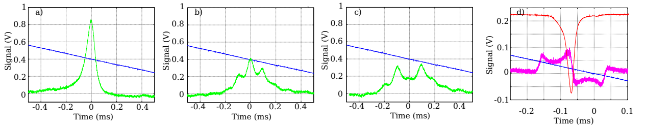
Figure 11.6.: (a-c) A few volts of modulation applied directly to the electrode during the scan of the resonator (with the voltage of this same electrode) with 532nm light (green). ((a) is the reference without modulation.) (d) Error signal obtained by modulating the voltage at the electrode at 249MHz and demodulating the reflected signal (magenta) during the scan of the frequency of the light of the laser at 1064nm (red).
