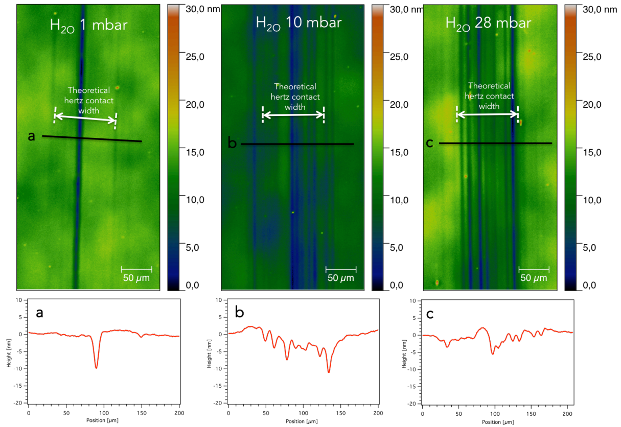
Figure 4.15 Scanning white-light interferometry measurements of the wear tracks obtained after friction test of a -C:H:Si:O against 52100 steel under (a) 1 mbar, (b) 10 mbar and (c) 28 mbar of water vapor n with the corresponding depth profile.
