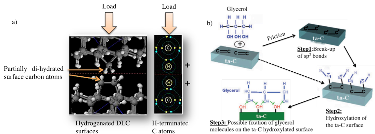
Figure 1.11. Proposed model for the passivation of carbon dangling bonds by hydrogen for hydrogenated DLC coatings from Erdemir et al. 54 (a) and (b) model of passivation of carbon dangling bonds by –OH groups from ta -C films, from Matta et al. 69 )
