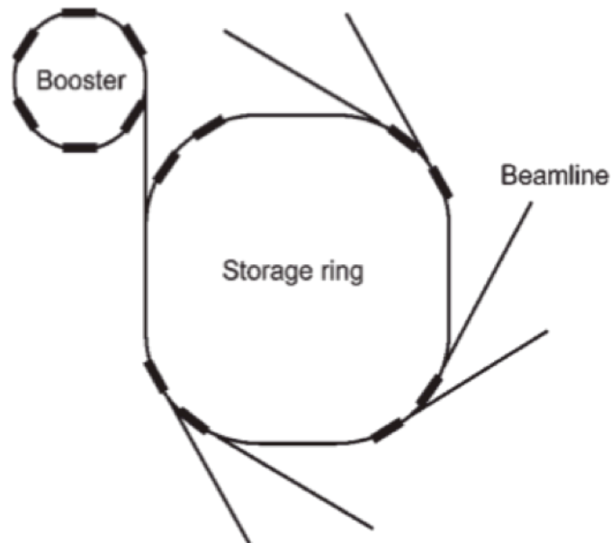
Figure 2.16. Description of synchrotron facility from reference 154
