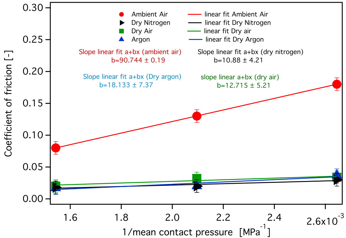
Figure 3.2. Evolution of the coefficient of friction as a function of the inverse of the mean theoretical Hertzian pressure for a -C:H:Si:O under different environmental conditions, and corresponding linear fits.
