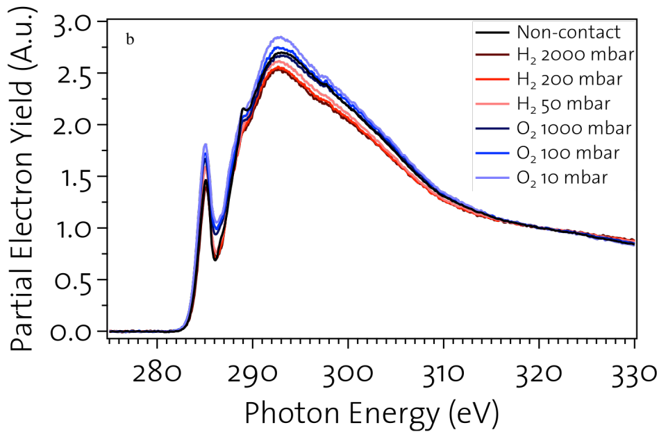
Figure 4.22. NEXAFS partial electron yield image of a-C:H:Si:O after tribological experiments under hydrogen (50, 200, 2000 mbar) and oxygen (10, 100, 1000 mbar) gas pressure. (a) The image is the sum of the images acquired at photon energies between 282 and 330 eV. Brighter colors correspond to higher intensity; (b) NEXAFS spectra extracted from region of interests (i.e. inside and outside the wear tracks)
