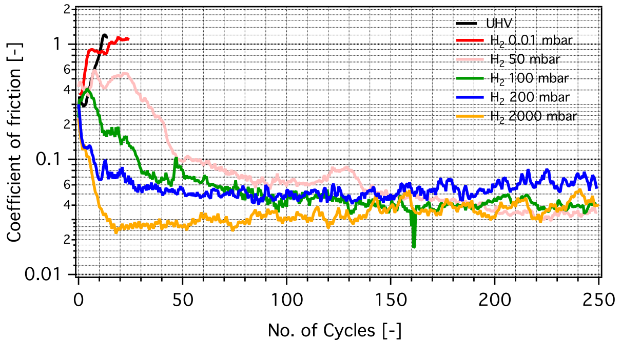
Figure 4.2. Evolution of the coefficient of friction vs. sliding cycles during tribological tests performed on a-C:H:Si:O sliding against 52100 steel pin under various hydrogen pressures (from high vacuum to 2000 mbar)
