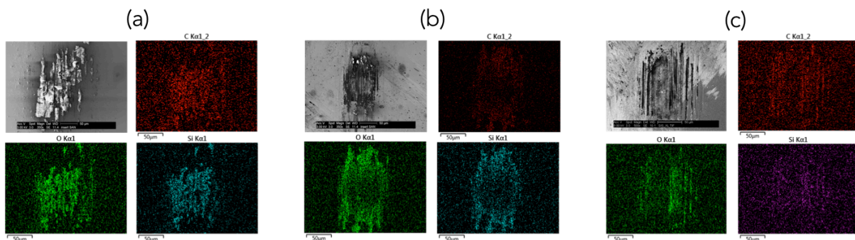
Figure 4.11. EDX analysis of the tribofilm formed on the steel counterbody upon sliding against a-C:H:Si:O at (a) 50 mbar of hydrogen, (b) 10 mbar of oxygen and (c) 1 mbar of water vapor
