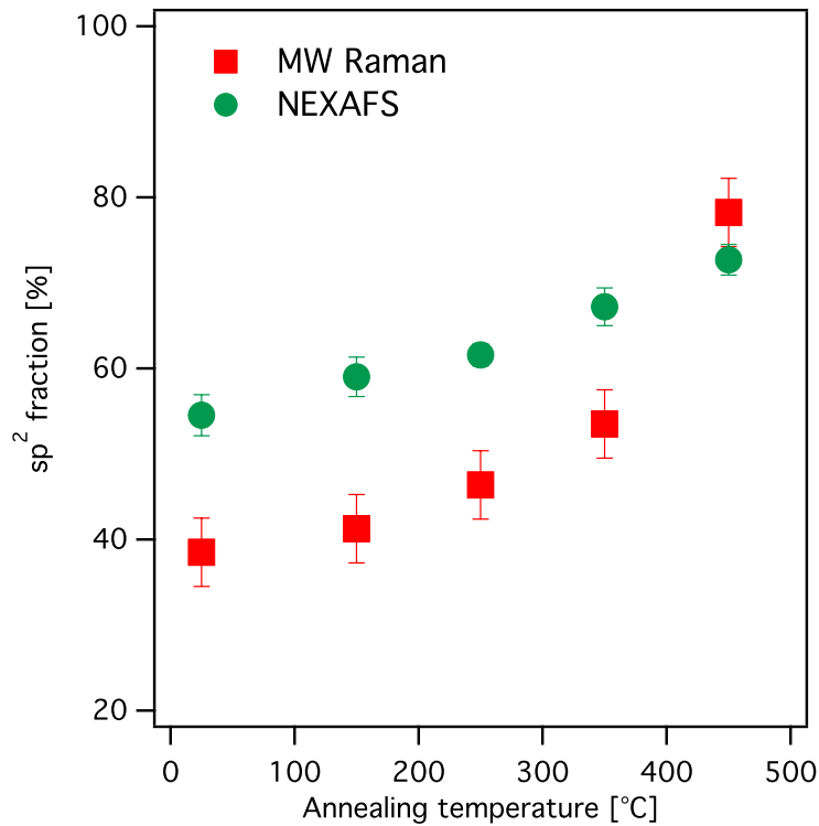
Figure 5.1. sp^2 -bonded carbon fraction in a\text{-C:H:Si:O} upon UHV annealing measured by MW Raman (red) and NEXAFS (green)
