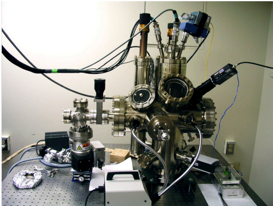
Figure 2.8. RHK 350 Scanning probe microscope from Carpick Research Group carpick.seas.epenn.edu
