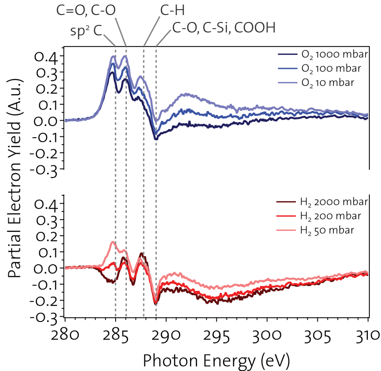
Figure 4.23. Difference in the NEXAFS partial electron yield spectra between worn and unworn regions of a -C:H:Si:O Red series curves: difference between a spectrum taken from the wear track generated upon sliding in hydrogen (50, 200 and 2000 mbar) and the spectrum from unworn a -C:H:Si:O; Blue series curves: difference between a spectrum taken from the wear track generated upon sliding in oxygen (10, 100 and 1000 mbar) and the spectrum from unworn a -C:H:Si:O.
