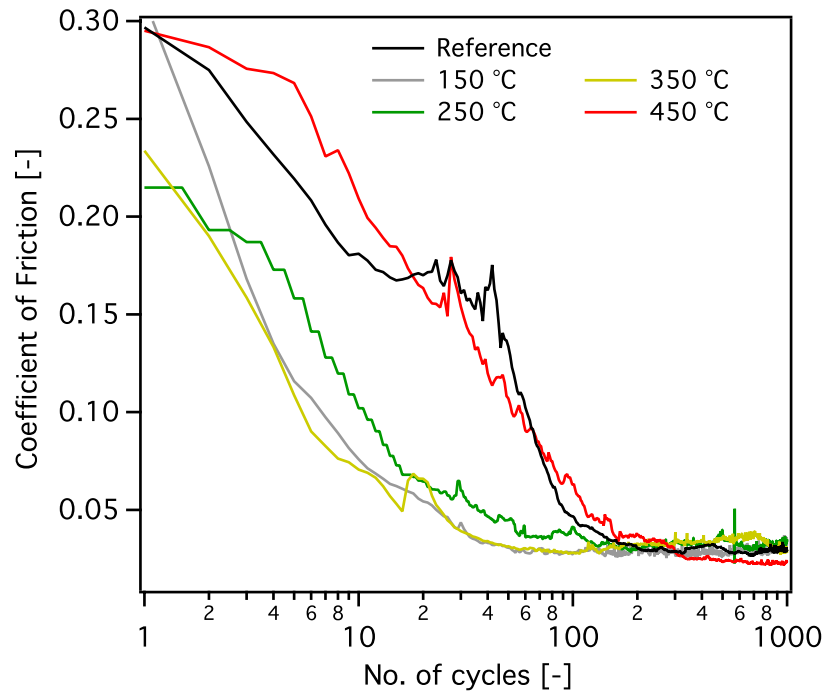
Figure 5.2. Evolution of coefficient of friction vs. cycles of annealed a -C:H:Si:O sliding against 52100 steel under dry nitrogen flow
