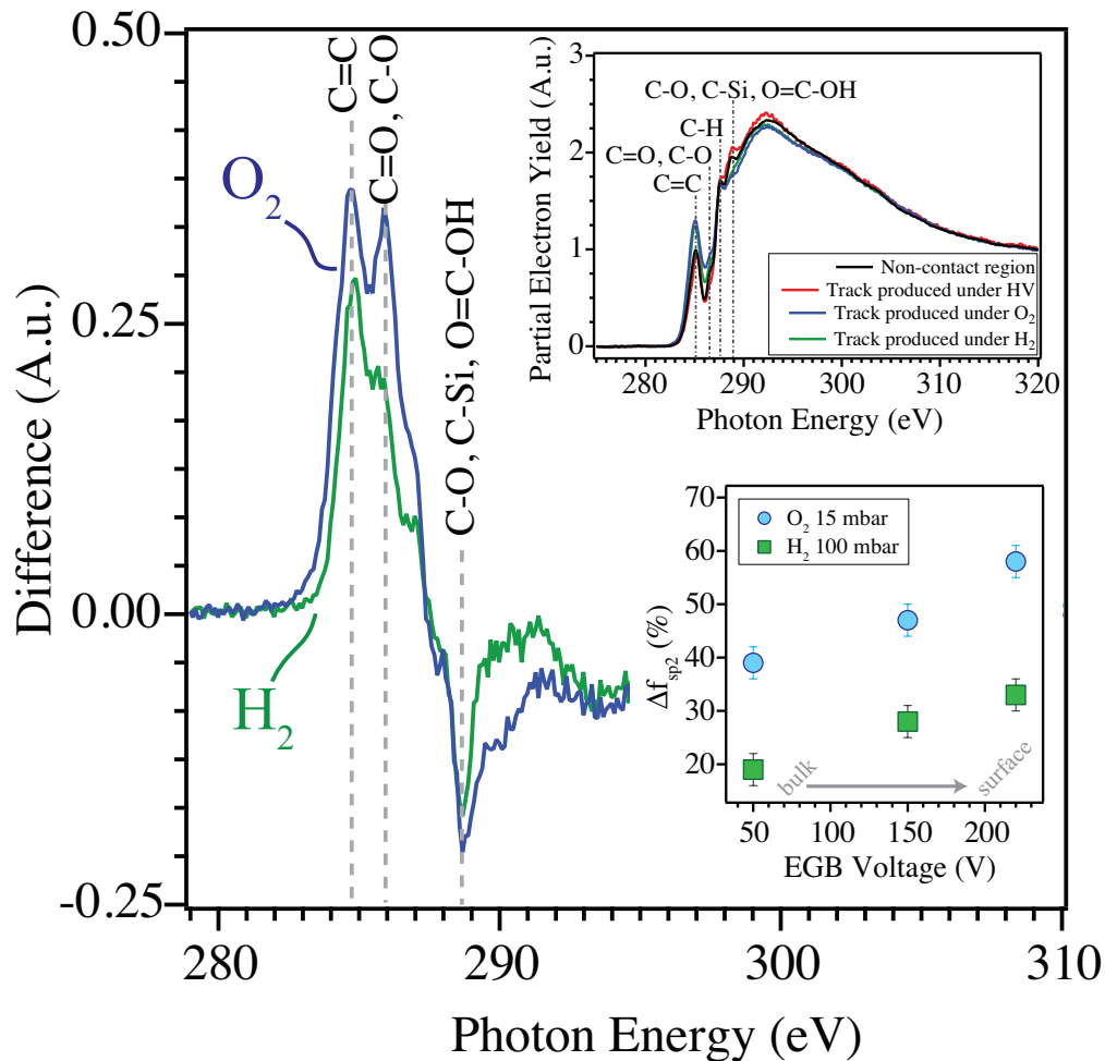
Figure 4.21. Difference in the NEXAFS partial electron yield spectra between worn and unworn regions of a -C:H:Si:O. Green curve: difference between a spectrum taken from the wear track generated upon sliding in hydrogen (100 mbar) and a spectrum from unworn a -C:H:Si:O; Blue curve: difference between a spectrum taken from the wear track generated upon sliding in oxygen (15 mbar) and a spectrum from unworn a -C:H:Si:O. The upper inset recall figure 15 (b) for comparison. The lower inset shows the relative variation of the fraction of sp^2 -bonded carbon for the track generated in hydrogen (100 mbar) or oxygen (15 mbar) as a function of the entrance grid bias (EGB) voltage (the surface sensitivity increases with the EGB voltage).
