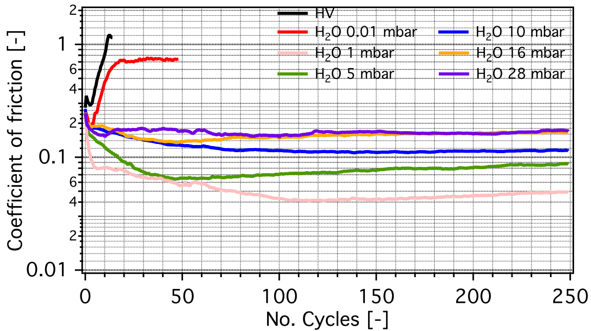
Figure 4.4. Evolution of the coefficient of friction vs. sliding cycles during tribological tests performed on a-C:H:Si:O sliding against 52100 steel pin under various environmental conditions (from high vacuum to 28 mbar of water vapor)
