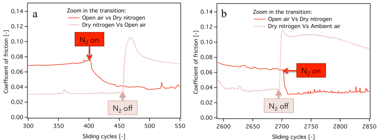
Figure 3.13. Detailed evolution of coefficient of friction for a\text{-C:H:Si:O} sliding against 52100 steel under a dynamic nitrogen flow (from Figure 12), (a) transition between high and low friction regimes for friction test started in ambient air (red) and dry nitrogen (pink) early in test. (b) transition at the end of the experiments.
