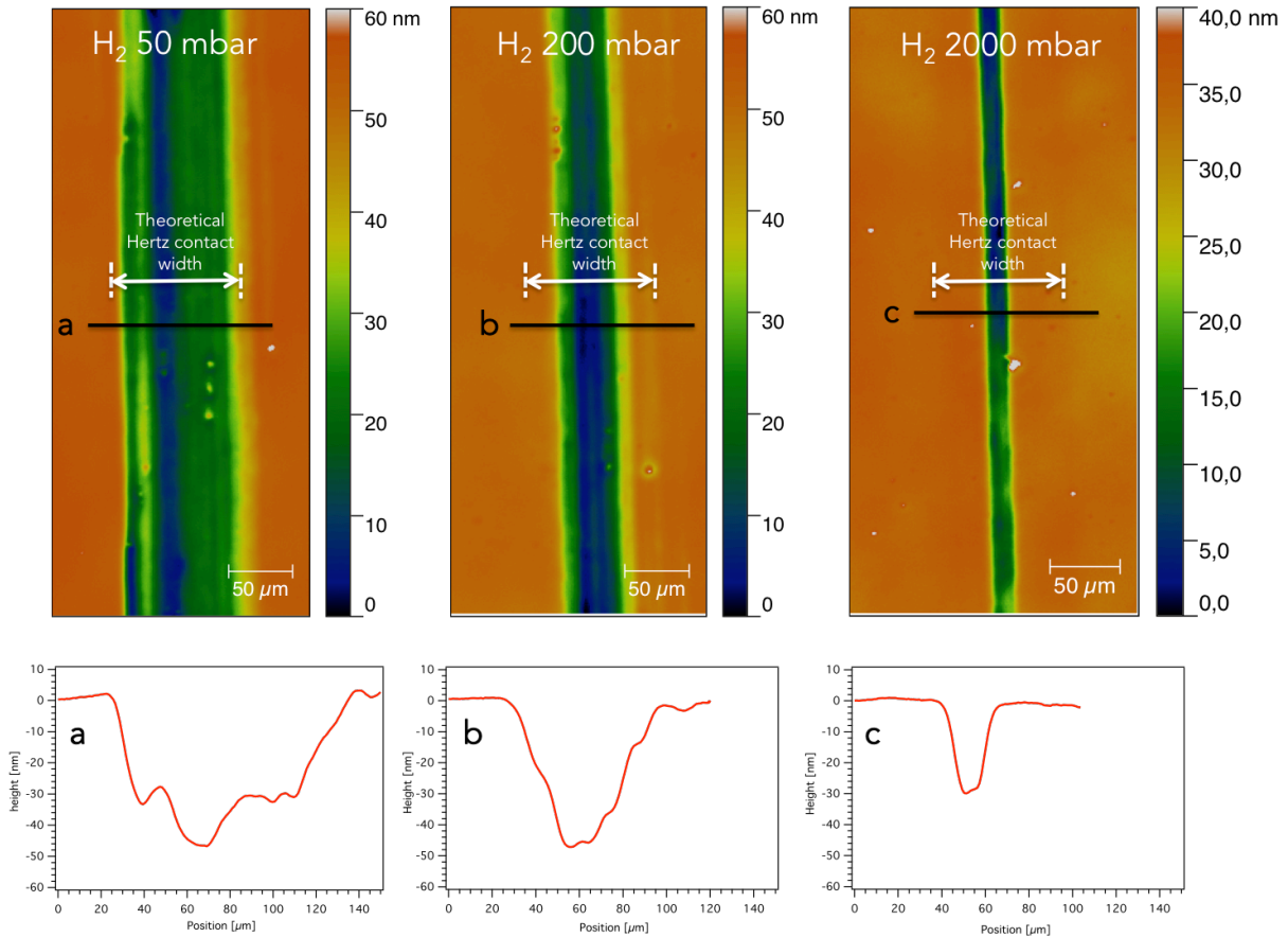
Figure 4.13. Scanning white-light interferometry measurements of the wear tracks obtained after friction test of a-C:H:Si:O against 52100 steel under (a) 50 mbar, (b) 200 mbar, (c) 2000 mbar of hydrogen with the corresponding depth profile.
