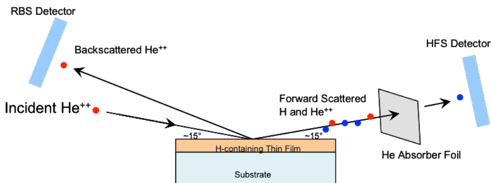
Figure 2.14. Scanning geometry of an HFS experiment
