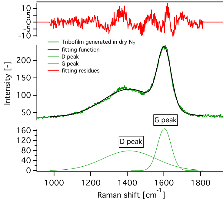
Figure 3.6. Gaussian fit of a Raman spectrum acquired at 325 nm on a tribofilm obtained after sliding a\text{-C:H:Si:O} against a 52100 steel ball under dry nitrogen flow.
