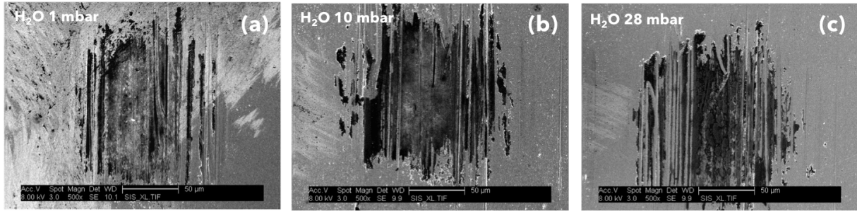
Figure 4.10. SEM analysis of the tribofilms formed on the steel counterbody upon sliding against a-C:H:Si:O under (a) 1 mbar, (b) 10 mbar and (c) 28 mbar of water vapor
