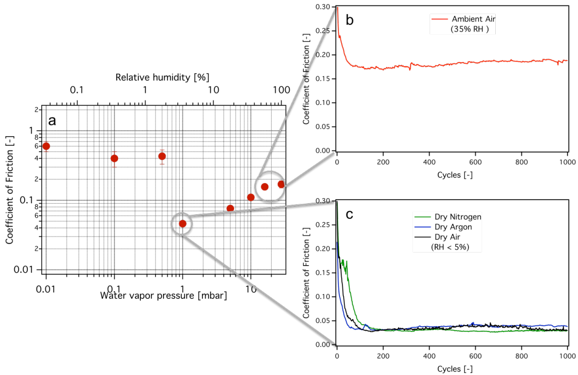
Figure 5.3. Correlation between the results obtained with the Environment Controlled Analytical Tribometer and the ambient air tribometer (CEAT) equipped with gas blowing system. Evolution of the coefficient of friction vs. sliding cycles with (a) various partial pressure of water vapor, (b) in ambient air (RH 35%), (c) under dry nitrogen, dry argon or dry air flow (RH<5%).
