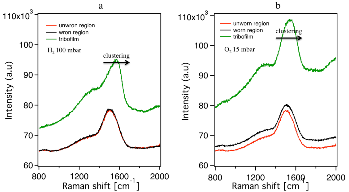
Figure 4.18. Visible Raman spectra acquired on worn and unworn regions of a -C:H:Si:O as well as on the tribofilm formed on 52100 steel pin after sliding at (a) 100 mbar of hydrogen and (b) 15 mbar of oxygen
