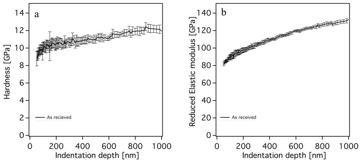
Figure A.3. (a) Hardness and (b) Elastic modulus of a-C:H:Si:O measured by nanoindentation
