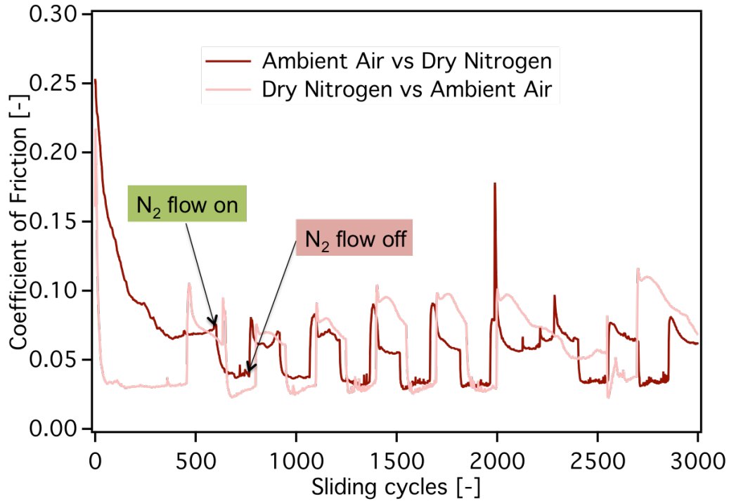
Figure 3.12. Evolution of the coefficient of friction for a\text{-C:H:Si:O} sliding against 52100 steel under dynamic flow of nitrogen gas, the experiments starting either in ambient air (red curve) or in dry nitrogen (pink curve).
