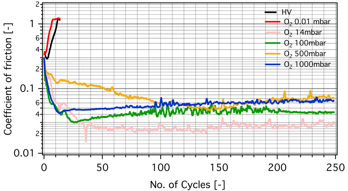
Figure 4.3. Evolution of the coefficient of friction vs. sliding cycles during tribological tests performed on a-C:H:Si:O sliding against 52100 steel pin under various environmental conditions (from high vacuum to 1000 mbar of oxygen)
