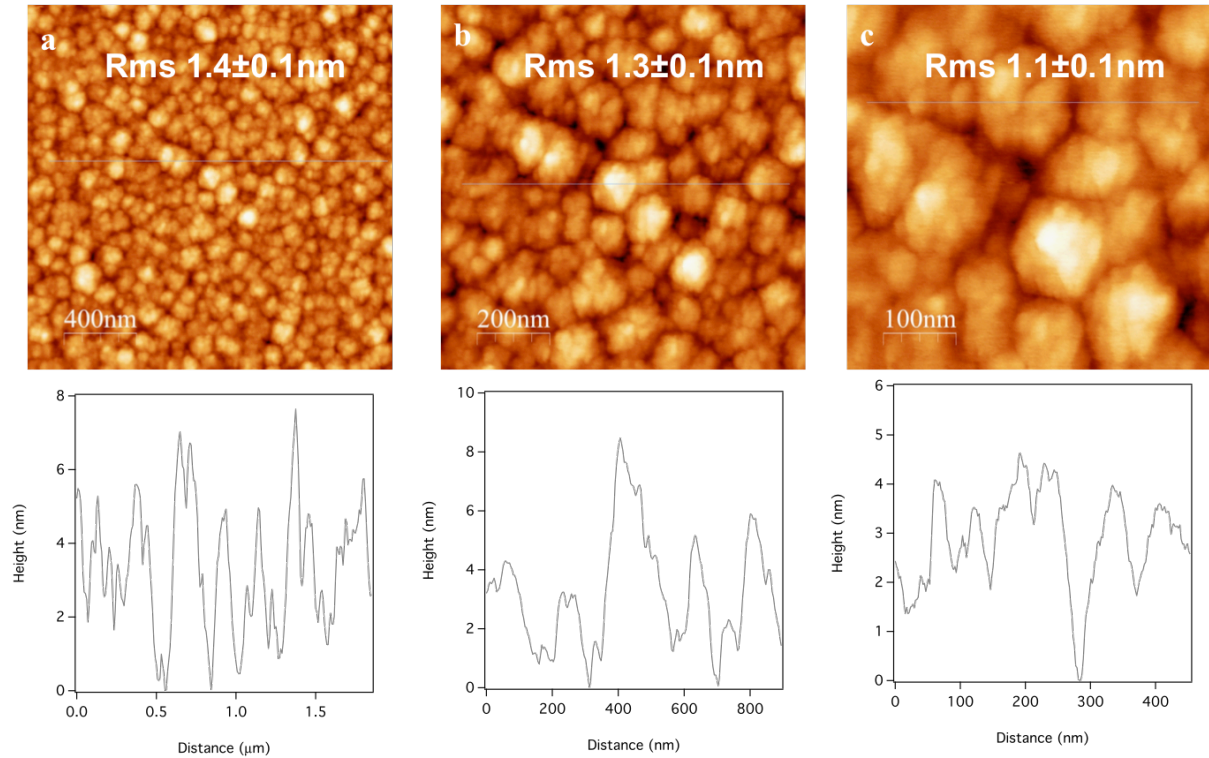
Figure A.2. rms roughness of a-C:H:Si:O measured by AFM an area of (a) 2 \times 2 \mu\text{m}^2 , (b) 1 \times 1 \mu\text{m}^2 and (c) 500 \times 500 \text{ nm}^2
