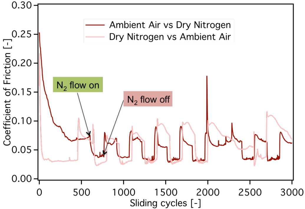
Figure 3.12. Evolution of the coefficient of friction for a\text{-C:H:Si:O} sliding against 52100 steel under dynamic flow of nitrogen gas, the experiments starting either in ambient air (red curve) or in dry nitrogen (pink curve).
