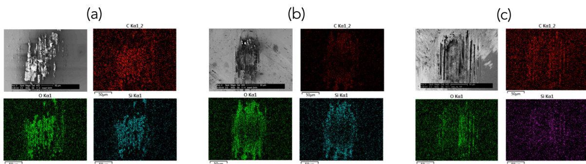
Figure 4.11. EDX analysis of the tribofilm formed on the steel counterbody upon sliding against a\text{-C:H:Si:O} at (a) 50 mbar of hydrogen, (b) 10 mbar of oxygen and (c) 1 mbar of water vapor
