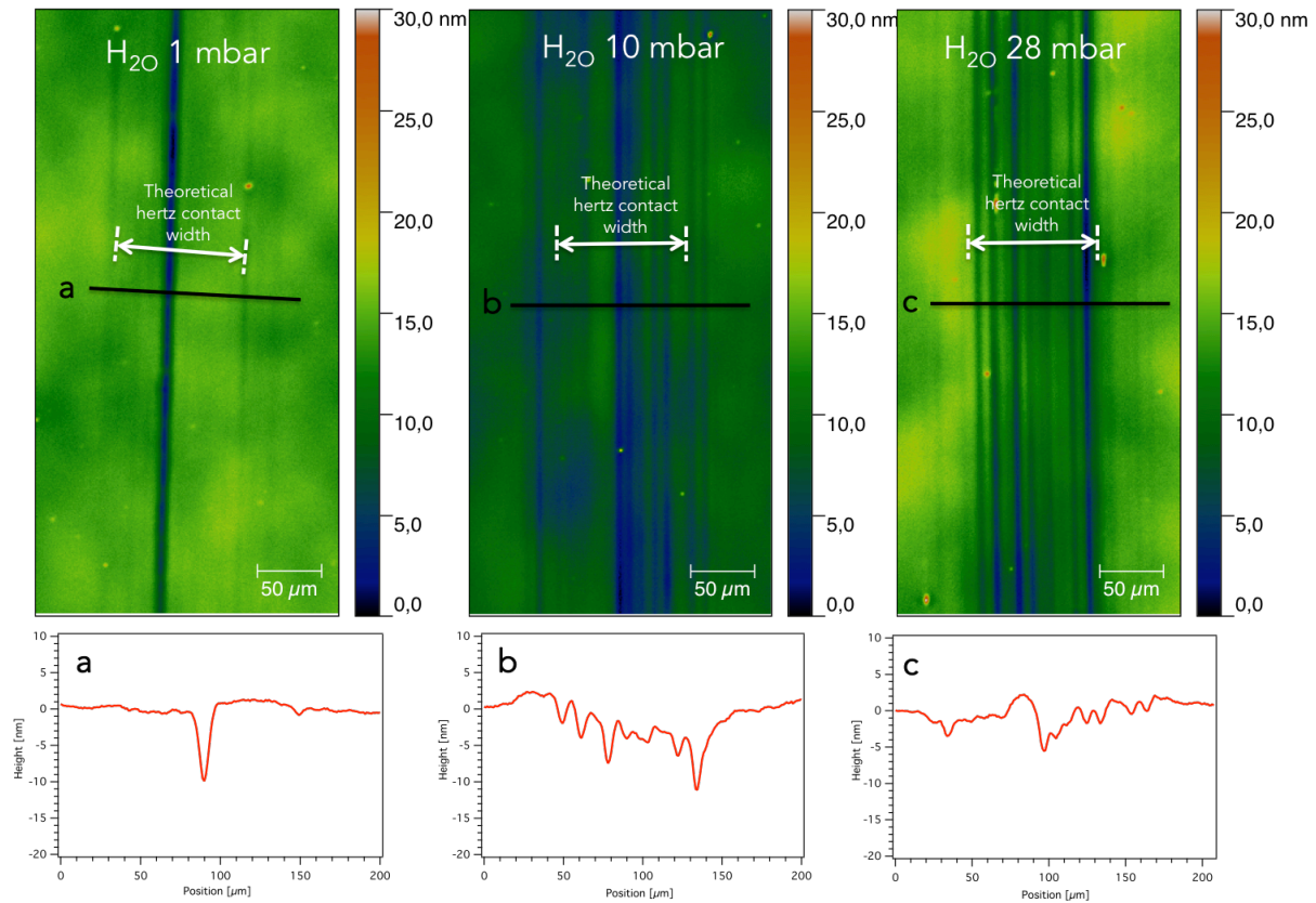
Figure 4.15 Scanning white-light interferometry measurements of the wear tracks obtained after friction test of a -C:H:Si:O against 52100 steel under (a) 1 mbar, (b) 10 mbar and (c) 28 mbar of water vapor n with the corresponding depth profile.
