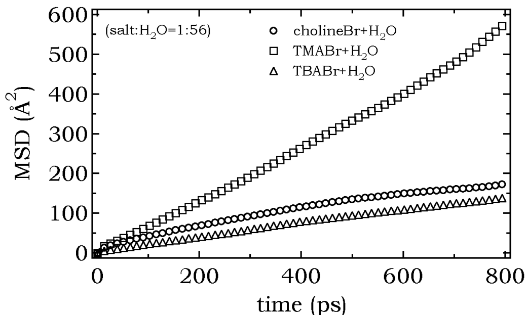
Figure 8.24: The MSD of average hydrogen atoms of TMA + , Choline + and TBA + cations are plotted as a function of time for aqueous solution with x_m=1:56 .
