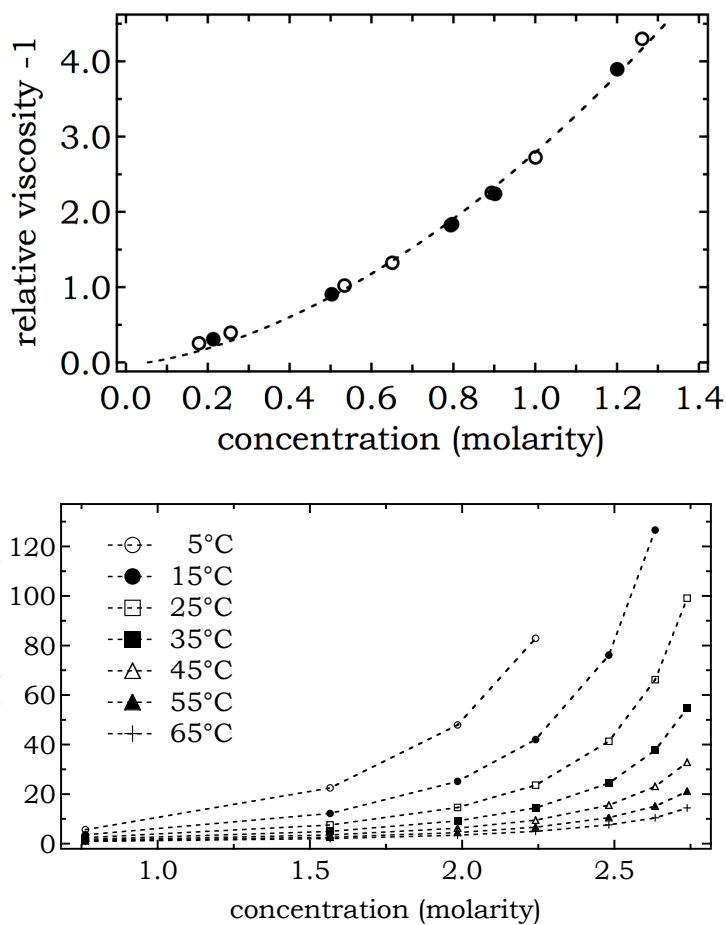
Figure 4.5: Viscosity of aqueous TBABr solution as a function of concentration and temperature [Kay 1966a] [Surdo 1979].
