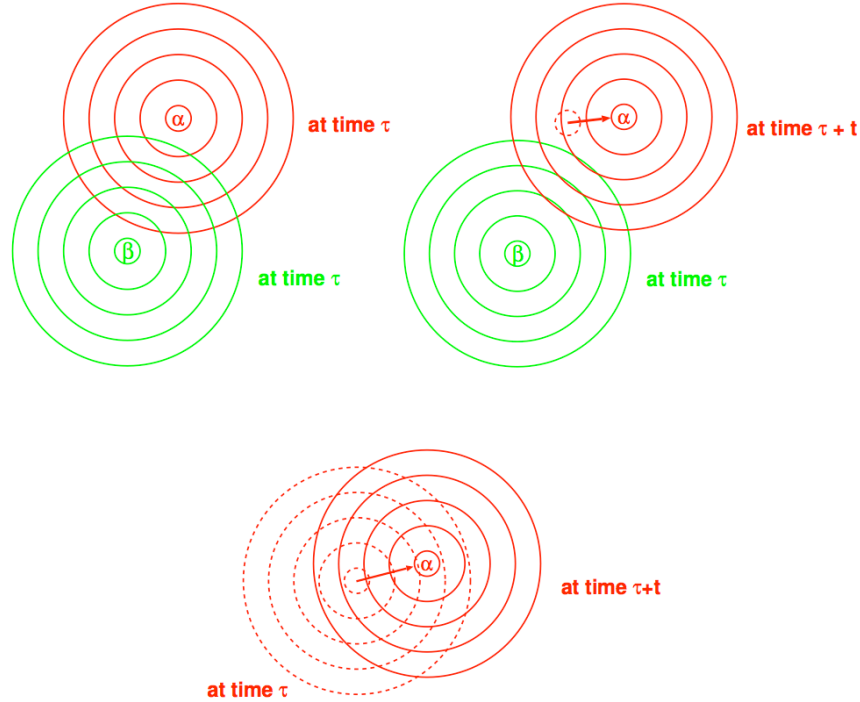
Figure 5.3: Origin of coherent and incoherent scattering.
