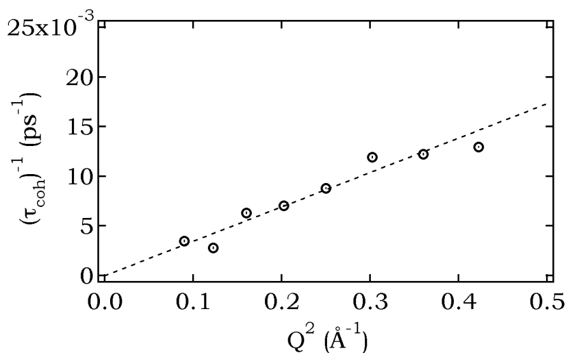
Figure 8.21: Inverse of translational relaxation time (extracted from simulated coherent I(Q,t) curves) are plotted as a function of Q^2 for aqueous TBABr solution with x_m=1:112 . The D_{tr} from a linear fit passing through origin (continuous diffusion).
