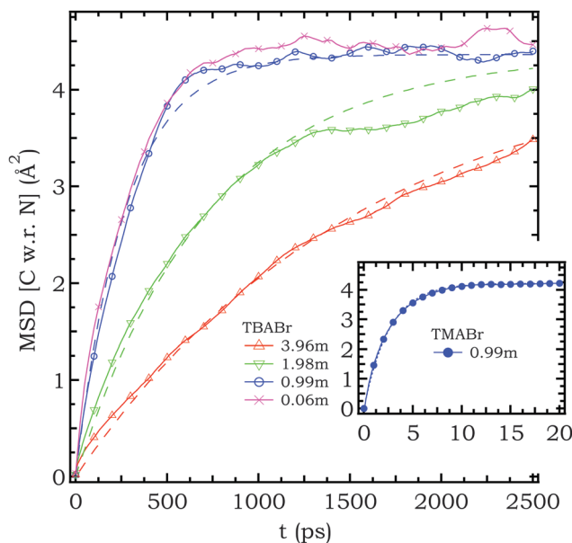
Fig. 5 Investigation of global cation rotation for \text{TBA}^+ and \text{TMA}^+ : mean square displacement (MSD) of \alpha C atoms with respect to the central N atom, versus time, for \text{TBA}^+ in selected TBABr solutions; inset features the same type of data for \text{TMA}^+ in 0.99 m TMABr solution. Dashed lines represent the fit of data with eqn (2).
