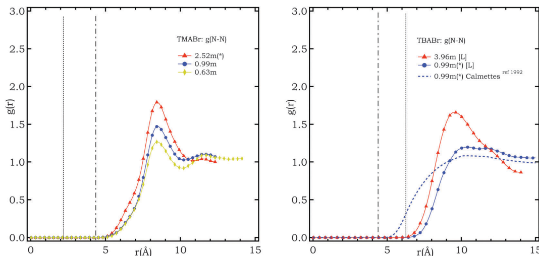
Fig. 3 Radial distribution function between the nitrogen atoms of cations, g_{NN} , for TMABr solutions (left) and TBABr solutions (right) for a series of concentrations as indicated. Symbol [L] indicates the use of large simulation boxes. Dotted and dashed-dotted vertical lines indicate, respectively, the position of the outermost hydrogen atoms of the cation and the position of the first peak in g_{NOW} . Dashed blue series in the right figure corresponds to data from a TBA–TBA potential derived from hypernetted chain (HNC) calculations in ref. 18.
