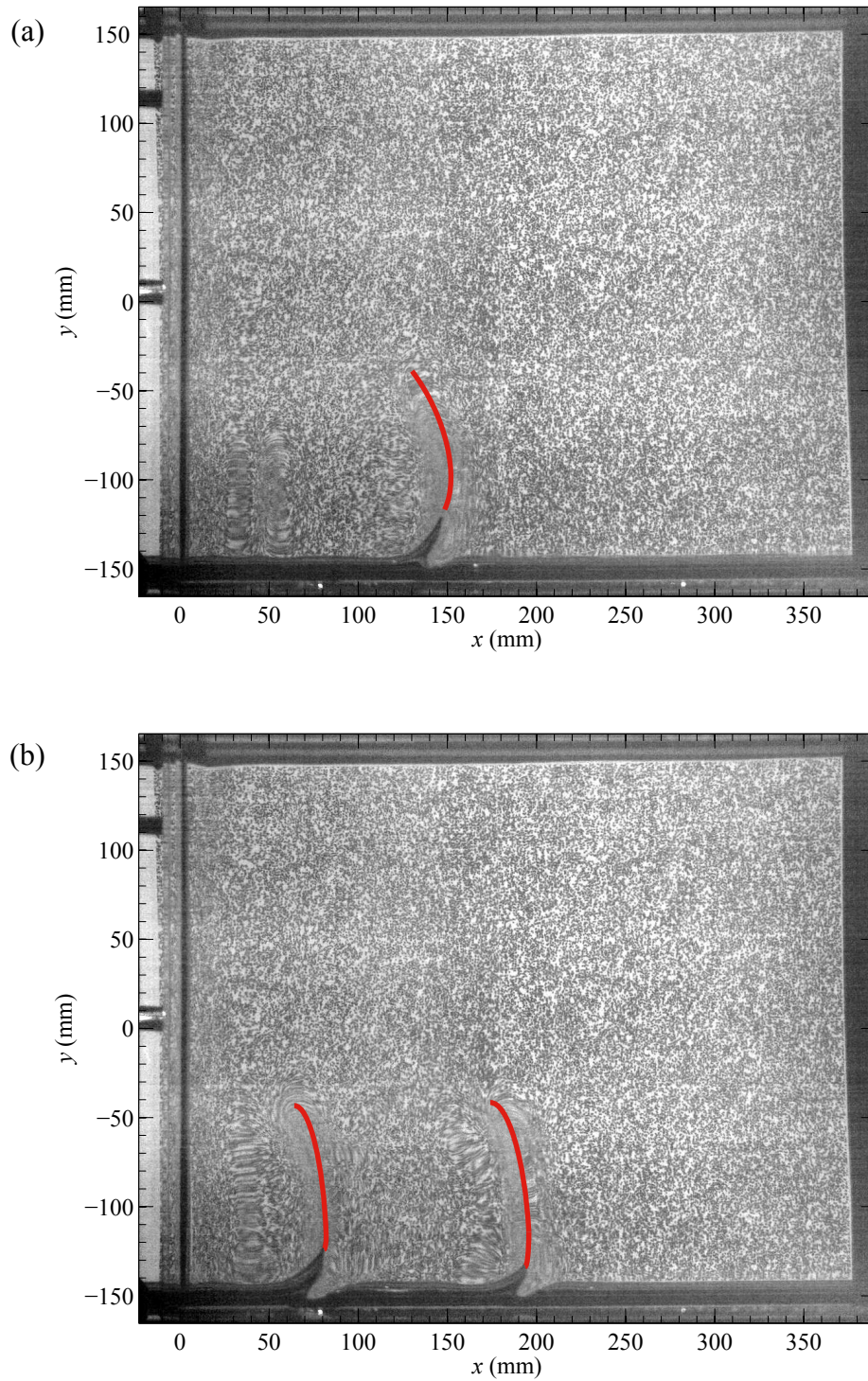
Figure 5.19: Dot patterns in presence of solitary waves for \nu = 562 \times 10^{-6} \text{ m}^2 \cdot \text{s}^{-1} , (a) at U_a = 10.9 \text{ m} \cdot \text{s}^{-1} , (b) at U_a = 11.2 \text{ m} \cdot \text{s}^{-1} . Red lines are added to ease the visualization of the solitary waves.
