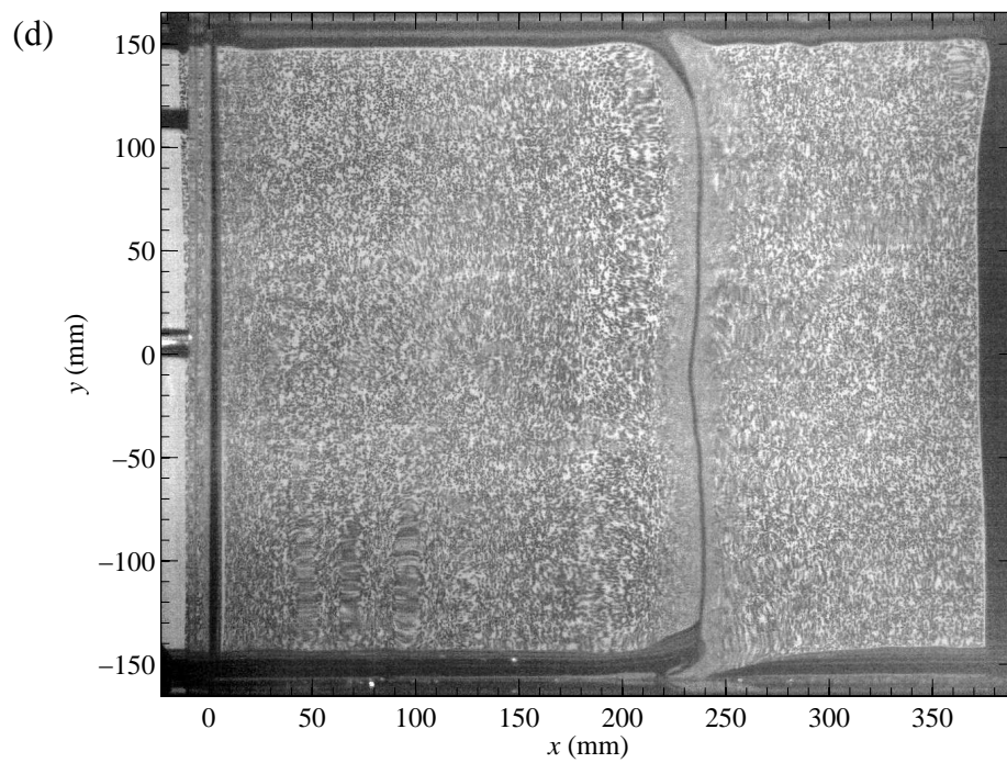
Figure 5.19 (continued). At U_a = 11.8 \text{ m}\cdot\text{s}^{-1} , (c) with multiple solitary waves, (d) with a fully transverse solitary wave.
