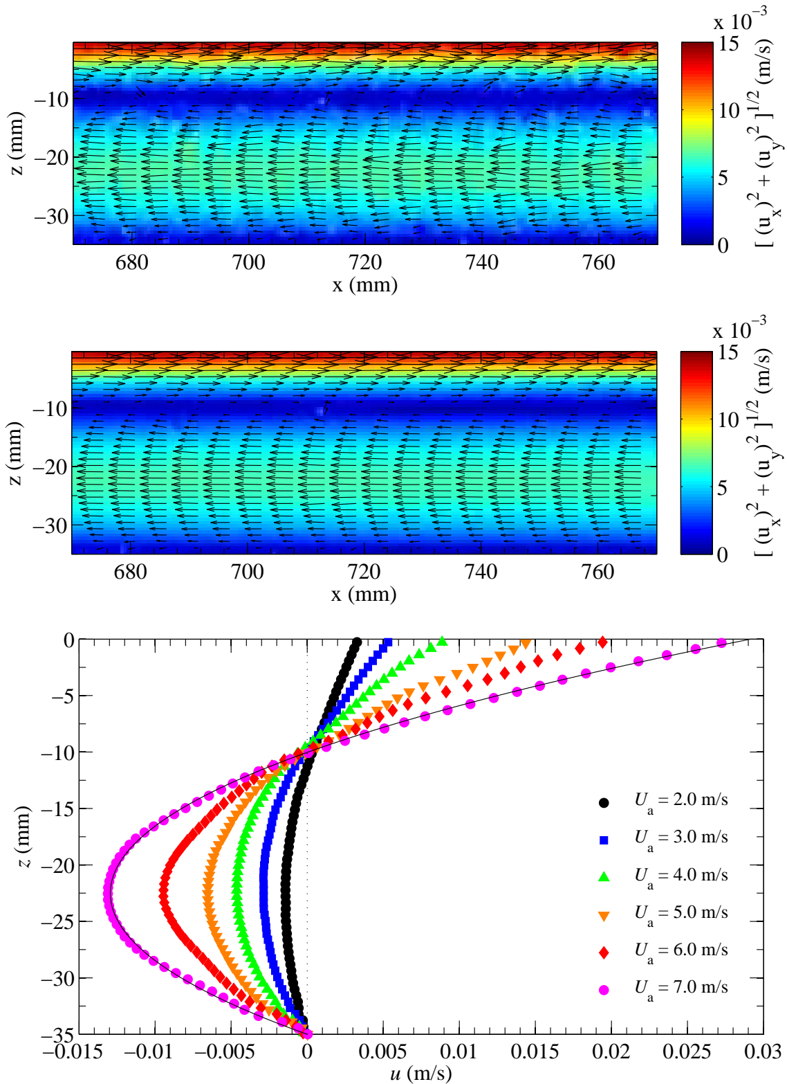
Figure 2.17: PIV measurements in the liquid at fetch x = 72 cm at the center of the tank. The wind is blowing left to right. (a) Instantaneous velocity field at U_a = 5.0 m.s -1 . (b) Temporally averaged velocity field at U_a = 5.0 m.s -1 . (c) Mean velocity profiles for various wind velocities U_a under 7 m.s -1 . The profiles are averaged in time and in the streamwise direction over \Delta x = 100 mm. The continuous line shows the quadratic profile (2.2.7) for U_a = 7.0 m.s -1 , with U_s fitted at 0.029 m.s -1 .
