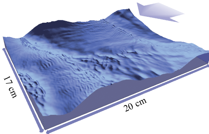
Figure 1.9: 3D rendering of the wave field at 6.4 \text{ m}\cdot\text{s}^{-1} . The arrow indicates the wind direction. Adapted from [Kiefhaber et al., 2014] .
