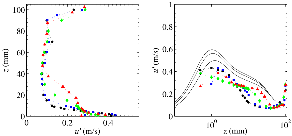
Figure 2.12: Root mean square of the velocity fluctuations at U_a = 3.9 \text{ m}\cdot\text{s}^{-1} at the center of the wind channel at fetch -100 \text{ mm} ( \bullet ), 20 \text{ mm} ( \blacksquare ), 500 \text{ mm} ( \blacklozenge ) and 1000 \text{ mm} ( \blacktriangle ). (Left) In linear coordinates. (Right) Compared in semilogarithmic coordinates with numerical simulations (continuous lines). Note that the axes are inverted between the two plots. The simulated profiles correspond from bottom to top to the increasing fetch x in table 2.2 on page 40.
