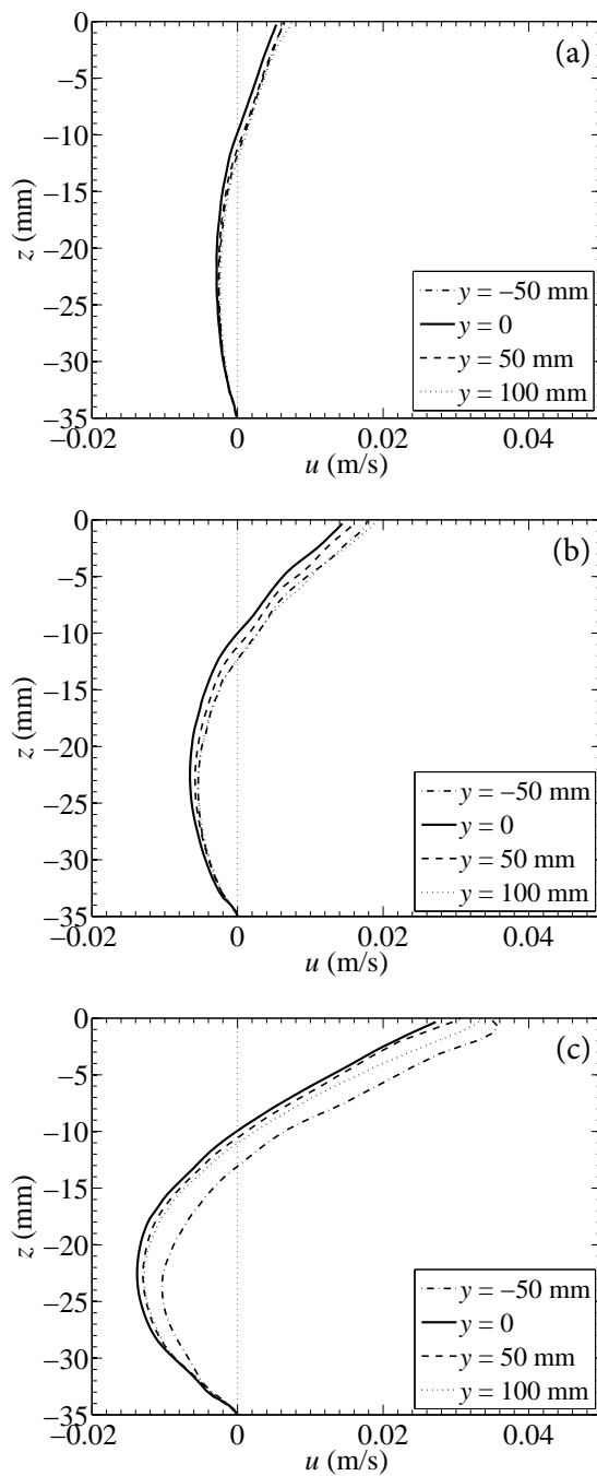
Figure 2.22: Mean velocity profiles obtained by PIV measurement in the liquid at fetch x = 72 cm at various y . The wind is blowing from left to right at wind velocity (a) U_a = 3.0 \text{ m.s}^{-1} ; (b) U_a = 5.0 \text{ m.s}^{-1} ; (c) U_a = 7.0 \text{ m.s}^{-1} .
