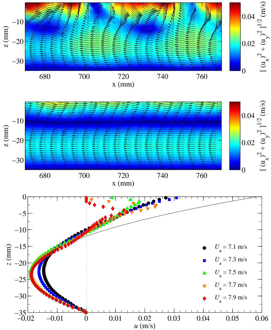
Figure 2.18: PIV measurements in the liquid at fetch x = 72 \text{ cm} at the center of the tank. The wind is blowing left to right. (a) Instantaneous velocity field at U_a = 7.5 \text{ m.s}^{-1} . (b) Temporally averaged velocity field at U_a = 7.5 \text{ m.s}^{-1} . (c) Mean velocity profiles for various wind velocities U_a over 7 \text{ m.s}^{-1} . The profiles are averaged in time and in the streamwise direction over \Delta x = 100 \text{ mm} . The continuous line shows the quadratic profile (2.2.7) fitted on the lower two third of the profile for U_a = 7.9 \text{ m.s}^{-1} .
